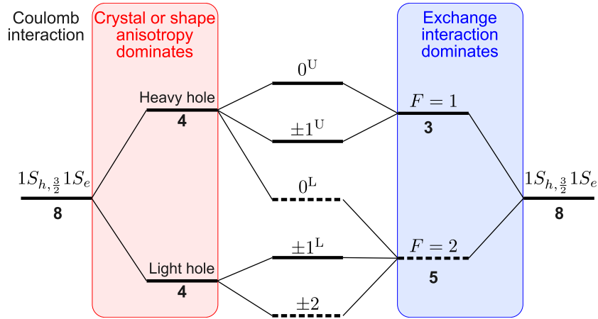
Figure 1.5: Energy diagram of the exciton fine structure of a semiconductor nanocrystal in the case of an oblate deformation. On the left, in red, the crystal or shape anisotropy split the sublevels. On the right in blue, the sublevels are split by the exchange interaction. Between these two limits, the energy levels are split into five sublevels, their order here corresponds to an oblate deformation. The dotted lines show the non-optically active states.
