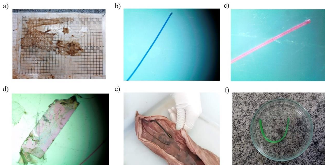
Figure 3. Macroplastics detected in the tuna and tuna-like species from the Southwestern Tropical Atlantic: a) plastic bag, b) blue filament, c) pink filament, d) plastic tape, e) nylon fishhook, and f) fragment of artificial bait.
