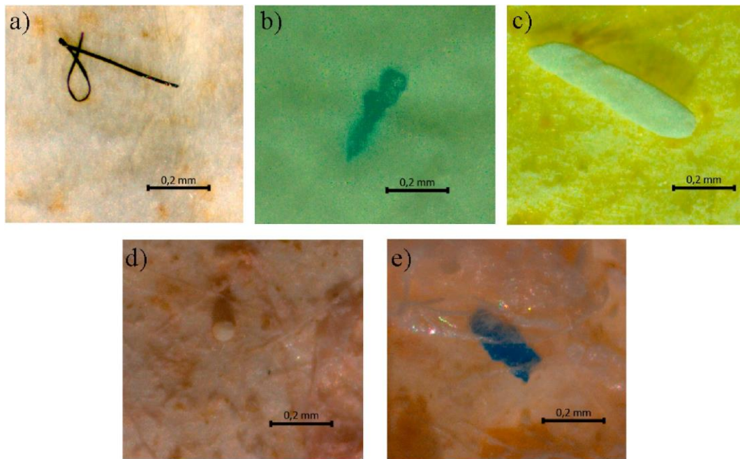
Fig. 2. Shapes of microplastics identified in the mesopelagic fishes: a) fibre; b) fragment; c) foam; d) pellet; e) film.
