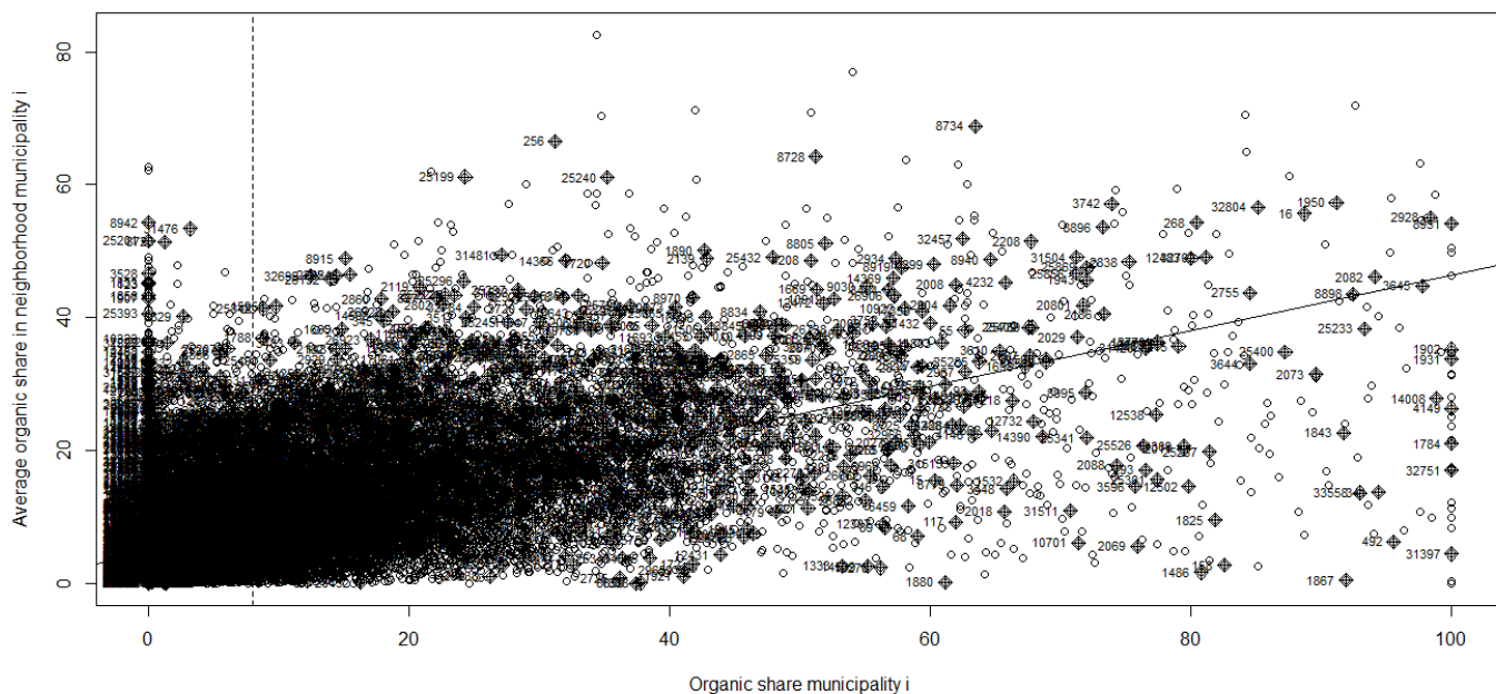
Figure 1.1: Spatial Autocorrelation Organic practice with contiguity neighborhood matrix (Moran's I)
