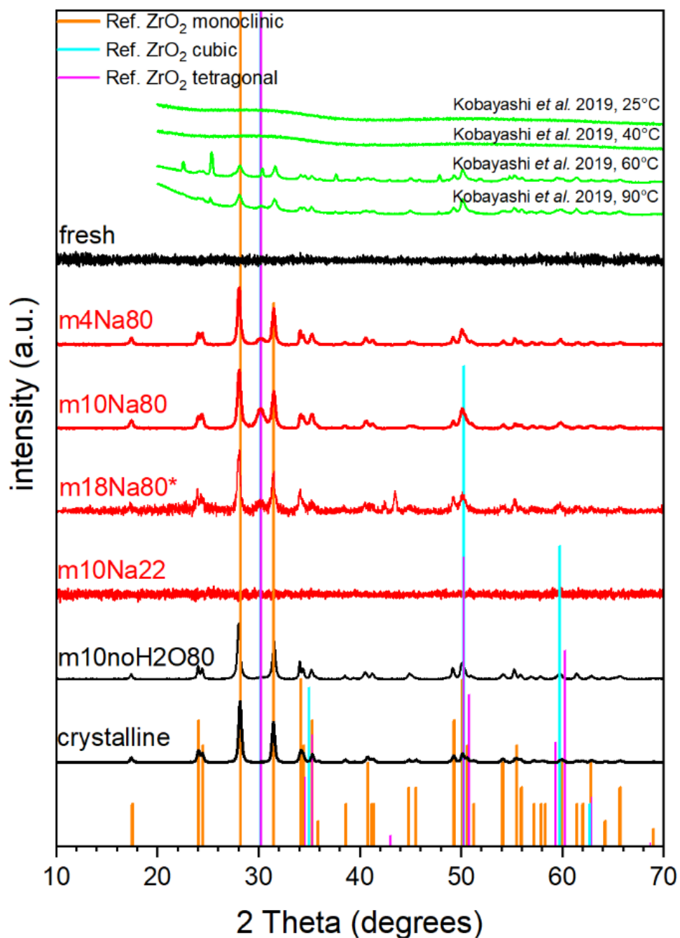
Figure 4.1: XRD patterns of ZrO 2 (s) samples: red: solid phases aged in NaOH solutions; black: freshly precipitated, aged without liquid phase and crystalline ZrO 2 (s) phases; green: diffractograms reported by Kobayashi et al. 70 . Vertical lines indicate reference data reported for ZrO 2 (cr) in the COD database 93-100 : ZrO 2 monoclinic (COD ID: 1528984), ZrO 2 tetragonal (COD ID: 1539831), ZrO 2 cubic (COD ID: 5000038).
