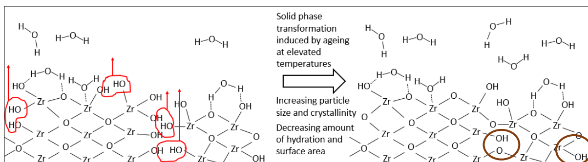
Figure 4.22: scheme of condensation reactions occurring during the ageing of the solid phases.
