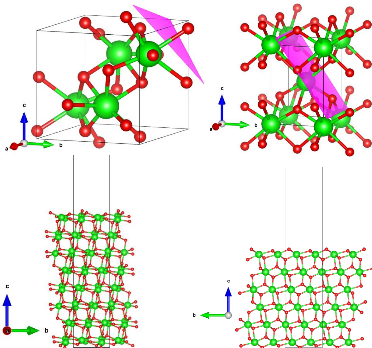
Figure 4.41: top: optimized unit cells, bottom: side view of the slabs after cutting, left: monoclinic (-1\ 1\ 1) , right: tetragonal (1\ 0\ 1) .
