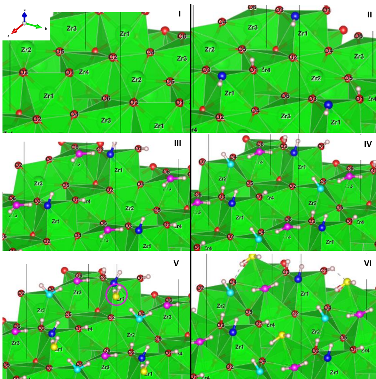
Figure 4.45: optimized monoclinic (-1\ 1\ 1) surface with (I): 0 water molecules, (II): 1 water molecule, (III): 2 water molecules, (IV): 3 water molecules, (V): 4 water molecules (1 ejected from the surface, marked with magenta circle), (VI): 4 water molecules adsorbed on the surface. Color code (for Figure 4.46-4.48): green: Zr atoms and Zr-O polyhedron, red: oxygen atoms from \text{ZrO}_2 , white: hydrogen atoms, blue: O atom of 1 st water, magenta: O atom of 2 nd water, cyan: O atom of 3 rd water, yellow: O atom of 4 th water.
