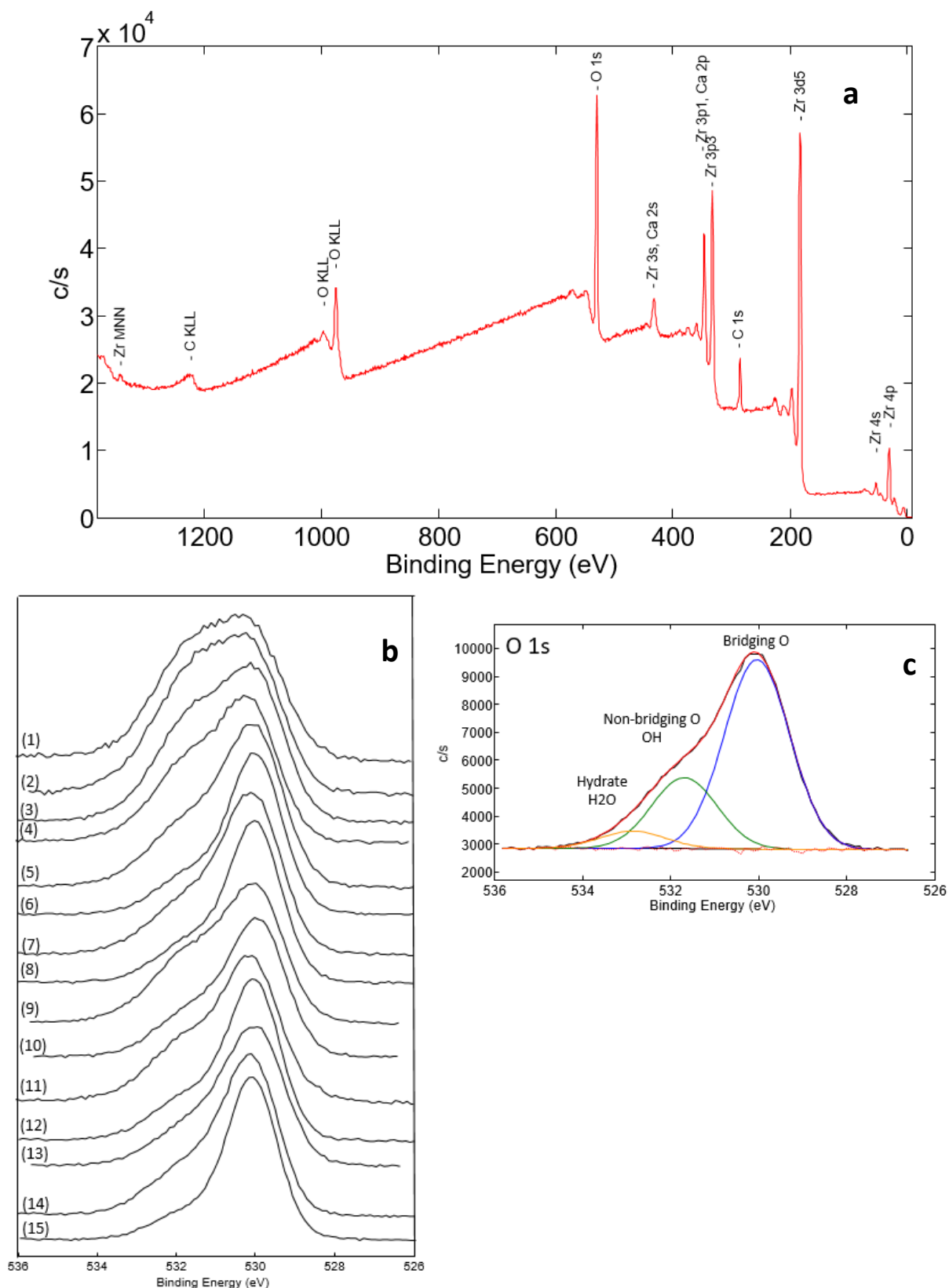
Figure 4.14: a) complete XPS spectrum of one solid, b) narrow scan of the O 1s signal of all \text{ZrO}_2 solids: (1) fresh, (2) m10Ca22, (3) m10Na22, (4) m4Ca80, (5) m4Ca80new, (6) m4_002Ca80, (7) m4_0.02Ca80new, (8) m10Ca80, (9) m10Ca80new, (10) m18Ca80, (11) m4Na80, (12) m10Na80, (13) m18Na80, (14) m10noH2O80, (15) commercial crystalline and c) an exemplary fit showing how the contributions of \text{O}^{2-} , OH and \text{H}_2\text{O} are calculated.
