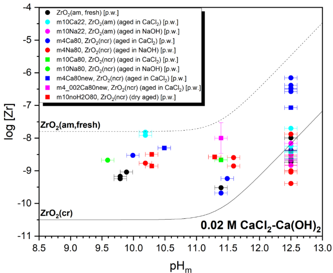
Figure 4.32: Solubility data of several solid phases, including also expected solubility curves for amorphous and crystalline solid phases based on data of NEA-TDB 17 and Altmaier et al. 19 , respectively.
