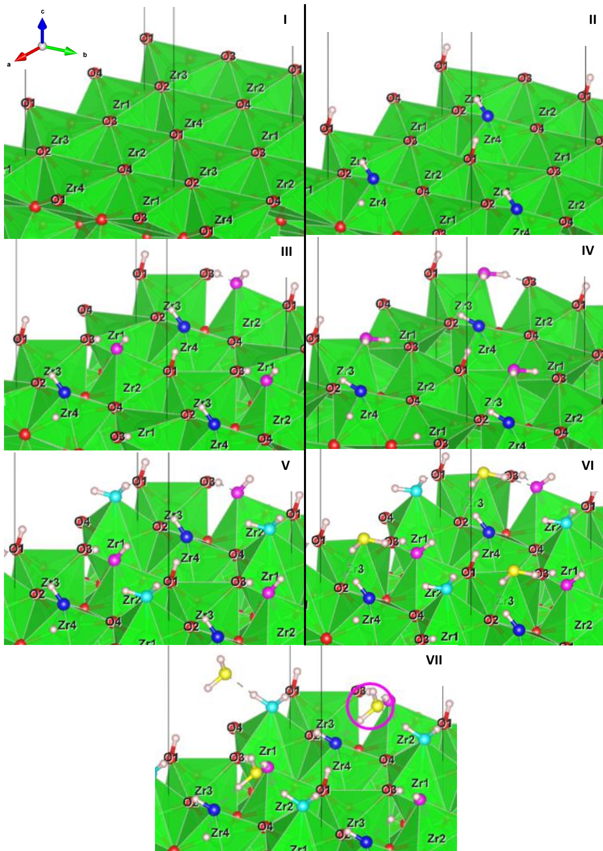
Figure 4.46: optimized tetragonal (1 0 1) surface with (I): 0 water molecules, (II): 1 water molecule, (III)+(IV): 2 water molecules, (V): 3 water molecules, (VI): 4 water molecules adsorbed on the surface, (VII): 4 water molecules (1 ejected from the surface, marked with magenta circle).
