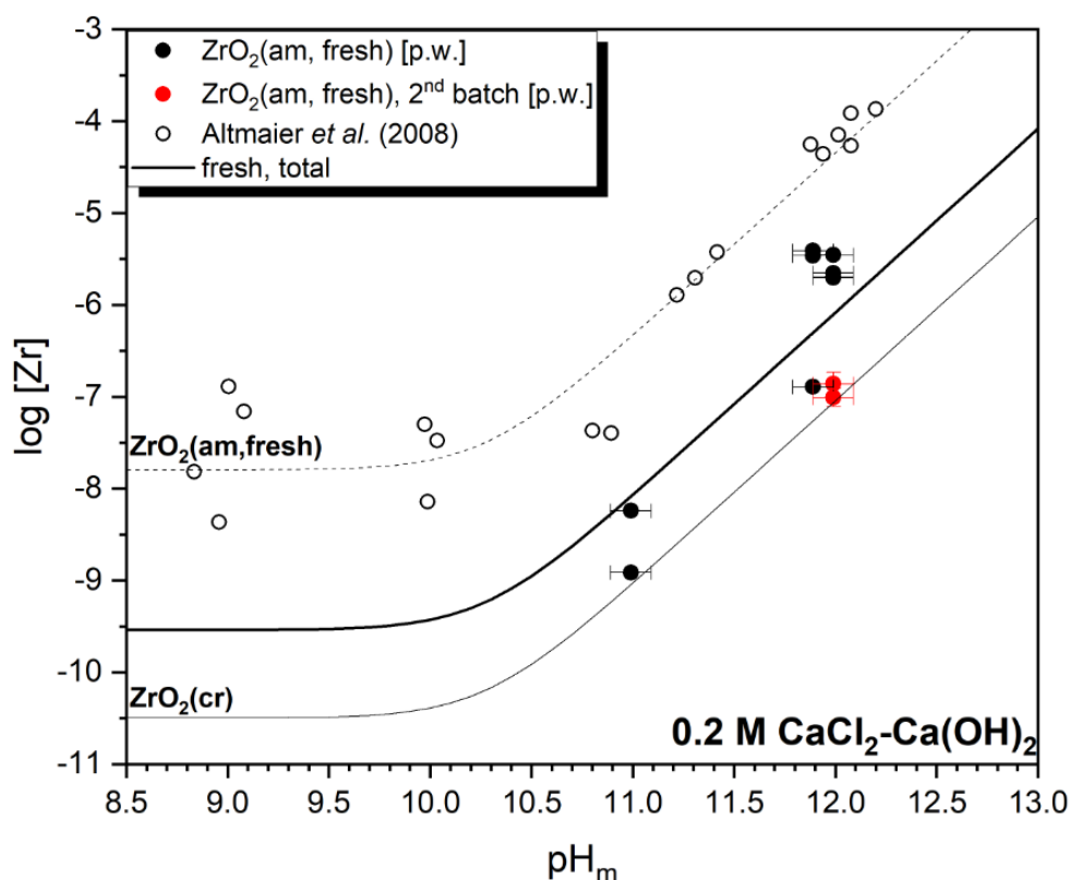
Figure 4.36: Solubility data and modelled solubility curve of the freshly precipitated \text{ZrO}_2(\text{am, hyd, fresh}) of the present work compared to data from Altmaier et al. 19 , including also expected solubility curves for amorphous and crystalline solid phases based on data of NEA-TDB 17 and Altmaier et al. 19 , respectively.
