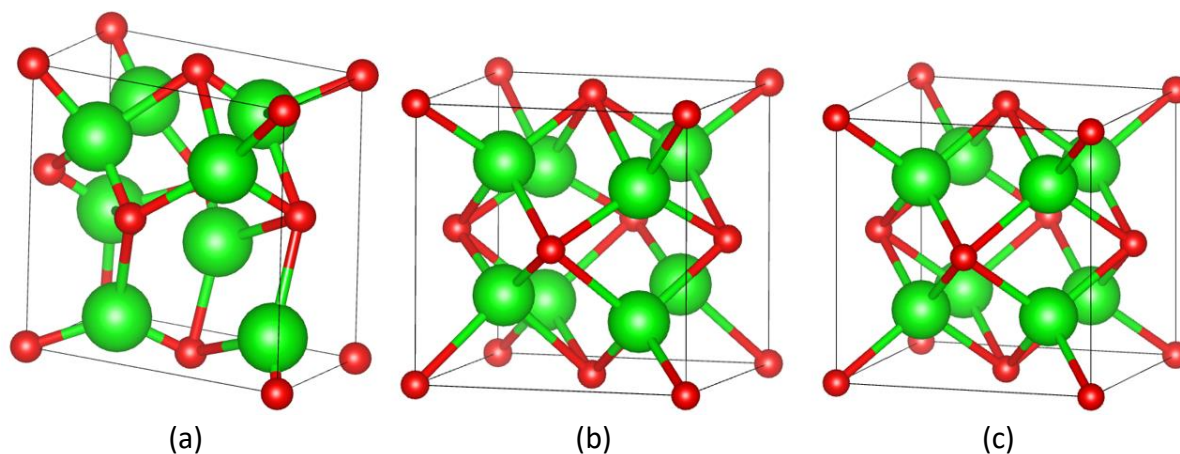
Figure 2.3: schematic structures of (a) monoclinic, (b) tetragonal and (c) cubic \text{ZrO}_2 . Adapted from 61 .
