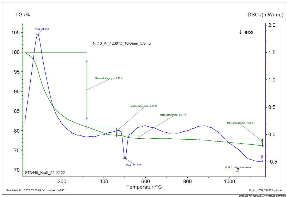
Figure A.1: TG-DTA results of the fresh (above) and m10Ca22 (below) ZrO_2(s) solid phases.
