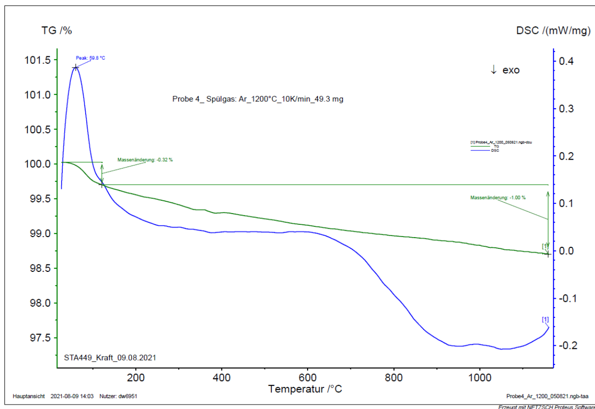
Figure A.7: TG-DTA results of the m10noH2O80 (above) and commercial crystalline (below) ZrO_2(s) solid phases.
