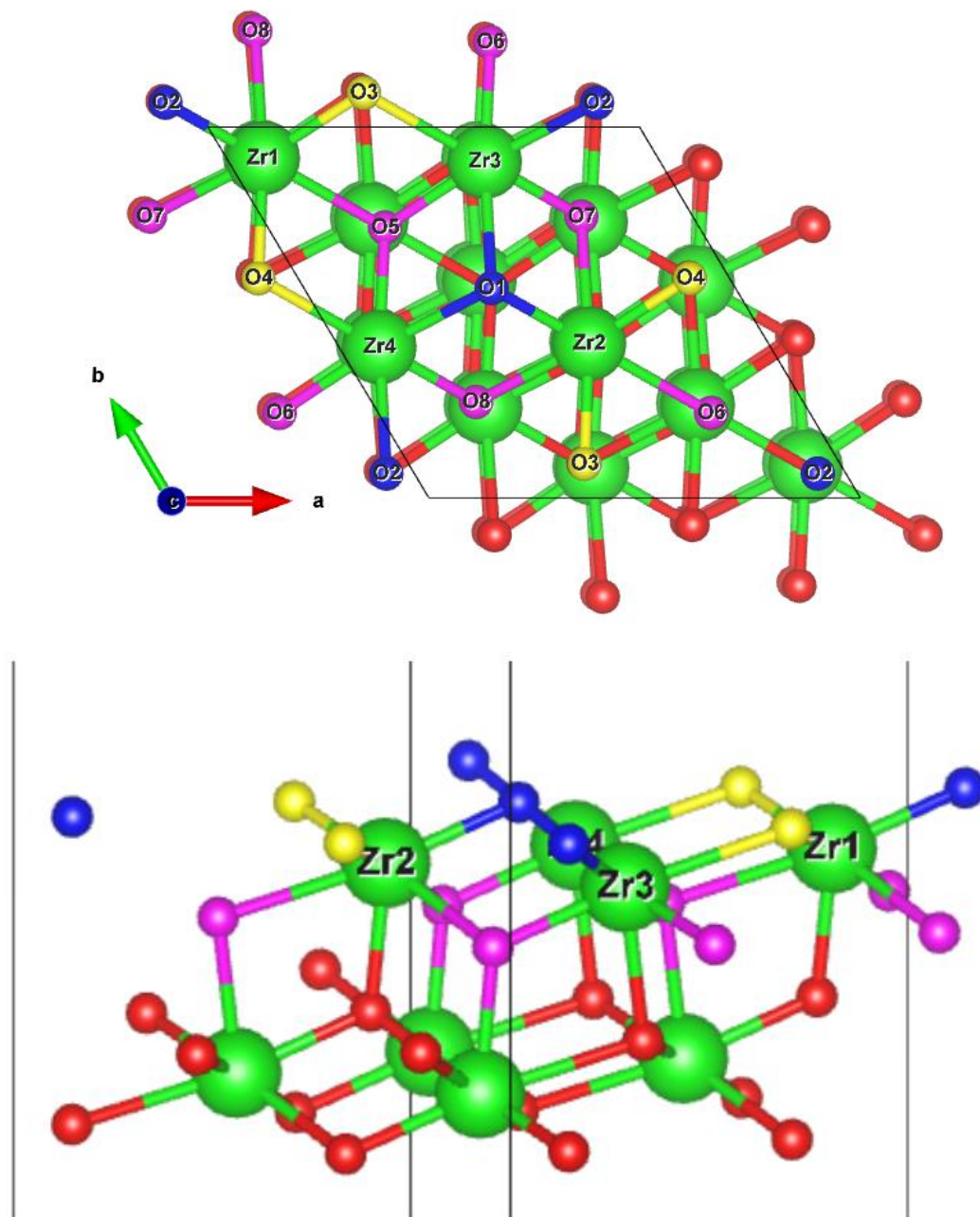
Figure 4.43: Surface coordination of the tetragonal (1 0 1) surface after optimization (top view: above, side view: below).
