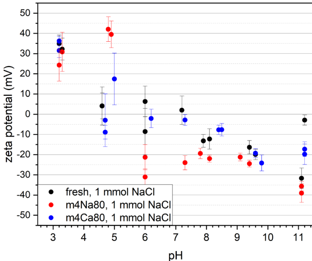
Figure 4.23: zeta potentials of fresh, m4Ca80 and m4Na80 ZrO 2 solid phases in NaCl solutions.
