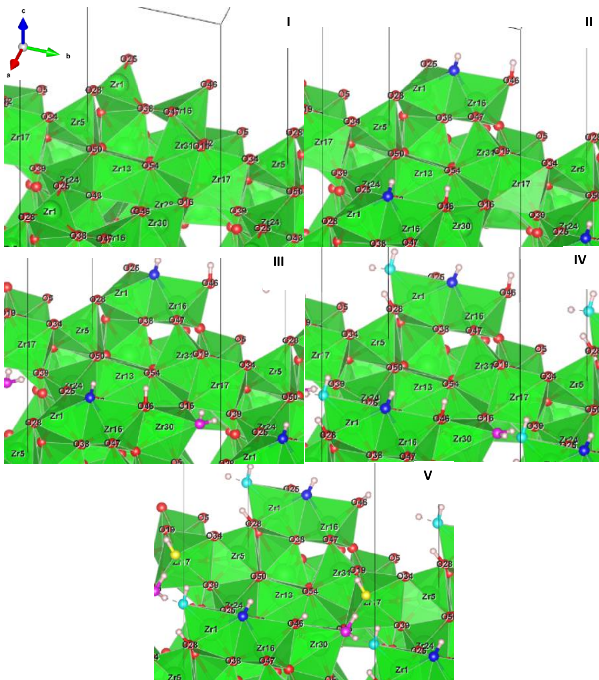
Figure 4.47: optimized amorphous surface with (I): 0 water molecules, (II): 1 water molecule, (III): 2 water molecules, (IV): 3 water molecules, (V): 4 water molecules adsorbed on the surface.
