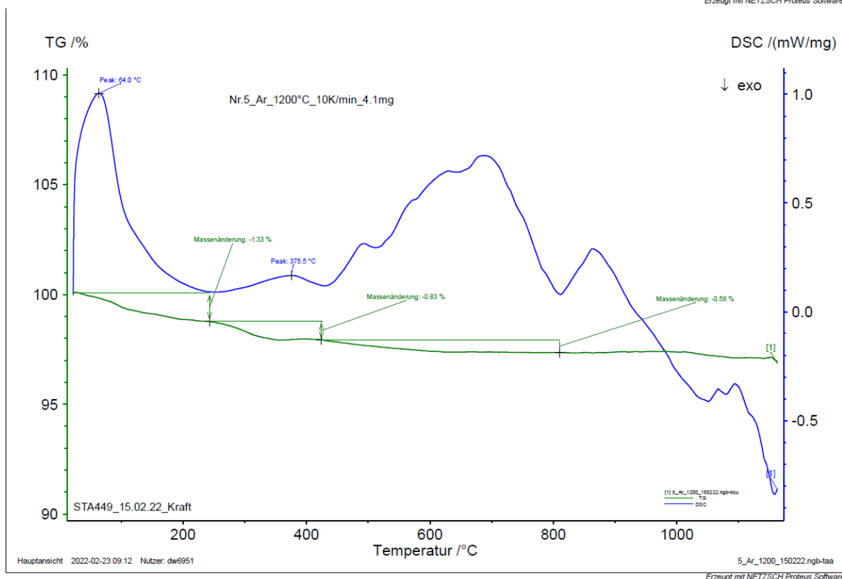
Figure A.4: TG-DTA results of the m4_002Ca80new (above) and m10Ca80 (below) ZrO 2 (s) solid phases.
