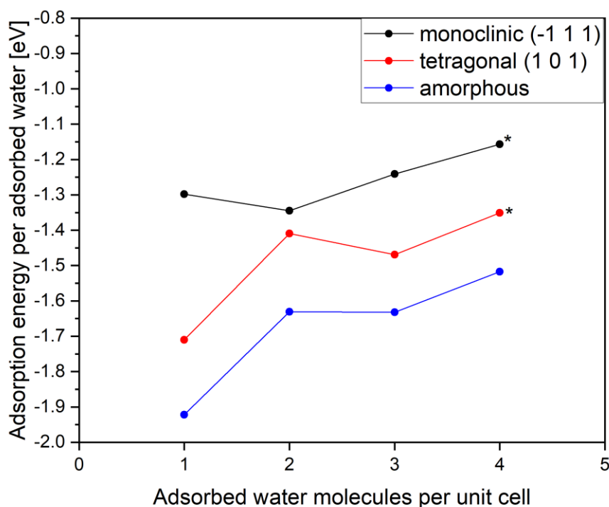
Figure 4.48: water adsorption energies on monoclinic (-1 1 1), tetragonal (1 0 1) and amorphous ZrO 2 surfaces. *marks structures with water that is not adsorbed to a surface Zr atom, but still connected to the surface by H bonds.
