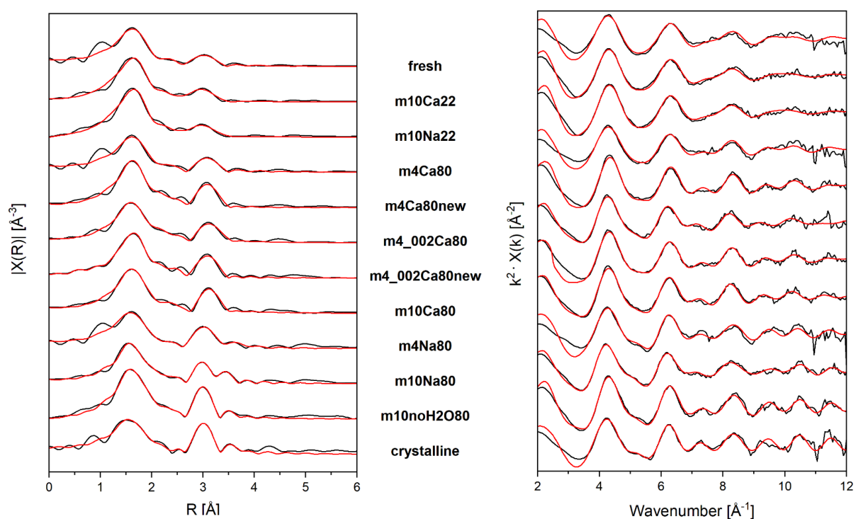
Figure 4.8: Fourier transform EXAFS spectra of the ZrO 2 (s) samples in R and k space.
