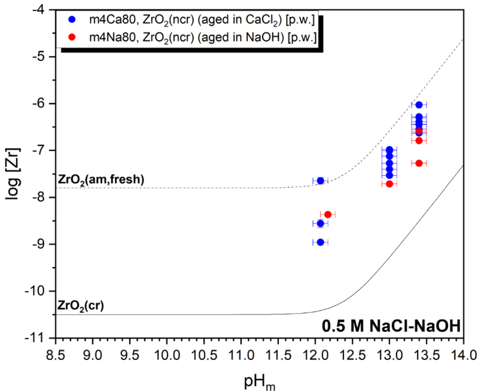
Figure 4.27: Solubility data of the aged solid phases m10Ca22 and m10Na22 (above) as well as m4Ca80 and m4Na80 (below), including also expected solubility curves for amorphous and crystalline solid phases based on data of NEA-TDB 17 and Altmaier et al. 19 , respectively.
