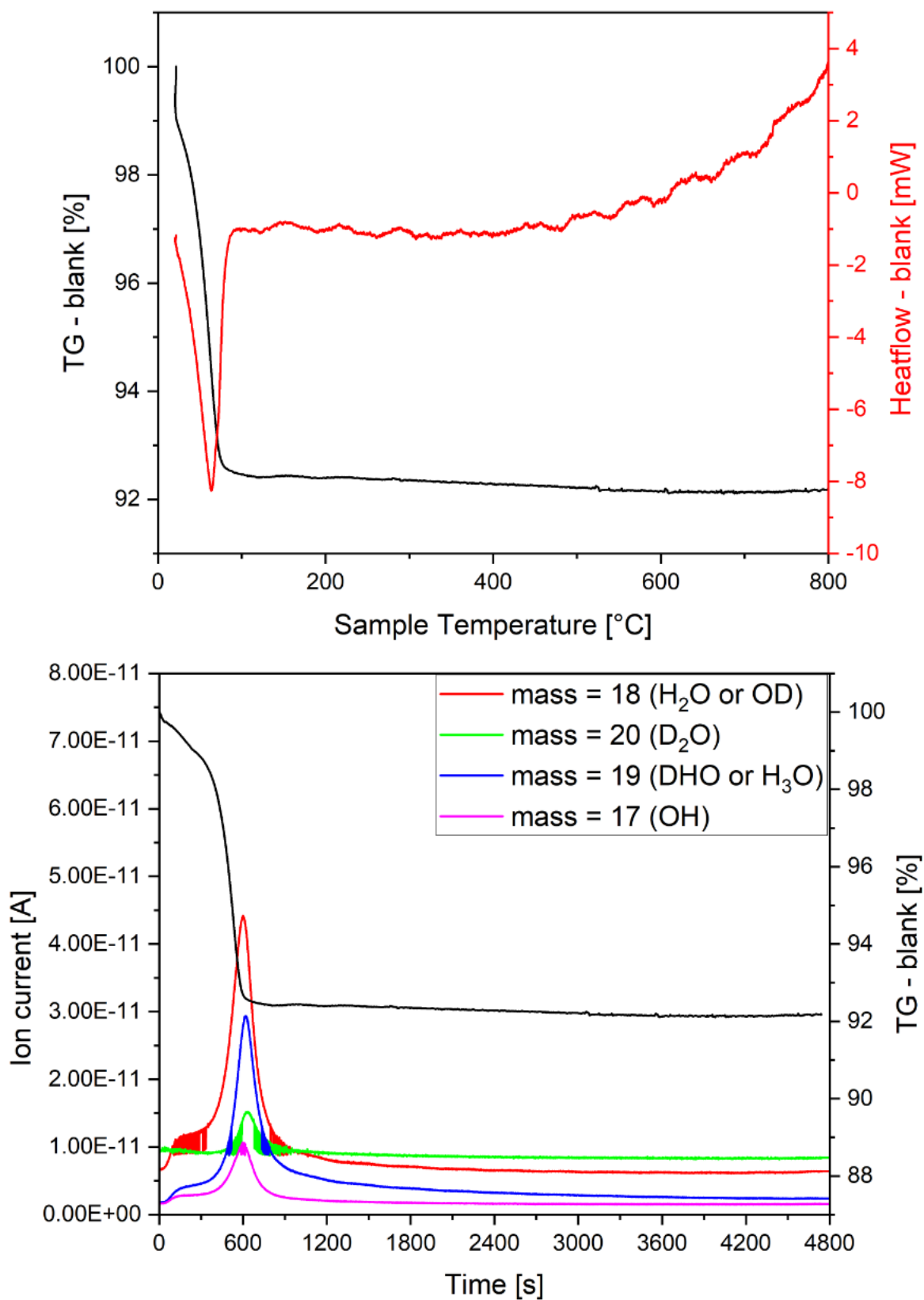
Figure 4.20: TG-DTA and TG-MS results for commercial crystalline ZrO 2 after exchange with D 2 O.
