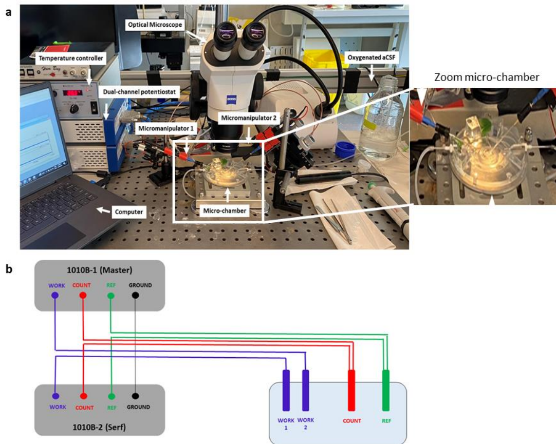
Figure 24. Setup for D-serine measurements on acute brain slices.
