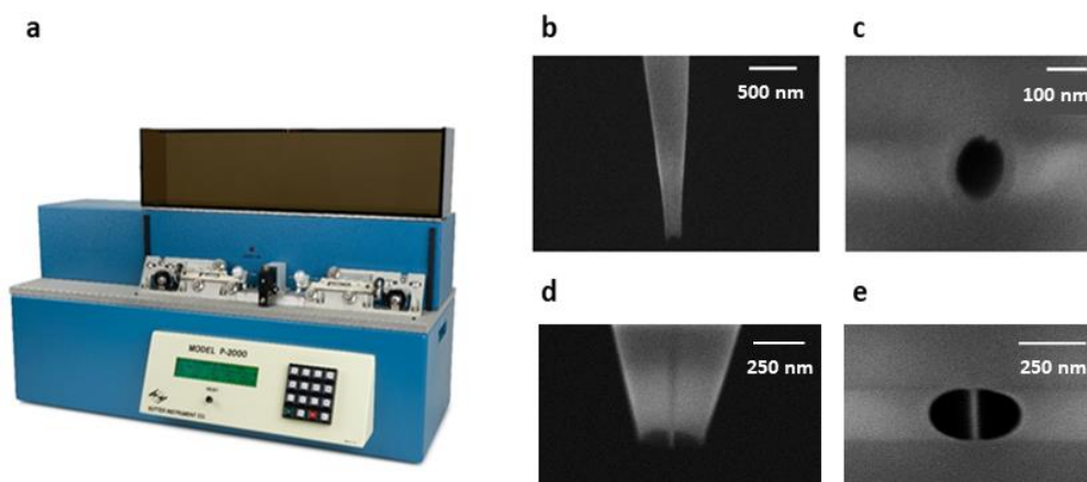
Figure 35. SICM probes fabrication.
