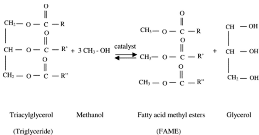
Figure 4. Production de FAME (Y. Zhang et al., 2003)
