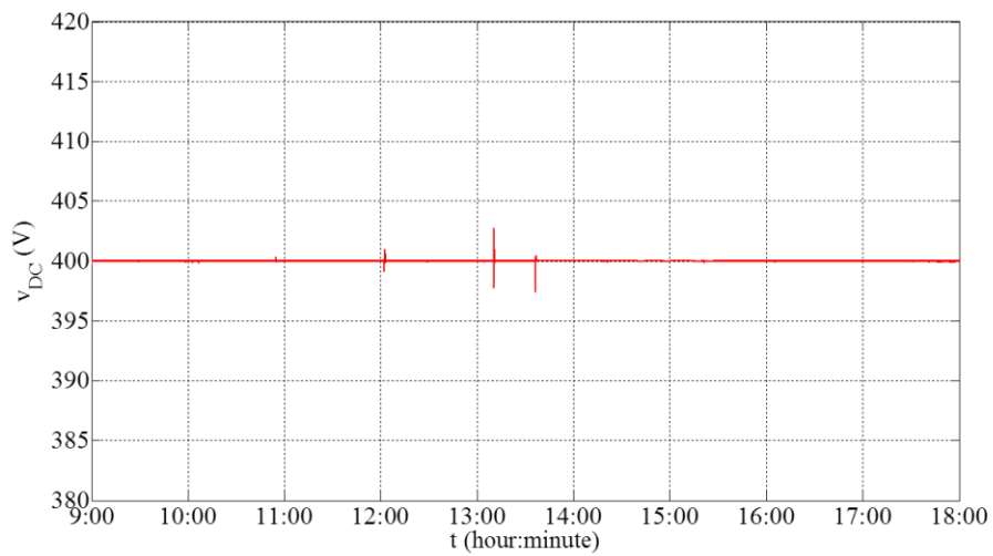
Figure 76. DC bus voltage.
