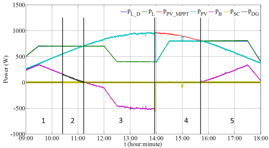
Figure 44. Power evolutions.
