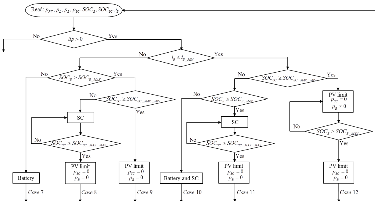
Figure 28. Flow chart of the power management strategy when PV output power is more than the required load power.
