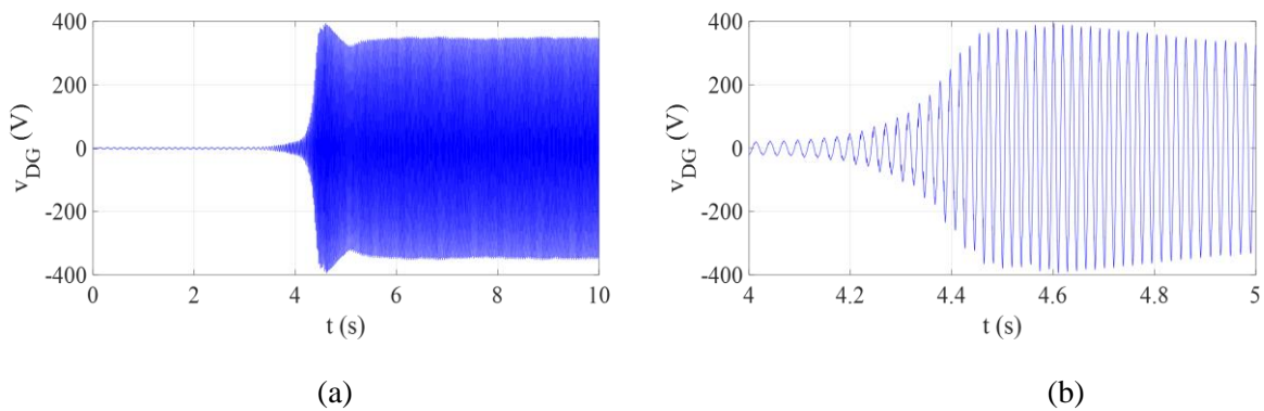
Figure 4. (a) Start-up voltage curve of DG without load and (b) the voltage curve between 4s and 5s.
