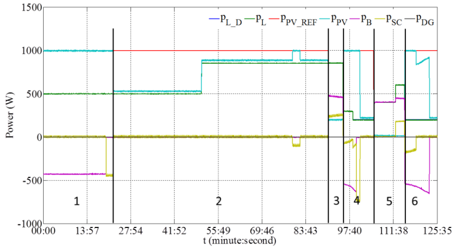
Figure 40. Power evolutions.
