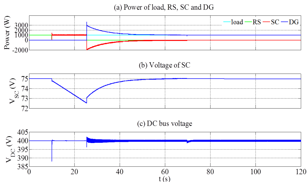
Figure 16. Dynamic response of shortage of renewable power.
