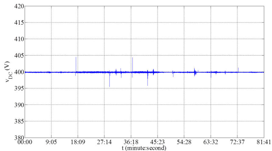
Figure 39. Evolution of DC bus voltage.
