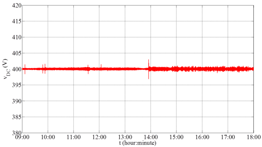
Figure 85. DC bus voltage.
