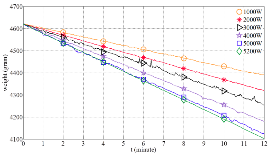
Figure 50. Declining curve of weight of fuel of different output power.
