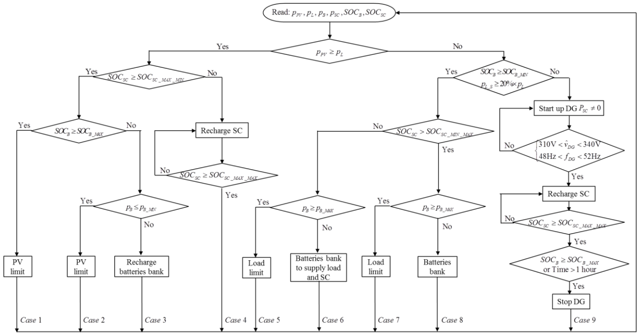
Figure 54. Flow chart of the power management strategy.
