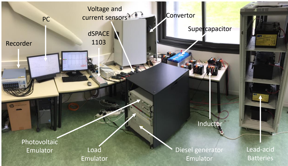
Figure 35. Image of experimental platform
