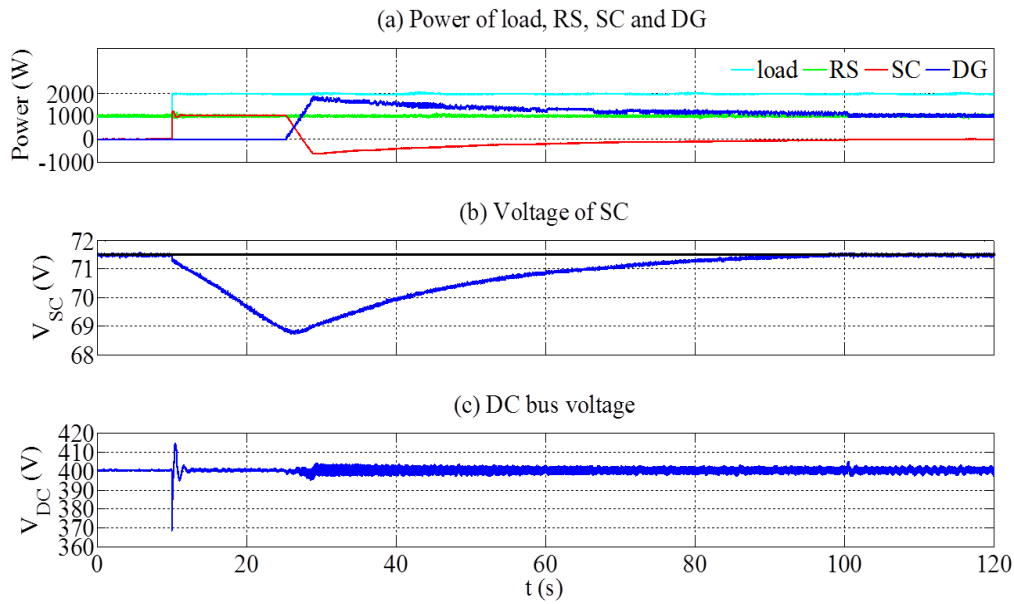
Figure 23. Dynamic response curves of microgrid parameters.
