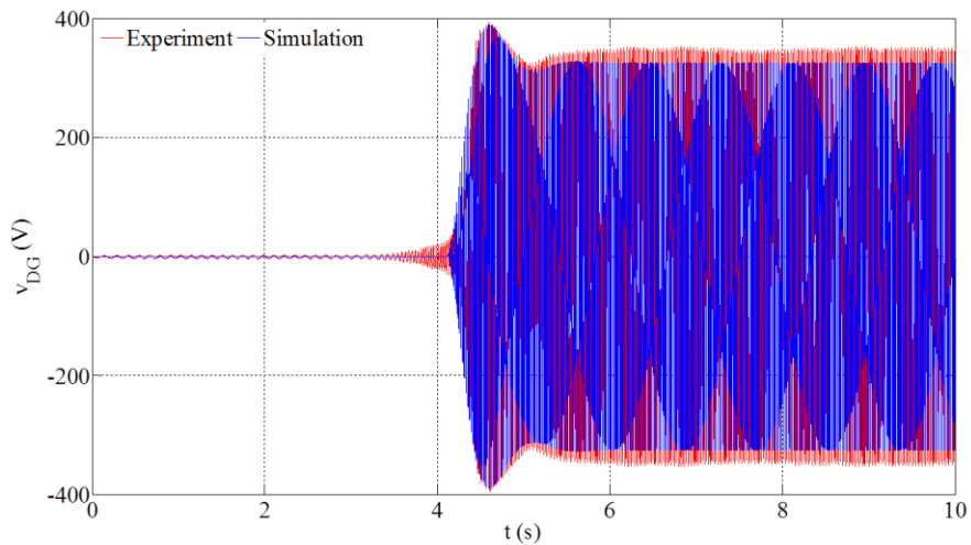
Figure 6. Start-up voltage curve of real DG and of the DG model.
