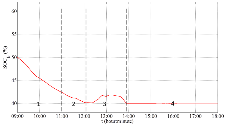
Figure 83. SOC evolution of electrochemical batteries.
