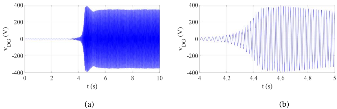
Figure 4. (a) Start-up voltage curve of DG without load and (b) the voltage curve between 4s and 5s.
