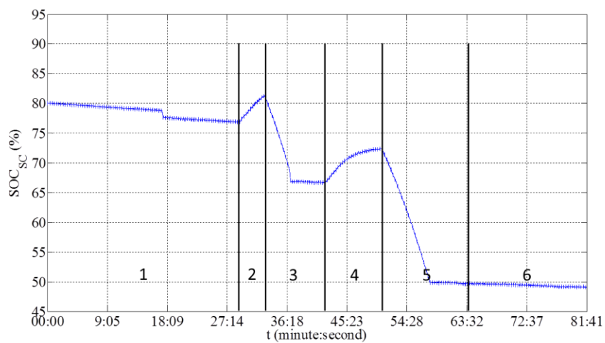
Figure 38. SOC evolution of supercapacitor.
