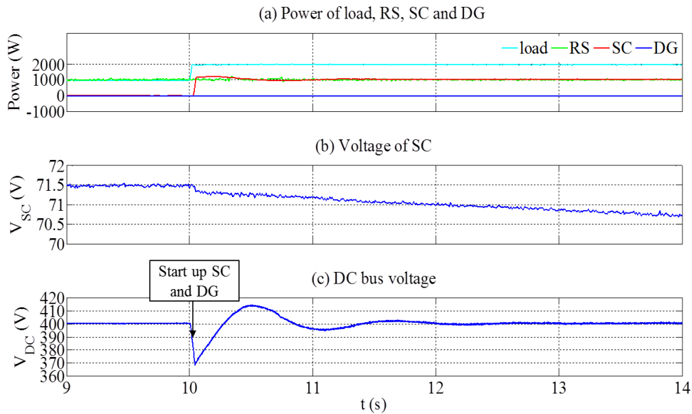
Figure 24. Detailed dynamic response curves of microgrid parameters before and after the SC connection in the case of sudden load power increase.
