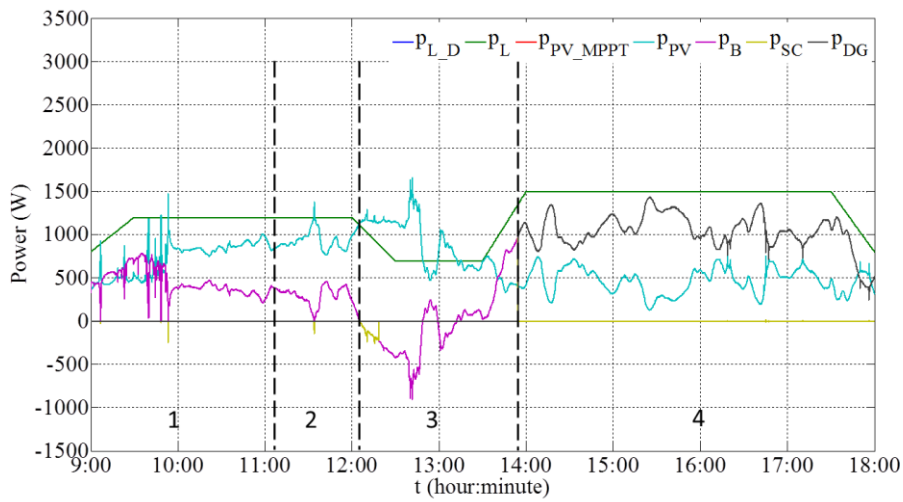
Figure 61. DC microgrid power evolutions.
