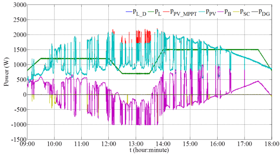
Figure 86. DC microgrid power evolutions.
