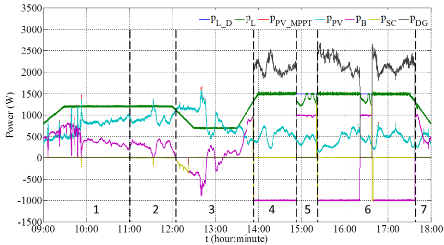
Figure 78. DC microgrid power evolutions.
