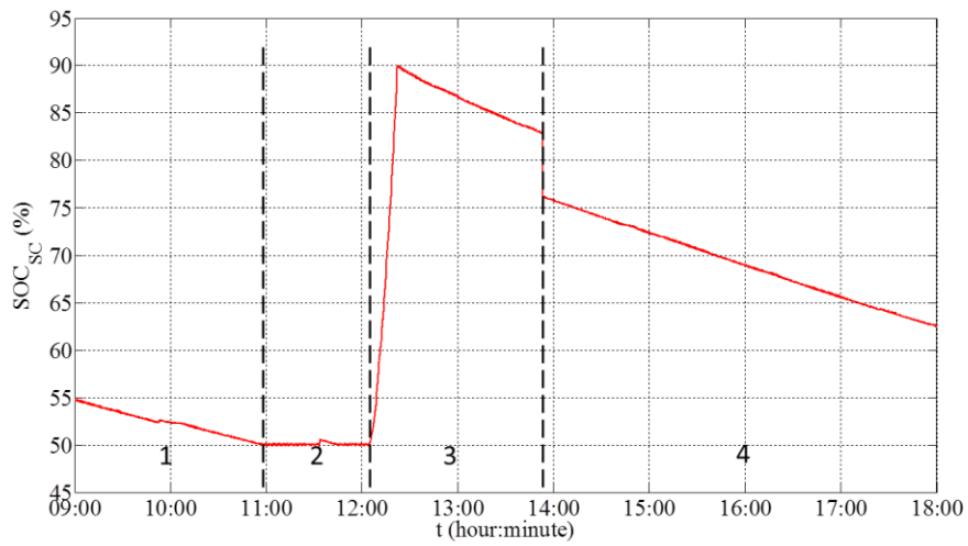
Figure 84. SOC evolution of supercapacitor.
