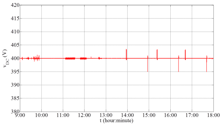
Figure 60. DC bus voltage.
