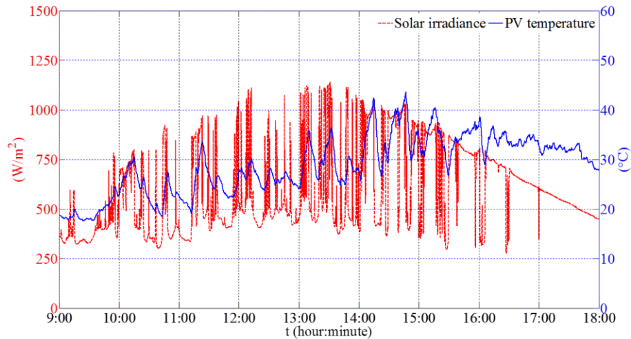
Figure 65. Solar irradiance and PV cell temperature.
