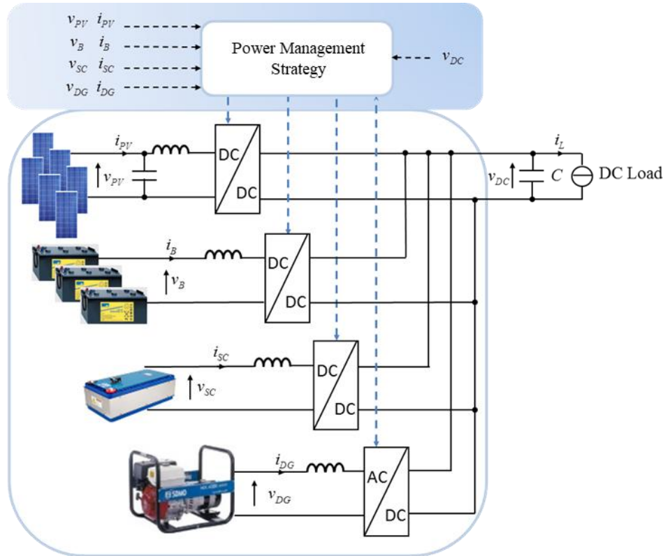
Figure 25. DC microgrid power system configuration [71].
