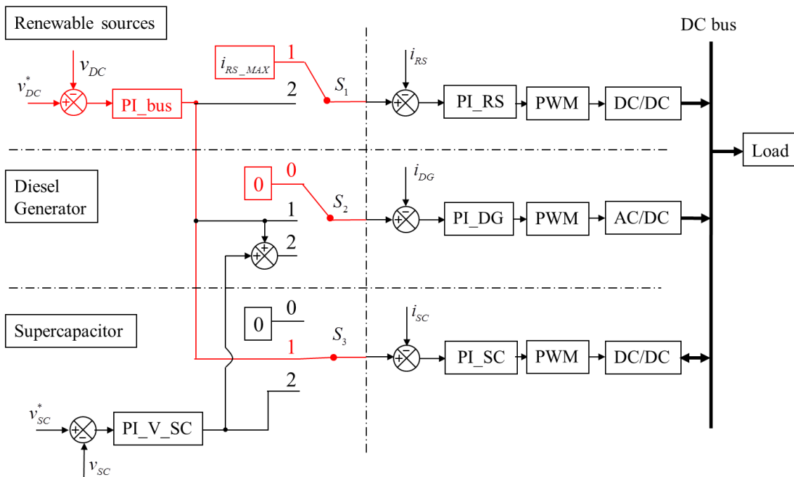
Figure 12. Control block diagram of the supercapacitor dominant mode.
