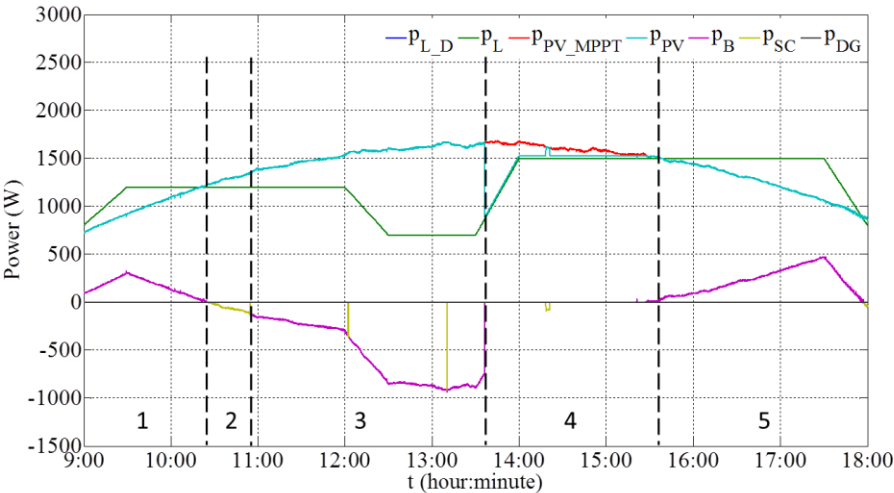
Figure 73. DC microgrid power evolutions.
