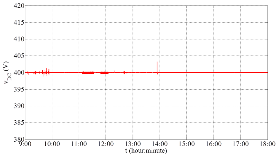
Figure 64. DC bus voltage.
