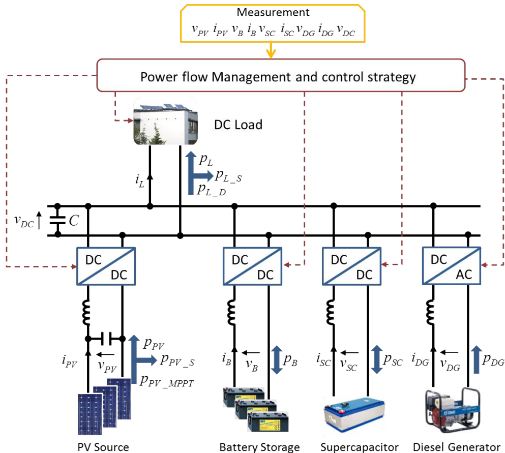
Figure 53. Topology of proposed off-grid DC microgrid system.
