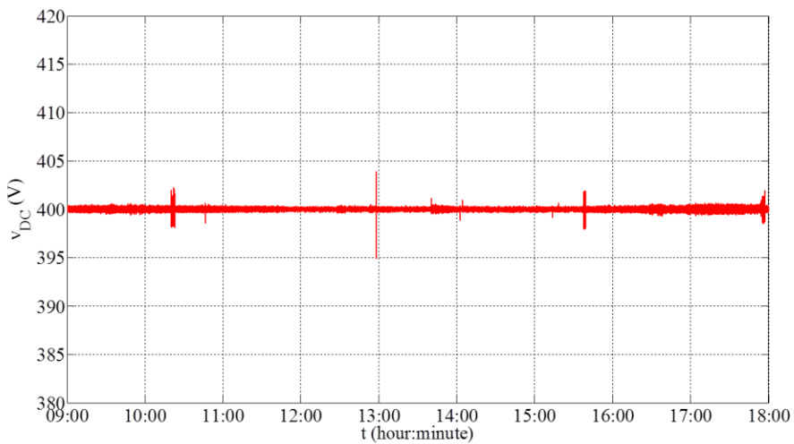
Figure 93. DC bus voltage.
