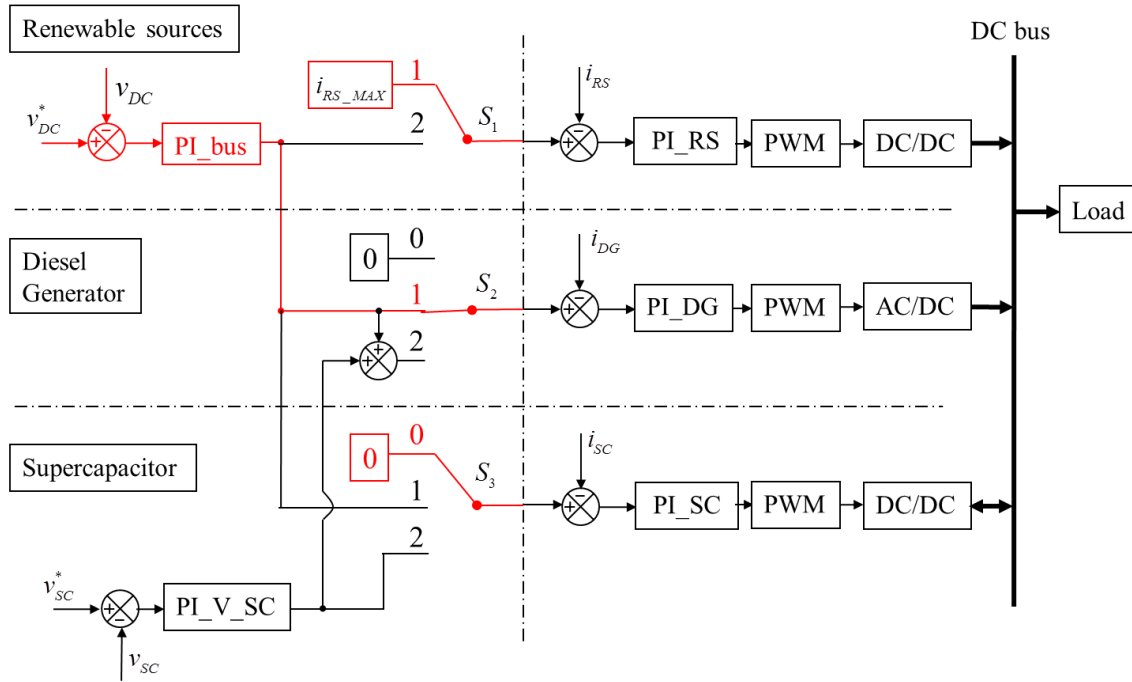
Figure 14. Control block diagram of the DG dominant mode.
