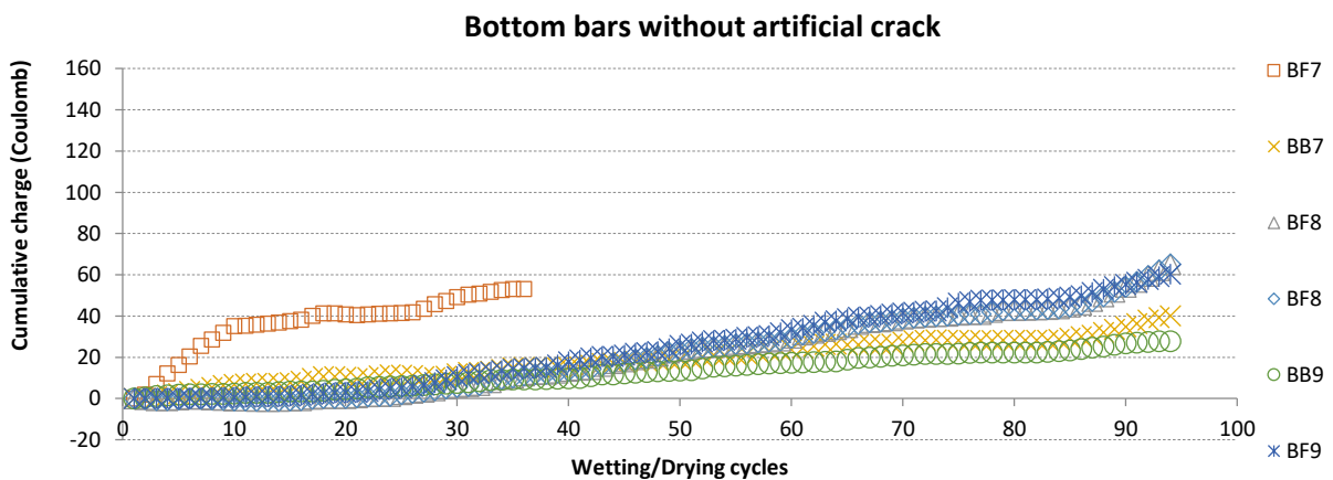
Figure 216 : Cumulative charge in Coulomb (C) for the 6 bottom-bars of sample G3-7, G3-8 and G3-9.
