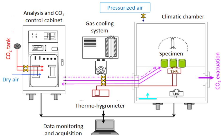
Figure 42. Climatic chamber
