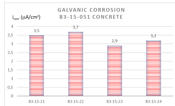
Figure 58. Concrete B3-15-051 – macro cell current density
