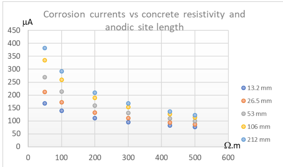
Figure 123 : Evolution of the total corrosion current in relation to the resistivity of concrete
