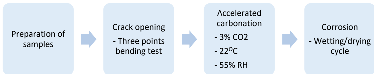
Figure 80. Process of reinforced concrete beams
