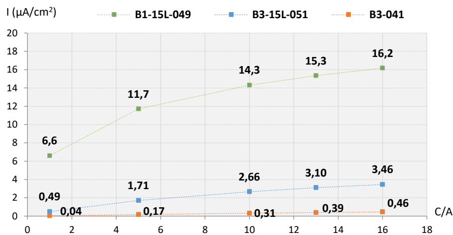
Figure 74. Macro cell corrosion vs cathode-anode ratio
