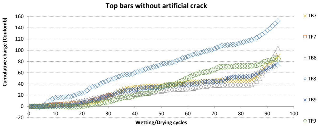
Figure 215 : cumulative charge in Coulomb (C) for the 6 top-bars of sample G3-7, G3-8 and G3-9. Top front bar of G3-07 was extracted after 30 cycles to check the corrosion
