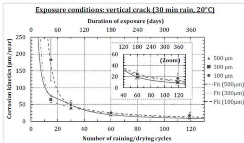
Figure 167 : corrosion kinetics versus time in Ghantous[2]
