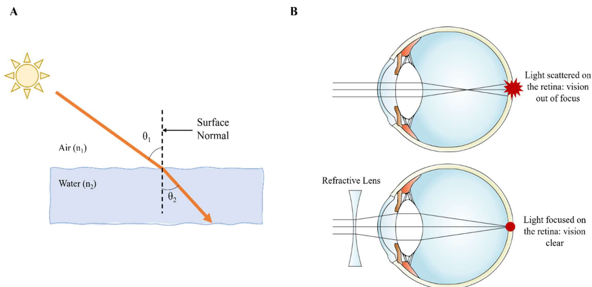
Figure 5. A visualization of refraction and one of its common applications. A) Light moves between the air and the water, distorting according to Snell's law, resulting in refraction. B) Top: light passing through the lens of a human eye exhibiting nearsightedness; Bottom: Light is filtered through a corrective lens, which refracts the light and allows the human eye to better focus the light on the retina, making vision clearer.
