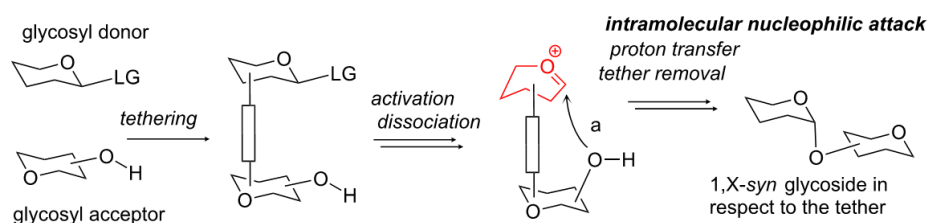
Scheme 5. The mechanistic outline of intramolecular glycosylation reaction 31
