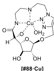
Figure 5. Proposed structure of complex #88·Cu 66
