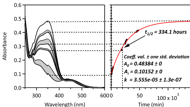
Figure 76. UV-Vis absorption spectra (left) and thermal return monitoring (right) of Z-22 \beta at 342 nm in CH 2 Cl 2 room temperature ( \approx 22-25^\circ\text{C} ). The reported data points are the result of a combination of 4 independent kinetic measurements realized on the same solution from the PSS 365 : 0 to 3720 min (step = 60 min); 18120 to 19020 min (step = 30 min); 23880 to 27600 min (step = 60 min); 44040 to 47760 min (step = 60 min).
