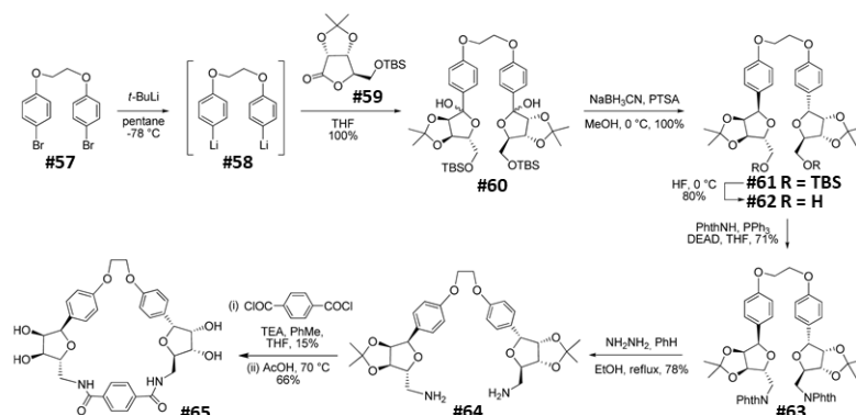
Scheme 14. Synthesis of glycothanes from ribonolactone 55
