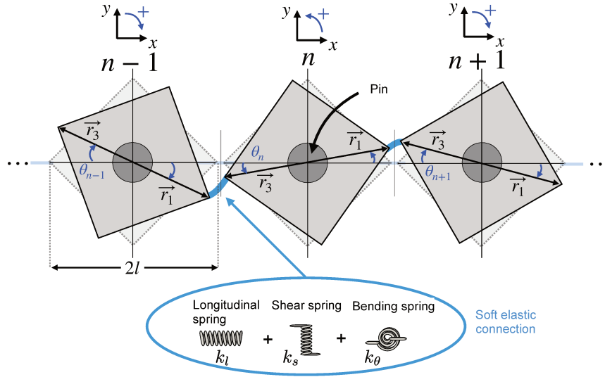
Figure 2.1: Geometry of the pinned structure. It comprises a total of N aligned rigid pinned particles, the n -th of which is connected to its direct neighbors n - 1 and n + 1 by soft elastic connections. Pins allow rotation but prevent translation.
