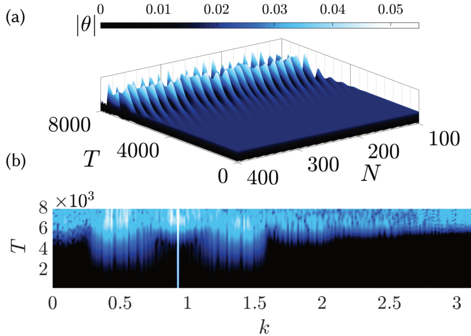
Figure 3.7: Panel (a) represents the evolution in time ( T ) of the absolute value of the rotation amplitude along the chain ( N ). Panel (b) represents the evolution in time of its k -spectrum. The result corresponds to case (I), green circle point ( k = 0.92991 , \delta = -0.003 ).
