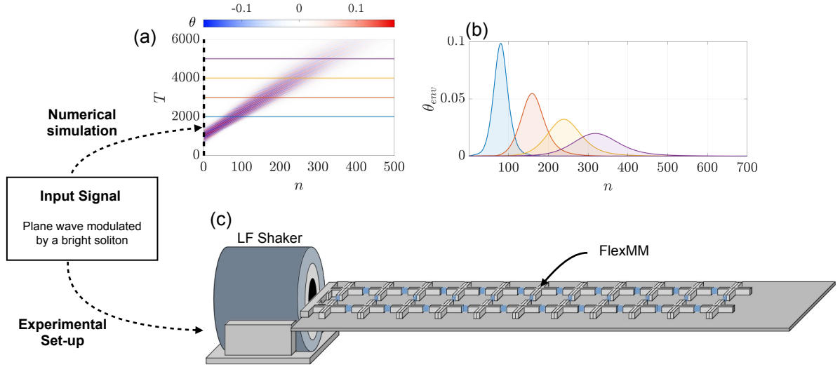
Figure 6.1: (a) Evolution of the \theta component of a bright envelope vector soliton with linear viscous damping propagating in the FlexMM. (b) Profile of the BEVS envelope at different moments. The system is excited using a driving function on the left extremity of the chain. (c) The input signal could be applied experimentally with a low-frequency (LF) shaker.
