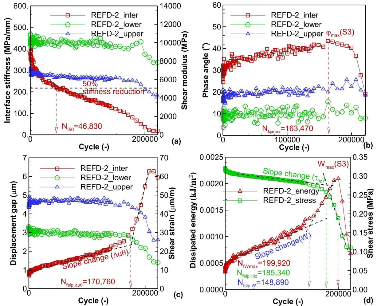
Figure 5.10: Fatigue test results for sample REFD-2 tested with \varepsilon_{\theta z g_0} = 50 \mu\text{m/m} : (a) norm of interface shear stiffness ( |K_{\theta z}^*| ), and of complex shear moduli of upper and lower layers ( |G_{\theta z,up}^*| , and |G_{\theta z,low}^*| ); (b) phase angle of interface complex shear stiffness ( \varphi_{K_{\theta z}} ), and of complex shear moduli of layers ( \varphi_{G,up} , \varphi_{G,low} ); (c) amplitude of displacement gap at the interface ( \Delta u_{\theta_0} ) and shear strains in layers ( \varepsilon_{\theta z,up_0} , \varepsilon_{\theta z,low_0} ), (d) dissipated energy at the interface ( W ) and shear stress amplitude ( \tau_{\theta z_0} )
