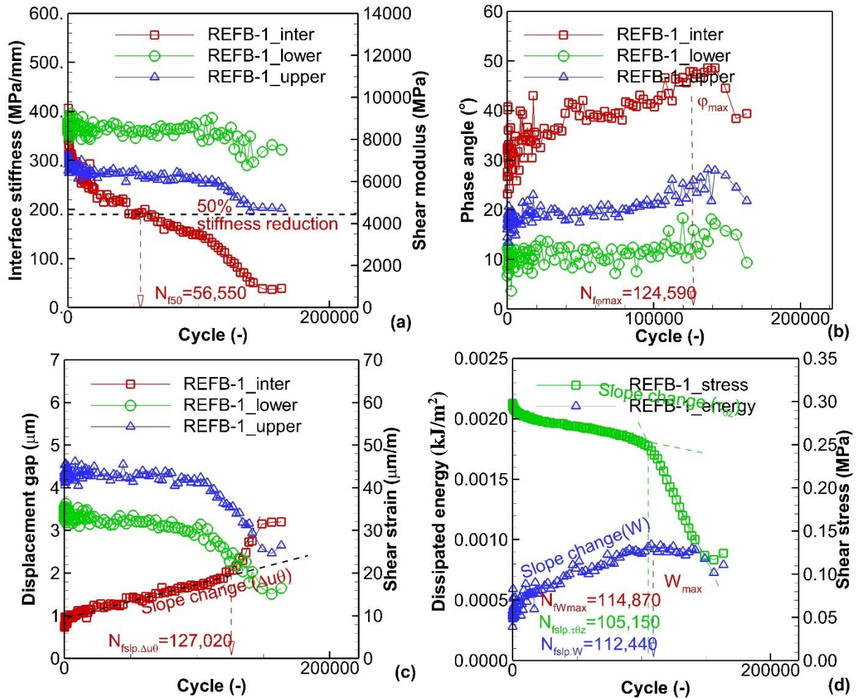
Figure B.2: Fatigue evolution for sample REF B-1 tested with \varepsilon_{\theta z g_0} = 50 \mu\text{m/m} , \sigma_{zz} = -0.026 \text{ MPa} : (a) norm of interface shear stiffness ( |K_{\theta z}^*| ), and of complex shear moduli of upper and lower layers ( |G_{\theta z, \text{up}}^*| , and |G_{\theta z, \text{low}}^*| ); (b) phase angle of interface complex shear stiffness ( \varphi_{K_{\theta z}} ), and of complex shear moduli of layers ( \varphi_{G, \text{up}} , \varphi_{G, \text{low}} ); (c) amplitude of displacement gap at the interface ( \Delta u_{\theta_0} ) and shear strains in layers ( \varepsilon_{\theta z, \text{up}_0} , \varepsilon_{\theta z, \text{low}_0} ), (d) dissipated energy at the interface ( W ) and shear stress amplitude ( \tau_{\theta z_0} )
