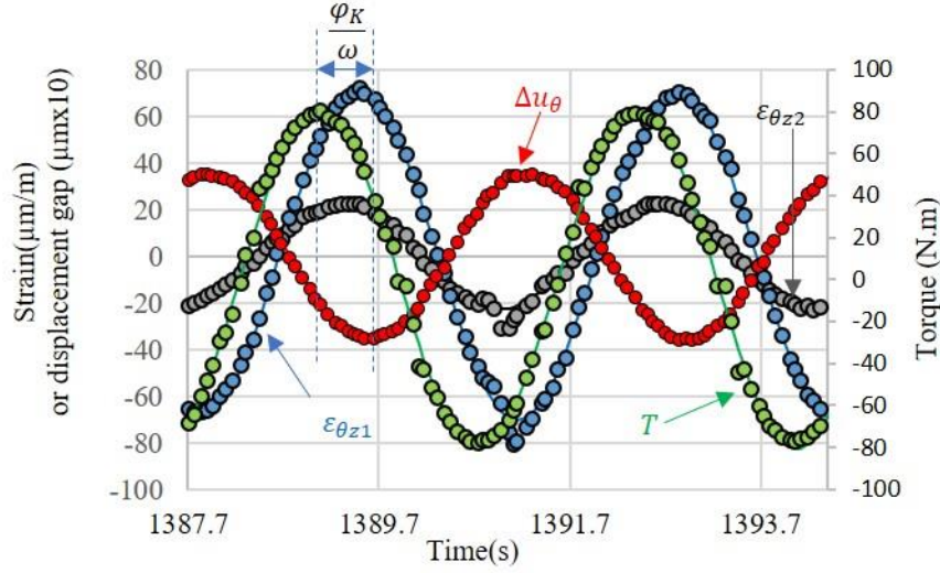
Figure 4.1: Example of 2-cycle signals recorded from shear complex modulus test of sample REFA-3 at 20°C, 0.3 Hz, global shear strain of 50 μm/m: Torque ( T ), shear strain in upper layer ( \epsilon_{\theta z.up} ), shear strain in lower layer ( \epsilon_{\theta z.low} ), and displacement gap at the interface ( \Delta u_{\theta} )
