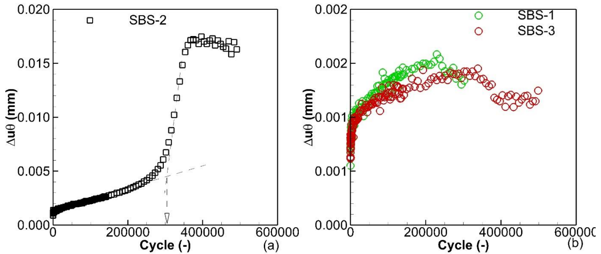
Figure 5.28: Evolution of displacement gap at the interfaces during fatigue tests of three samples tested with \varepsilon_{\theta z g_0} = 50 \mu\text{m/m} , \sigma_{zz} = 0.0026 \text{ MPa} : (a) SBS-2; (b) SBS-1 and SBS-3
