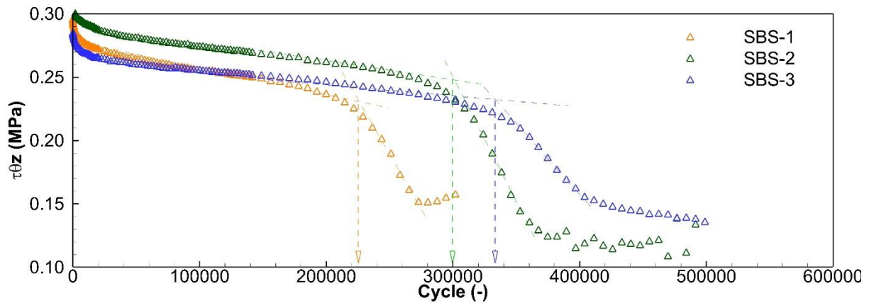
Figure 5.29: Evolution of shear stresses during fatigue tests of three samples with the interface using polymer-modified bitumen tested with \varepsilon_{\theta z g_0} = 50 \mu\text{m/m} , \sigma_{zz} = 0.0026 \text{ MPa}
