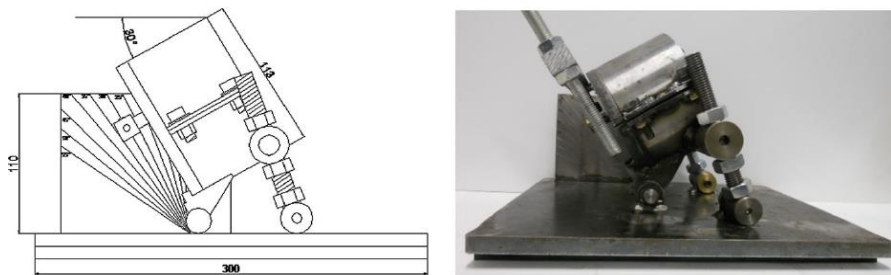
Figure 1.15: Schematic and a picture of Sapienza inclined shear test machine (SISTM) (D'Andrea & Tozzo, 2016)
