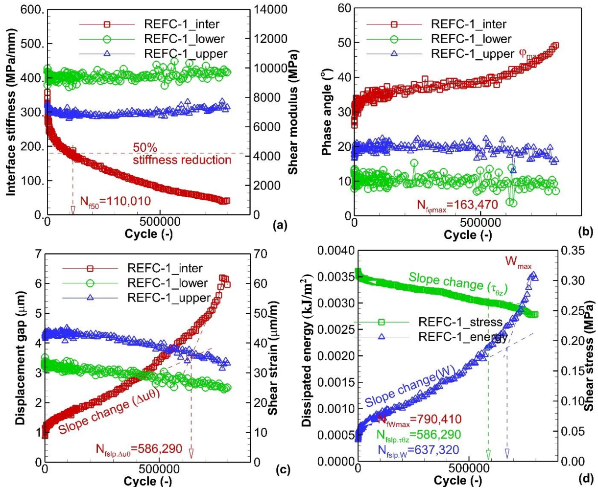
Figure B.4: Fatigue evolution for sample REFC-1 tested with \varepsilon_{\theta z,0} = 50 \mu\text{m/m} , \sigma_{zz} = -0.125 MPa: (a) norm of interface shear stiffness ( |K_{\theta z}^*| ), and of complex shear moduli of upper and lower layers ( |G_{\theta z,up}^*| , and |G_{\theta z,low}^*| ); (b) phase angle of interface complex shear stiffness ( \varphi_{K_{\theta z}} ), and of complex shear moduli of layers ( \varphi_{G,up} , \varphi_{G,low} ); (c) amplitude of displacement gap at the interface ( \Delta u_{\theta 0} ) and shear strains in layers ( \varepsilon_{\theta z,up,0} , \varepsilon_{\theta z,low,0} ), (d) dissipated energy at the interface ( W ) and shear stress amplitude ( \tau_{\theta z,0} )
