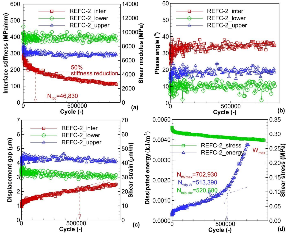
Figure B.5: Fatigue evolution for sample REFC-2 tested with \varepsilon_{\theta z g,0} = 50 \mu\text{m/m} , \sigma_{zz} = -0.125 \text{ MPa} : (a) norm of interface shear stiffness ( |K_{\theta z}^*| ), and of complex shear moduli of upper and lower layers ( |G_{\theta z,up}^*| , and |G_{\theta z,low}^*| ); (b) phase angle of interface complex shear stiffness ( \varphi_{K_{\theta z}} ), and of complex shear moduli of layers ( \varphi_{G,up} , \varphi_{G,low} ); (c) amplitude of displacement gap at the interface ( \Delta u_{\theta,0} ) and shear strains in layers ( \varepsilon_{\theta z,up,0} , \varepsilon_{\theta z,low,0} ), (d) dissipated energy at the interface ( W ) and shear stress amplitude ( \tau_{\theta z,0} )
