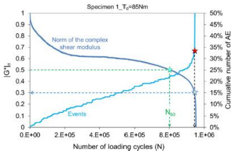
Figure 1.43: Evolution of cumulative AE events and normalised |G^*| during a shear-torque fatigue test (Ragni, Takarli, et al., 2020)
