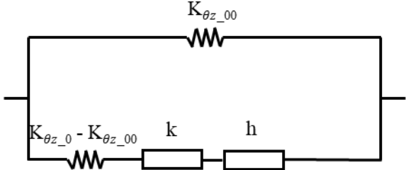
Figure 1.36: Huet-Sayegh model
