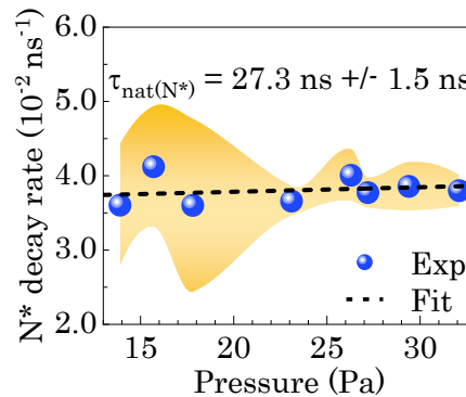
Figure 3.6: Stern-Volmer plot depicting the excited N atom's decay rate during the fluorescence emission w.r.t the working pressure (Pa). Each data point (blue circle) represents the lifetime of the de-excitation process, which produces the fluorescence ( \tau_{N^*} ). The yellow gradient in the background depicts the error bar of the data set.
