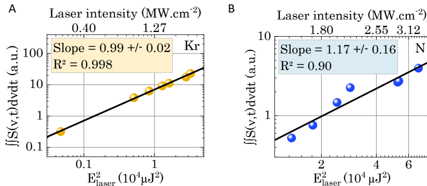
Figure 3.7: Temporally integrated TALIF signal as a function of the square of the laser energy for A. Krypton and B. Nitrogen.
