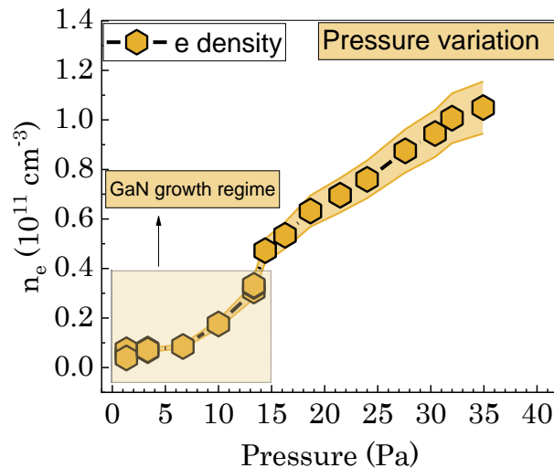
Figure 3.10: Electron density ( n_e ) plotted vs the working pressure range of 0-35 Pa. The patterned inset from 2-15 Pa depicts the growth regime that was used to deposit GaN.
