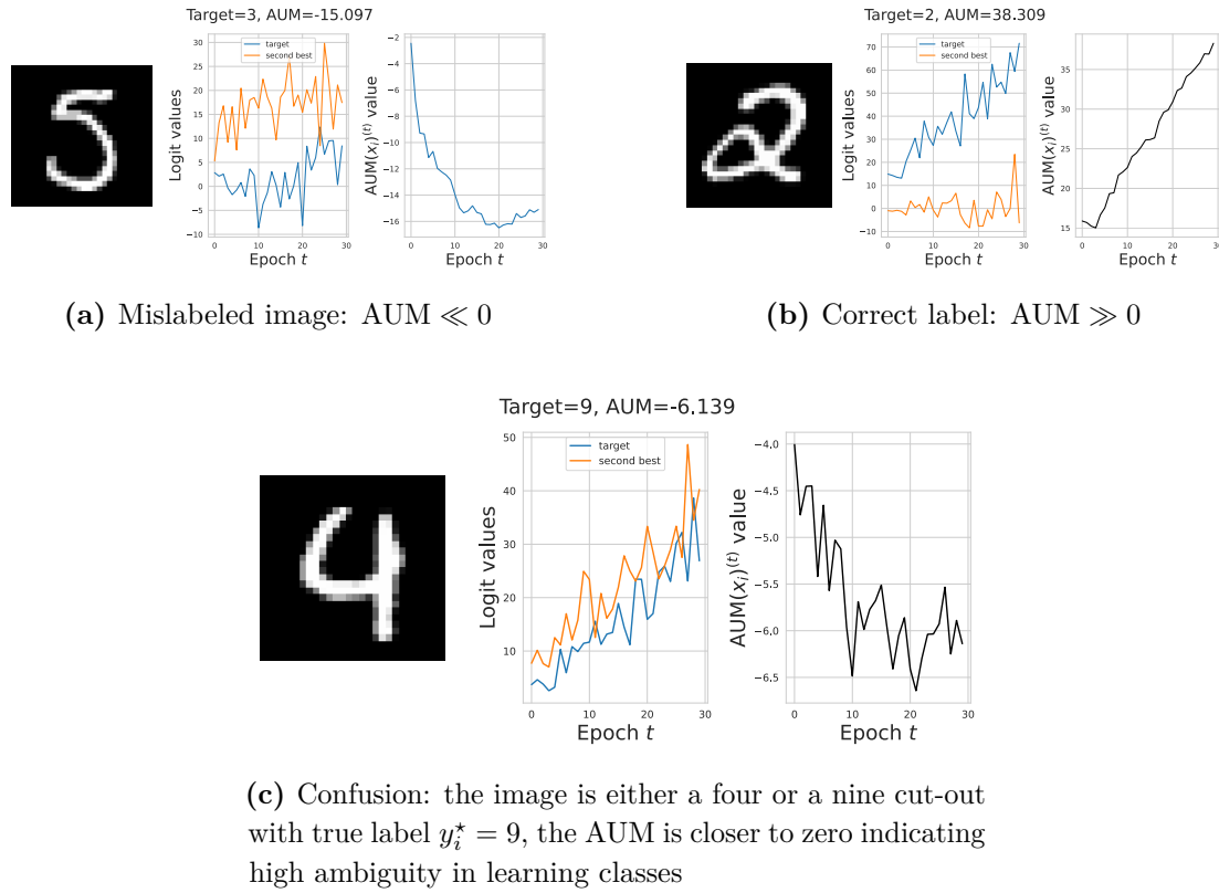
Figure 2.2 Three examples from the MNIST dataset to illustrate the behavior of the AUM: if the sample is mislabeled the AUM is low as the classifier disagrees with the given label. Note that if T > 0 is too high the memorization kicks in and the AUM increases again. When the sample is correctly labeled the AUM increases over training. When the sample is ambiguous, the AUM is closer to 0. Results are from a 2-layer convolution network with max-pooling. Training is done in T = 30 epochs using Adam optimizer with a learning rate set to 0.01 and batches of 100 samples.
