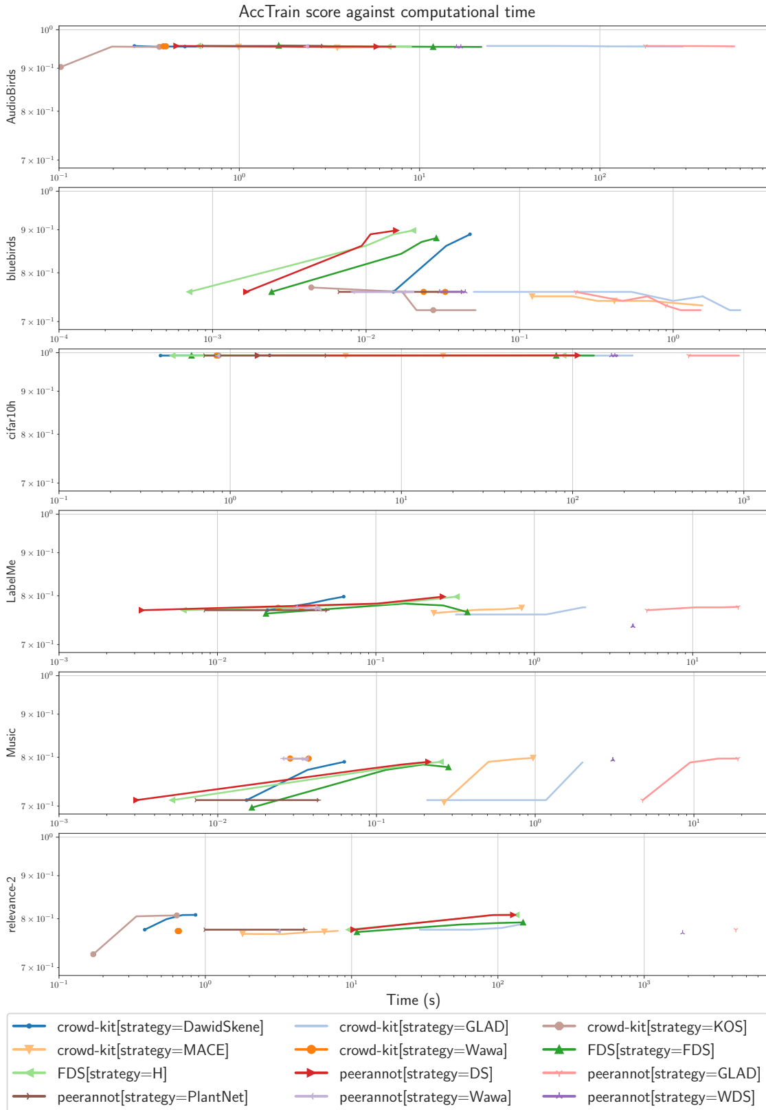
Figure 3.18 AccTrain score against computational time depending on the crowdsourced dataset and solver.
