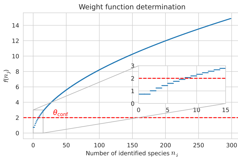
Figure 4.13 Weight function in Equation (4.1) used to map the number of identified species to a trust score in the Pl@ntNet label aggregation strategy. A new user starts with a weight of f(0) = f(1) = \gamma \simeq 0.74 . The user confidence threshold \theta_{\text{conf}} = 2 requires a user to have identified at least n_j = 8 species to become self-validating . The parameters \alpha = 0.5 , \beta = 0.2 and \gamma \simeq 0.74 are used in practice.
