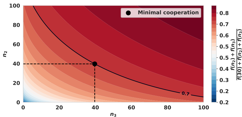
Figure 4.22 Minimal number of identified species n_2 and n_3 for two users to validate an observation with a common disagreeing vote if the author has n_1 = 30 identified species. The \theta_{\text{acc}} threshold is \frac{f(n_2)+f(n_3)}{f(n_1)+f(n_2)+f(n_3)} and must be greater than \theta_{\text{acc}} = 0.7 .
