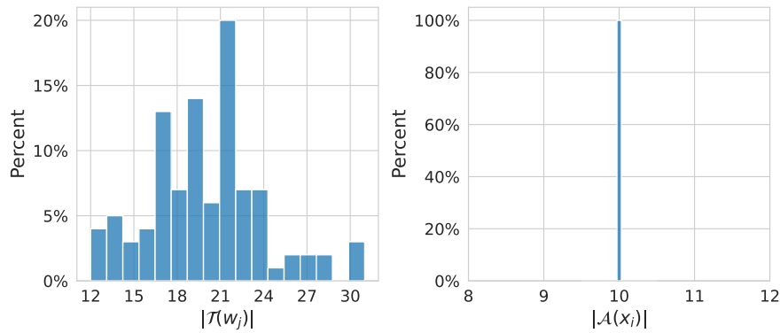
Figure B.1 Distribution of the number of tasks given per worker (left) and of the number of labels per task (right) in the setting with simulated discrete difficulty levels.
