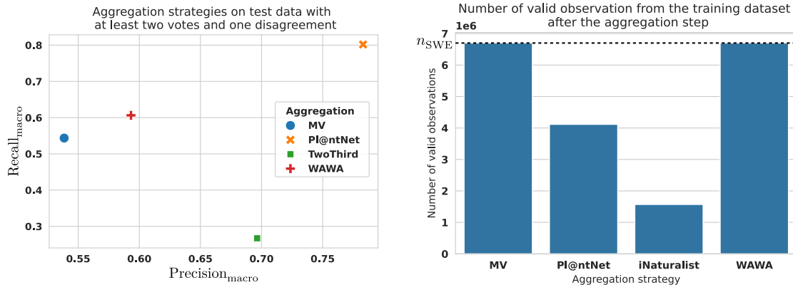
(a) Precision and recall of label aggregation strategies on \mathcal{D}_{\text{disagreement}} . (b) Number of observations in \mathcal{D}_{\text{SWE}} indicated as valid for training ( s_i = 1 ).
