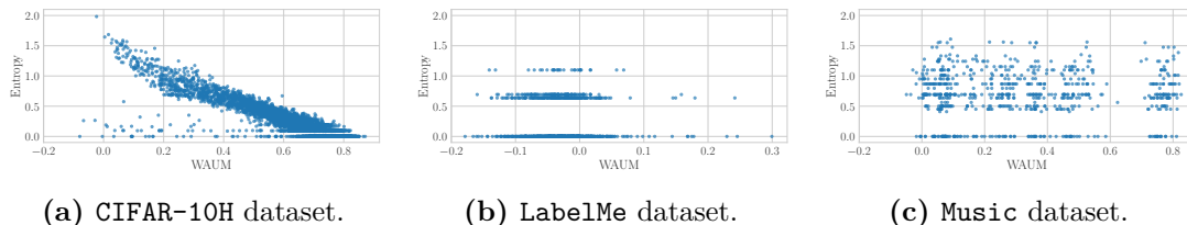
Figure 2.5 Entropy of votes vs. WAUM for CIFAR-10H, LabelMe, and Music, each point representing a task/image. When large amounts of votes per task are available, WAUM and entropy ranking coincide well, as in (a). Yet, when votes are scarce, as in (b) and (c), entropy becomes irrelevant while our introduced WAUM remains useful. Indeed, tasks with few votes can benefit from feedback obtained for a similar one. And for the LabelMe dataset in particular, there are only up to three votes available per task, thus only four different values of the entropy possible, making it irrelevant in such cases for modeling task difficulty.
