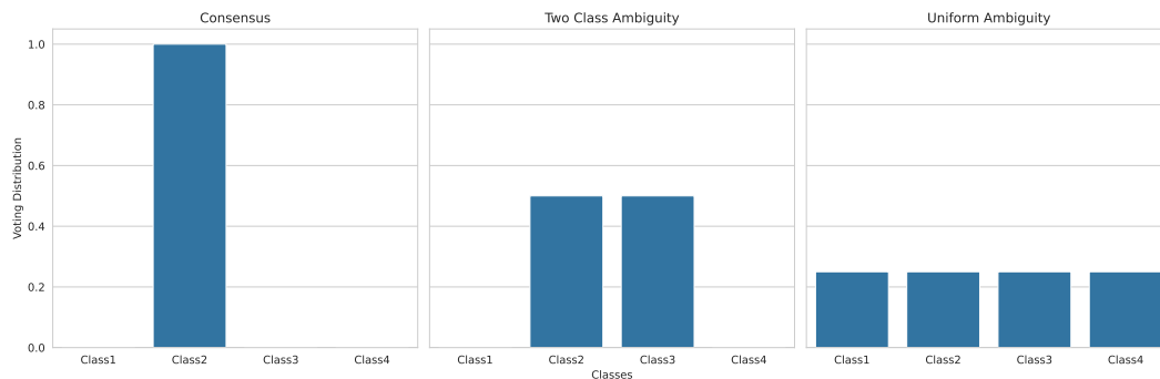
Figure 1.7 Three different configurations where the MV strategy can lead to the same label. When there is consensus there is no ambiguity to select the label. However, ambiguities can happen differently. There can be ambiguities between all classes or between a subset of classes.
