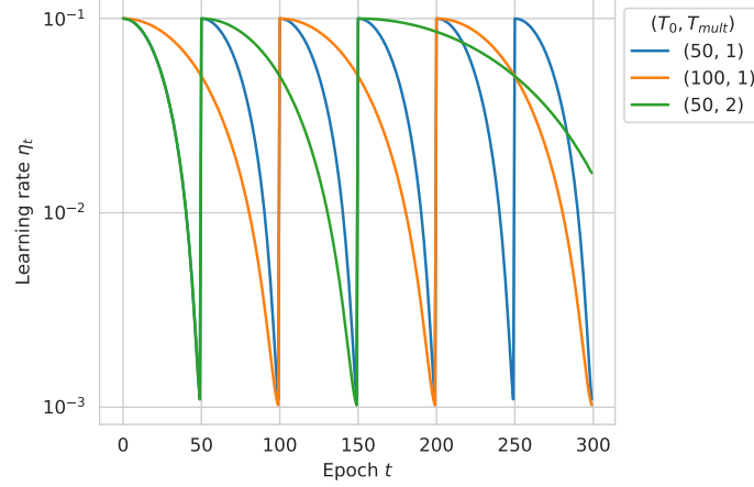
Figure 4.12 Learning rate schedule with a cosine annealing strategy with warm restarts. The learning rate at epoch t depends on the number of epochs in the initial cycle T_0 and the cycle length factor T_{mult} . The initial learning if \eta_{\max} = 0.1 and the minimal learning rate is \eta_{\min} = 10^{-3} .
