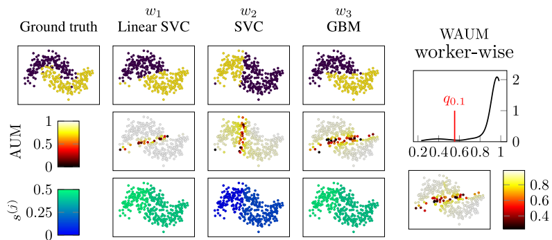
Figure 2.9 two_moons dataset: simulated workers with associated AUM and normalized trust scores. The hyperparameter \alpha is set to 0.1 for the worker-wise WAUM. Notice that the SVC classifier is mostly wrong (since we only train for one epoch for this worker), inducing a lower trust score overall.
