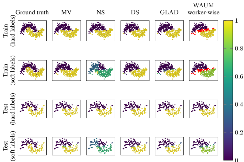
Figure 2.10 two_moons dataset: One realization of Table 2.2 varying the aggregation strategy. Label predictions on train/test sets provided by a three dense layers’ artificial neural network (30, 20, 20) trained on smooth labeled obtained after aggregating the crowdsourced labels (as in Figure 2.9). Points in red are pruned from the training set in the worker-wise WAUM aggregation. The \alpha hyperparameter is set to 0.1. Each point represents a task x_i , and its color is the probability of belonging in class 1. One can visualize the ambiguity in the soft training aggregated labels, but also in the resulting predictions by the neural network. Errors represented are standard deviations.
