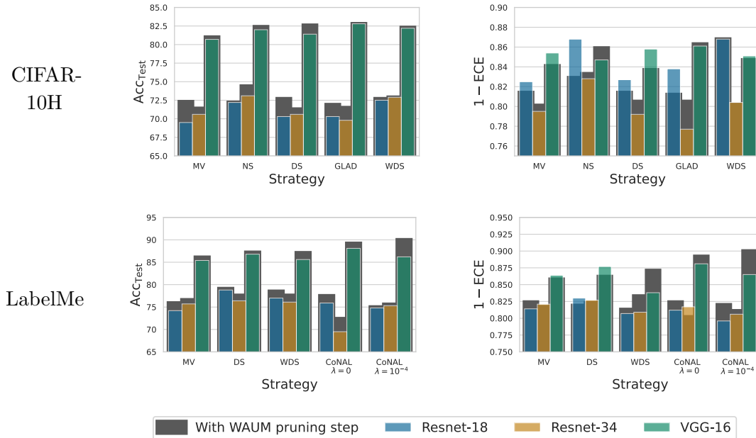
Figure 2.16 Performance obtained by training on the pruned dataset from the WAUM preprocessing step on CIFAR-10H and LabelMe. We consider multiple neural network architectures – ResNet-18, ResNet-34 or VGG-16 with batch normalization and two supplementary dense layers. We show that performance in accuracy is improved in most cases. Calibration performance in terms of ECE fluctuates depending on the architecture considered, especially for the CIFAR-10H dataset. Using the WAUM with CoNAL on the LabelMe dataset, we obtain the best performance both in accuracy and calibration.
