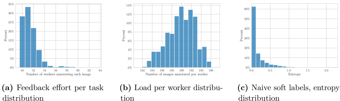
Figure 1.10 CIFAR-10H: dataset visualization
