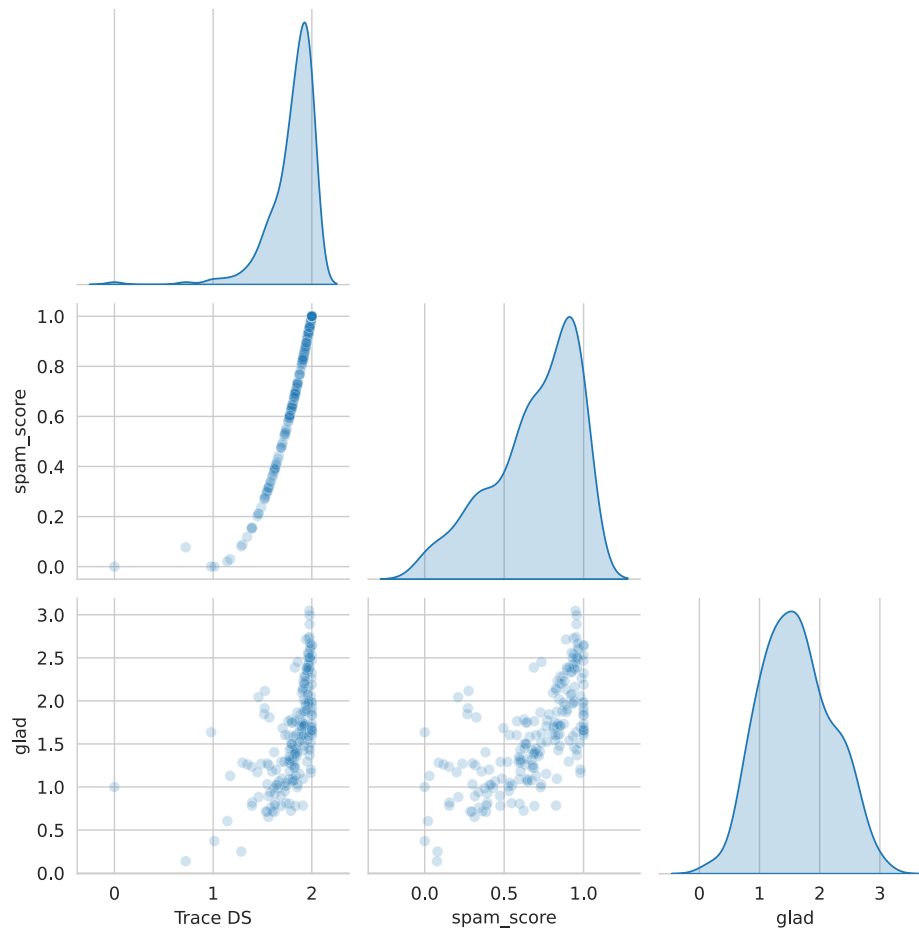
Figure 3.13 Comparison of ability scores by workers for the birds audio dataset. Most workers do seem to perform similarly, with very little noise voluntarily induced.
