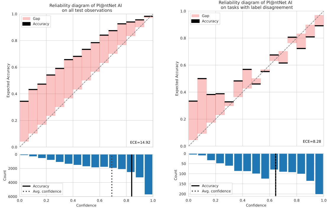
(a) Reliability diagram of Pl@ntNet AI on \mathcal{D}_{\text{expert}} (b) Reliability diagram of Pl@ntNet AI on \mathcal{D}_{\text{disagreement}}
