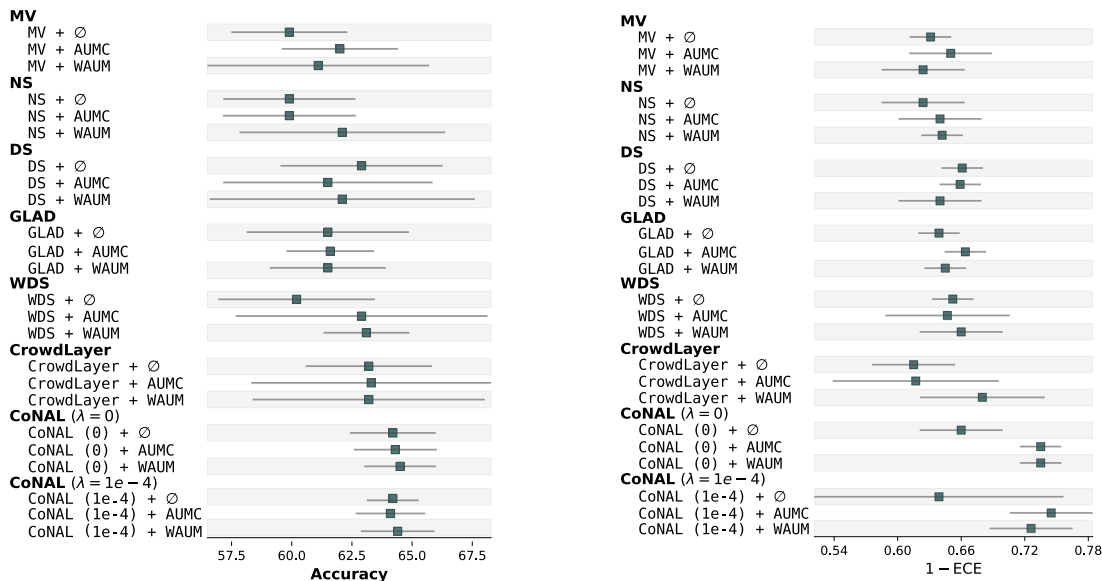
Figure 2.15 Ablation study on Music using the VGG backbone: \alpha = 0.05 . Errors are Gaussian confidence intervals at 95%.
