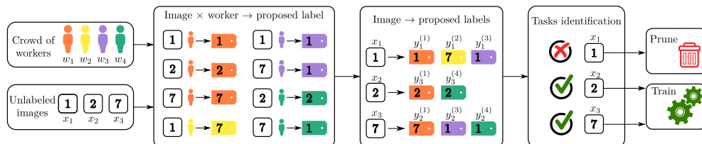
Figure 2.3 Learning with crowdsourcing labels: from label collection with a crowd to training on a pruned dataset. High ambiguity from either crowd workers or tasks intrinsic difficulty can lead to mislabeled data and harm generalization performance. To illustrate our notation, here the set of tasks annotated by worker w_3 is \mathcal{T}(w_3) = \{1, 3\} while the set of workers annotating task x_3 is \mathcal{A}(x_3) = \{1, 3, 4\} .
