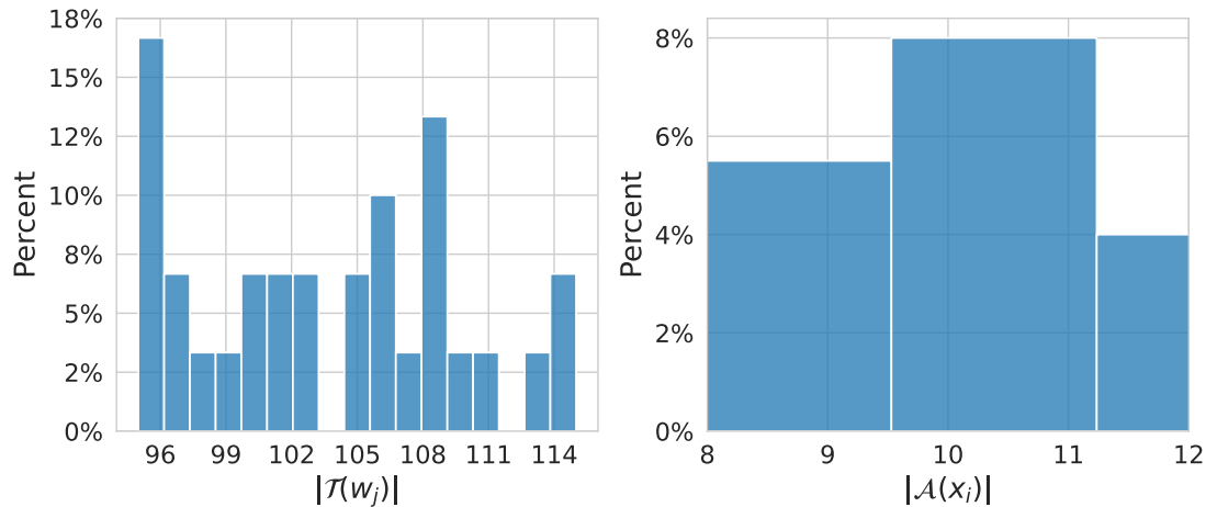
Figure 3.5 Distribution of the number of tasks given per worker (left) and the number of labels per task (right) in the independent mistakes setting with voting imbalance enabled.
