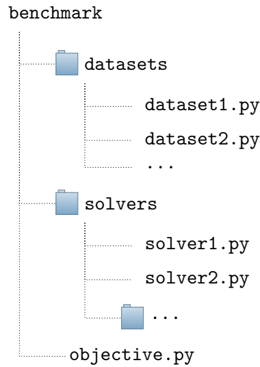
Figure 3.14 Template of a benchmark folder in Benchopt.
