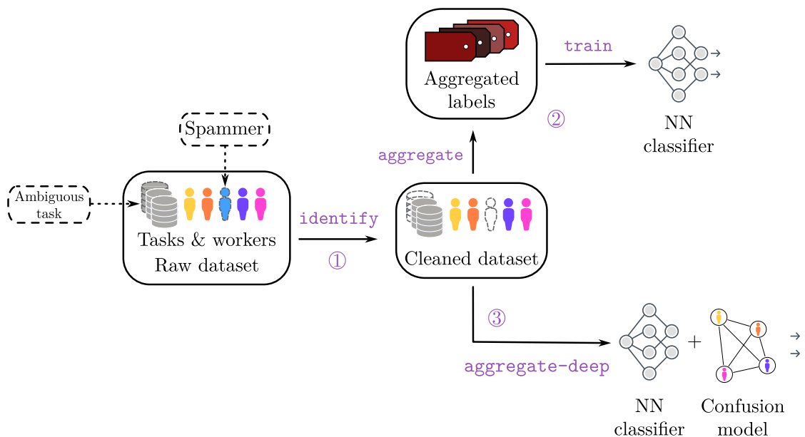
Figure 3.1 Pipeline on how to handle crowdsourced datasets with peerannot . After collecting the data, the identify module helps find poorly performing workers and/or ambiguous tasks. Those can be pruned to recover a cleaned set. Then, the aggregate module can be used to infer a label from multiple labels. The aggregate-deep module can be used to train a classifier from the crowdsourced labels without aggregation. Finally, the train module can be used to train a classifier from aggregated labels.
