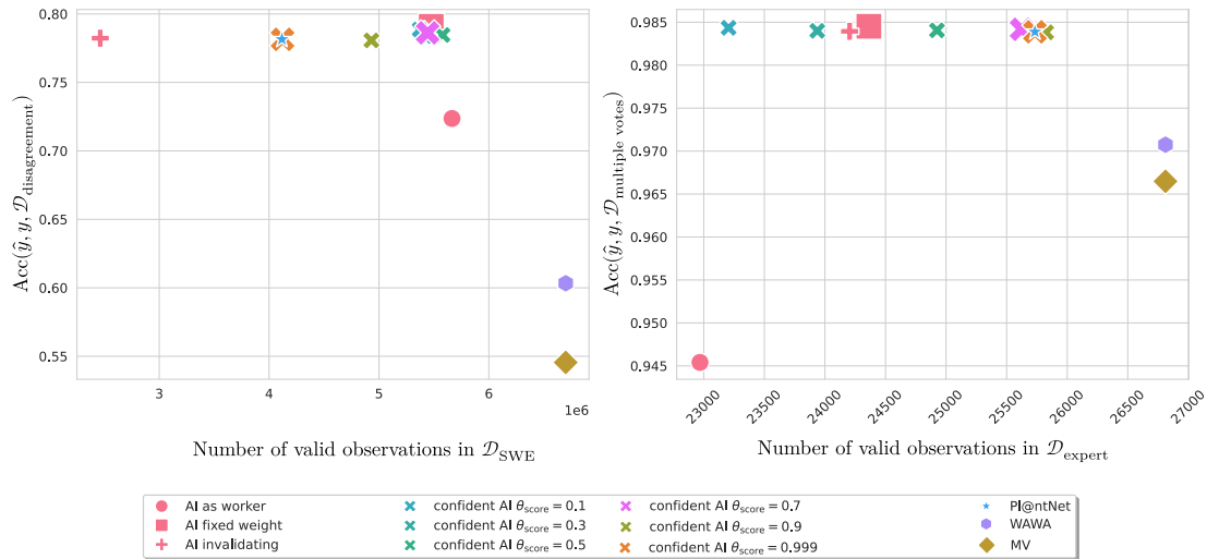
Figure 4.23 Performance in label recovery and number of observations marked as valid depending on how the AI vote is integrated. MV, WAWA and Pl@ntNet strategy without AI vote are used as reference. The best-performing strategy overall is confident AI with \theta_{score} = 0.7 . We also see that when \theta_{score} tends to 1, we recover the vanilla Pl@ntNet aggregation strategy.
