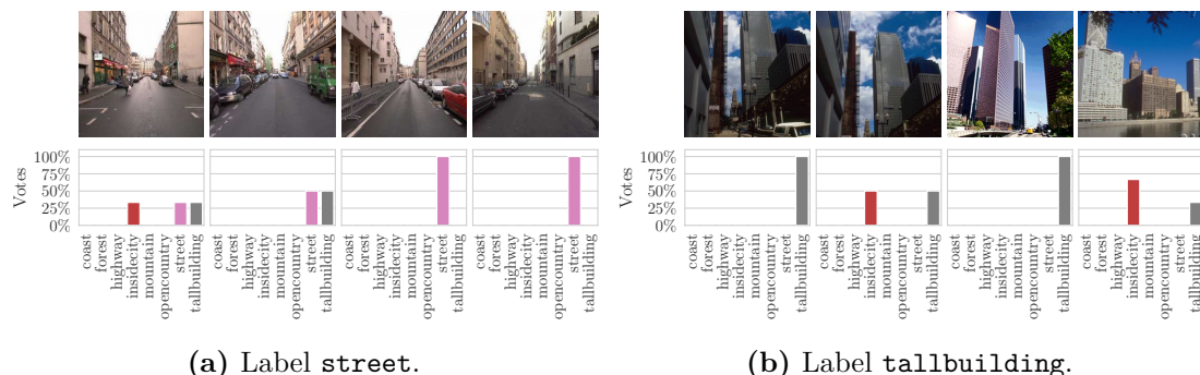
Figure 2.12 LabelMe dataset: Worst WAUM for classes (top) and the associated voting distribution for each image (bottom). (a) Label street (b) Label tallbuilding . Even if the two tasks are very similar, because the workers are different the associated proposed labels can differ and add noise during training.
