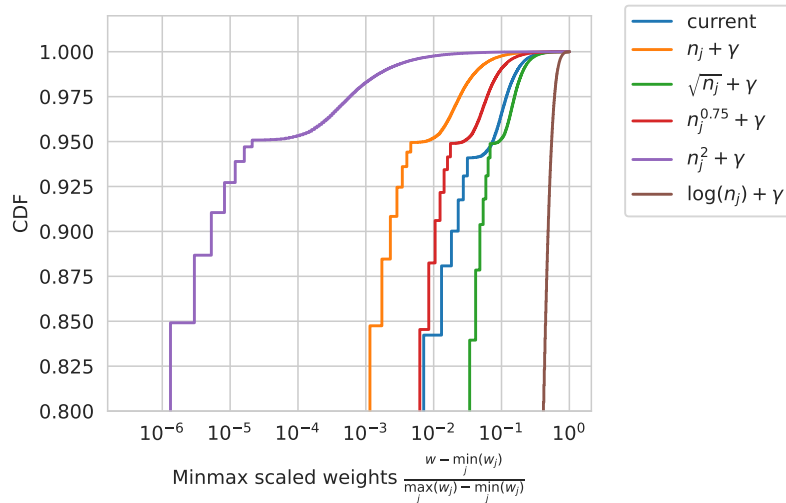
Figure 4.20 Zoomed empirical CDF of the weights obtained after running Pl@ntNet’s label aggregation strategy with the weight functions tested in Table 4.1. The log transformation result is represented for the sake of completeness.
