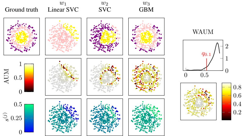
Figure 2.8 three_circles : one realization of simulated workers w_1, w_2, w_3 , with their AUM, normalized trust scores s^{(j)} (left) and WAUM distributions (right) for \alpha = 0.1 . Worker w_1 has less impact on the final WAUM in the disagreement area. Note also that for worker w_1 (LinearSVC), the region with low AUM values recovers the usual classifier’s margin around the decision boundary.
