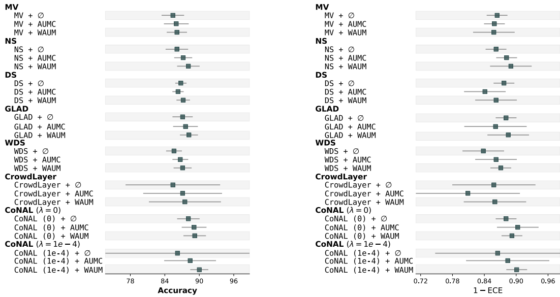
Figure 2.13 Ablation study on Labe1Me using the VGG backbone: \alpha = 0.01 . Errors are Gaussian confidence intervals at 95%.
