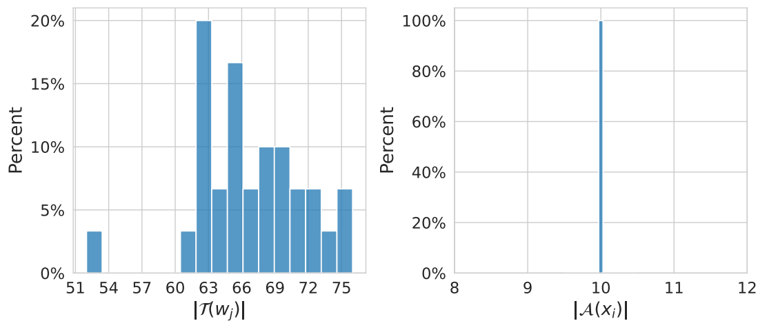
Figure 3.6 Distribution of the number of tasks given per worker (left) and the number of labels per task (right) in the correlated mistakes setting.
