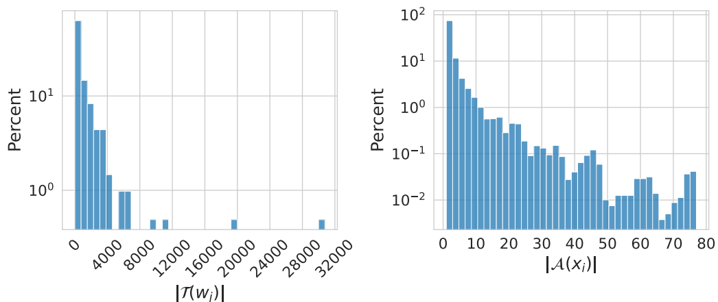
Figure 3.12 Distribution of the number of tasks given per worker (left) and of the number of labels per task (right) in the Audio Birds letters dataset.
