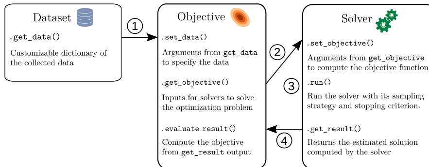
Figure 3.16 Dependency relation between datasets, solvers and objective objects. The three classes are the core of the Benchopt library and communicate to run the optimization problem and monitor the performance on multiple datasets. First, the data from Datasets are passed to the Objective class. Then, the objective communicates this data for the solver to be instantiated and run. Finally, the solver returns the sequence of parameters \{\theta_k\}_k to the objective to compute the performance metrics.
