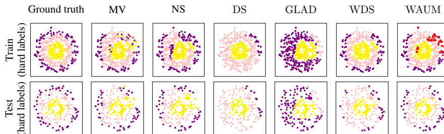
Figure 2.6 three_circles : One realization of Table 2.1 varying the aggregation strategy. Training labels are provided from Figure 2.8 and predictions on the test set are from three dense layers’ artificial neural network (30, 20, 20) trained on the aggregated soft labels. For ease of visualization, the color displayed for each task represents the most likely class. Red points are pruned from training by WAUM with threshold \alpha = 0.1 . Here, we have n_{\text{task}} = 525 . WAUM method as in Table 2.1 uses WDS labels.
