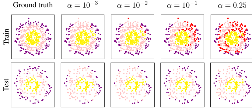
Figure 2.7 Influence of \alpha on the pruning step. Red dots indicate data points pruned from the training set, at level q_\alpha in the WAUM (see line 10 in Algorithm 4). We consider ( \alpha \in \{10^{-3}, 10^{-2}, 10^{-1}, 0.25\} ). The neural network used for predictions is three dense layers (30, 20, 20), as for other simulated experiments. Training labels are from the WDS + WAUM strategy with performance reported in Table 2.1. The more we prune data, the worse the neural network can learn from the training dataset. However, removing the tasks with high disagreement noise helps to generalize.
