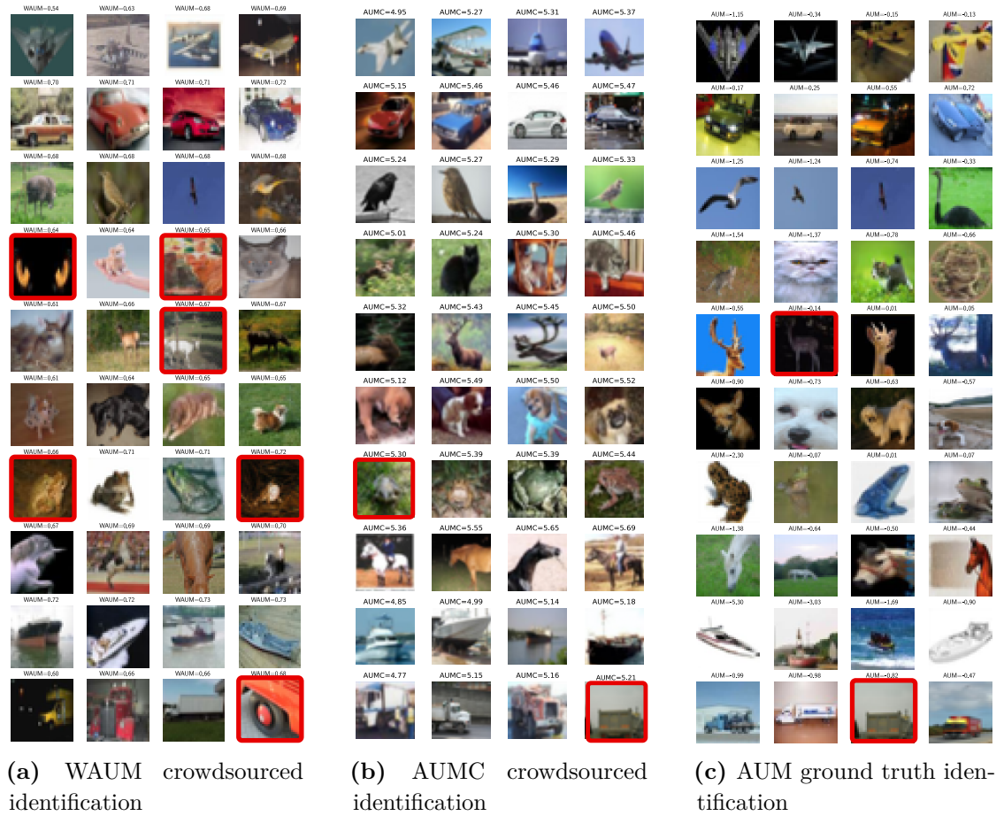
Figure 2.17 Comparison of the worse images detected by the WAUM, AUMC and classical AUM preprocessing step. Identification was computed with a ResNet-18 for 50 epochs using the parameters described in Section 1.2.5. Each row represents the class given by the unobserved ground truth label from the CIFAR-10 dataset. Only the AUM uses the ground truth label, other methods are based on the crowdsourced labels only. Images framed in red can be hard to classify.
