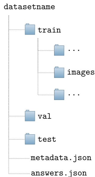
Figure 3.2 Template of a dataset folder in peerannot . Collected votes are in answers.json , all necessary information on the dataset are in metadata.json . Tasks are either in the train , val or test folders. test tasks are assumed to have an associated ground truth label.
