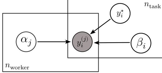
Figure 1.9 Bayesian plate diagram representation of the GLAD model. Only the labels \{y_i^{(j)}\}_{i,j} are observed. Latent variables to estimate are the true labels (y_i^*)_i . Parameters are the worker ability \alpha_j and the task difficulty \beta_i . The underlying task features (x_i)_i are not considered.
