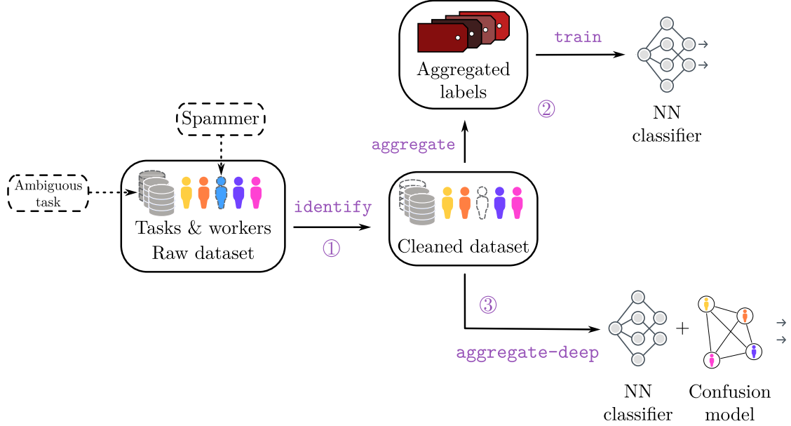
Figure 1.6 pipeline of crowdsourcing experiments. The data is collected. We identify poorly performing workers and/or ambiguous tasks. Then labels are aggregated to be used in a supervised learning setting. If the tasks are available and the goal is to learn a predictor, deep-learning-based strategies can be used to learn the confusion model and the classifier at the same time.
