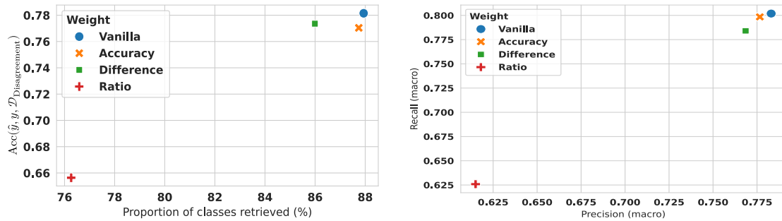
(a) Accuracy on \mathcal{D}_{\text{disagreement}} w.r.t. to the proportion of classes retrieved
