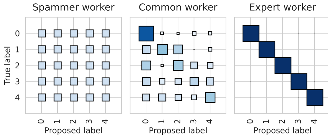
Figure 3.7 Three types of profiles of worker confusion matrices simulated with peerannot . The spammer answers independently of the true label. Expert workers identify classes without mistakes. In practice common workers are good for some classes but might confuse two (or more) labels. All workers are simulated using the peerannot simulate command.
