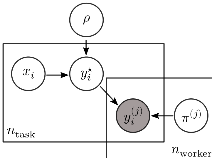
Figure 1.8 Bayesian plate diagram representation of the DS model. Only the labels \{y_i^{(j)}\}_{i,j} are observed. Latent variables to estimate are the true labels (y_i^*)_i . Parameters are the prevalence \rho of each class and the confusion matrices \{\pi^{(j)}\}_j for each worker. The underlying task features (x_i)_i are not considered.
