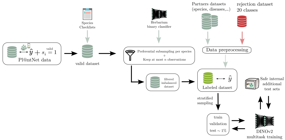
Figure 4.11 Pl@ntNet pipeline: the steps to train a neural network from the collaboratively annotated data. The algorithm presented in Section 4.2 is used to get labels and a validity indicator. Subsampling and data from partners are then combined to get a labeled dataset to train the current DINOv2 model. Evaluation is performed on the generated test set and additional private test sets.
