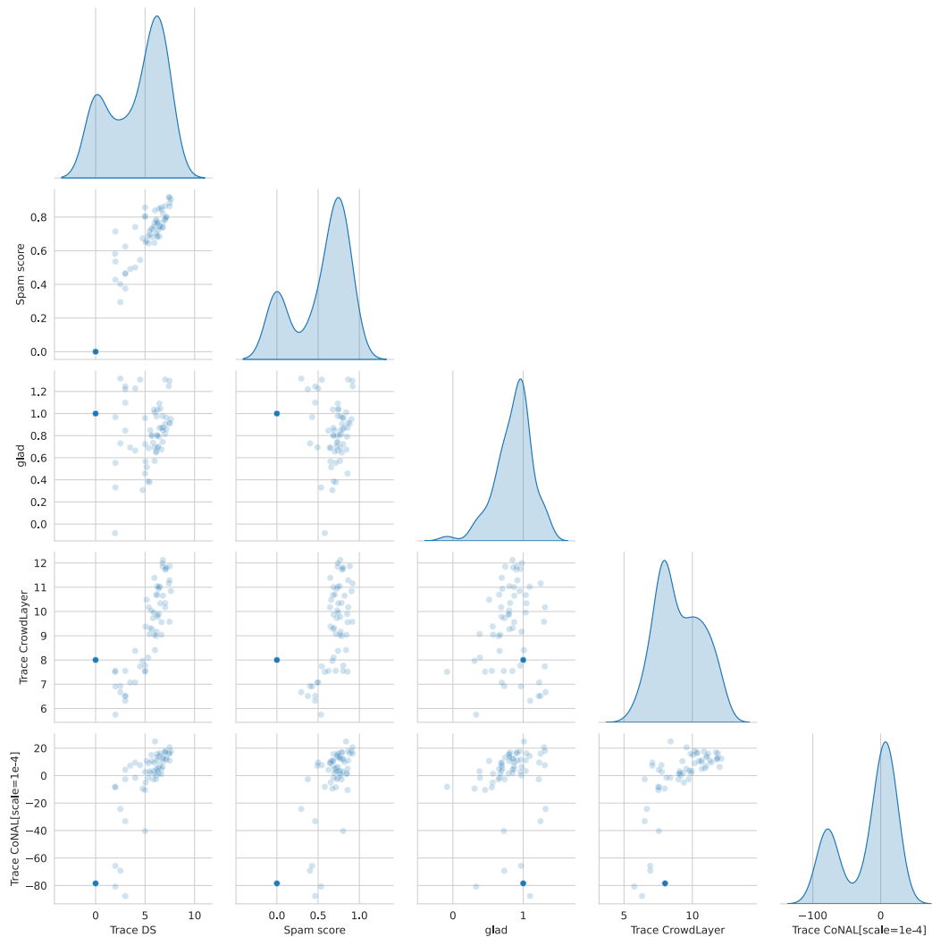
Figure 3.11 With few labels per task, workers are more difficult to rank. It is more difficult to separate workers with their abilities in this crowd. Hence the importance of investigating the generalization performance of the methods presented in the previous section.
