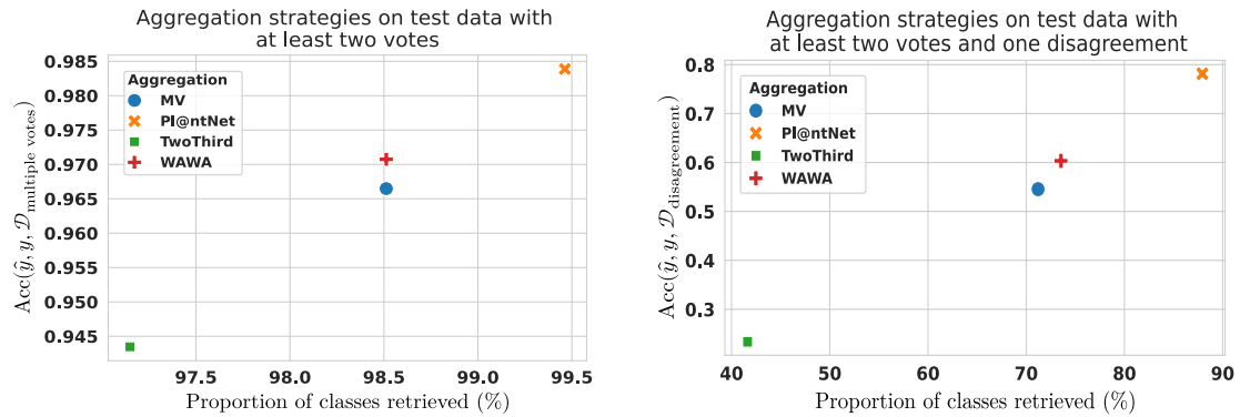
(a) Accuracy on \mathcal{D}_{\text{multiple votes}} w.r.t. to the proportion of classes recovered
