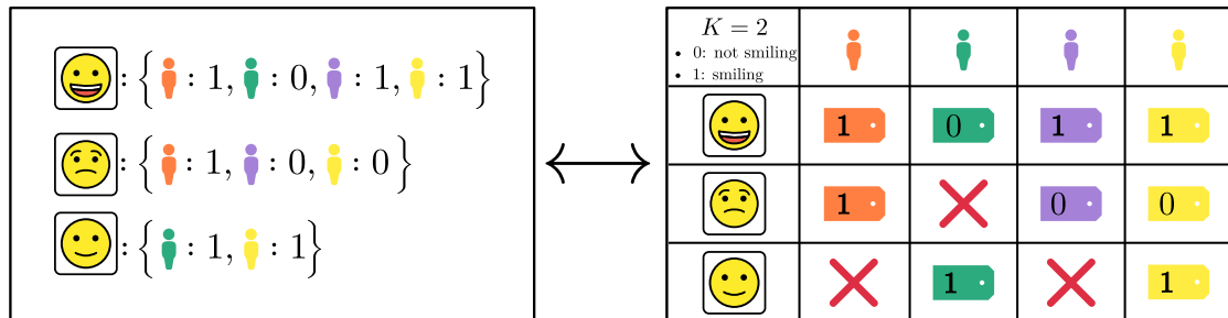
Figure 3.3 Data storage for the toy-data crowdsourced dataset, a binary classification problem ( K = 2 , smiling/not smiling) on recognizing smiling emoticons. On the left how peerannot stores the data, and on the right the raw data.
