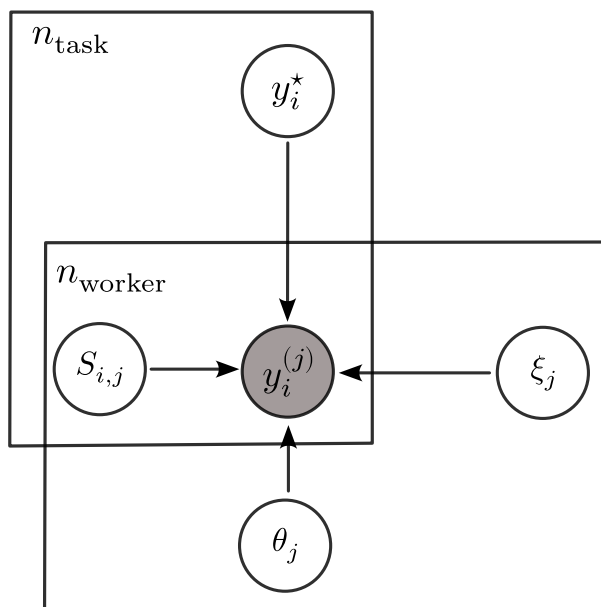
Figure 3.19 Bayesian plate diagram representation of the MACE model. Only the labels \{y_i^{(j)}\}_{i,j} are observed. Latent variables to estimate are the true labels ( y_i^* ), the spamming state ( S_{i,j} ) _{i,j} , the probability to spam ( \theta_j ) _j and the worker behavior when spamming ( \xi_j ) _j .
