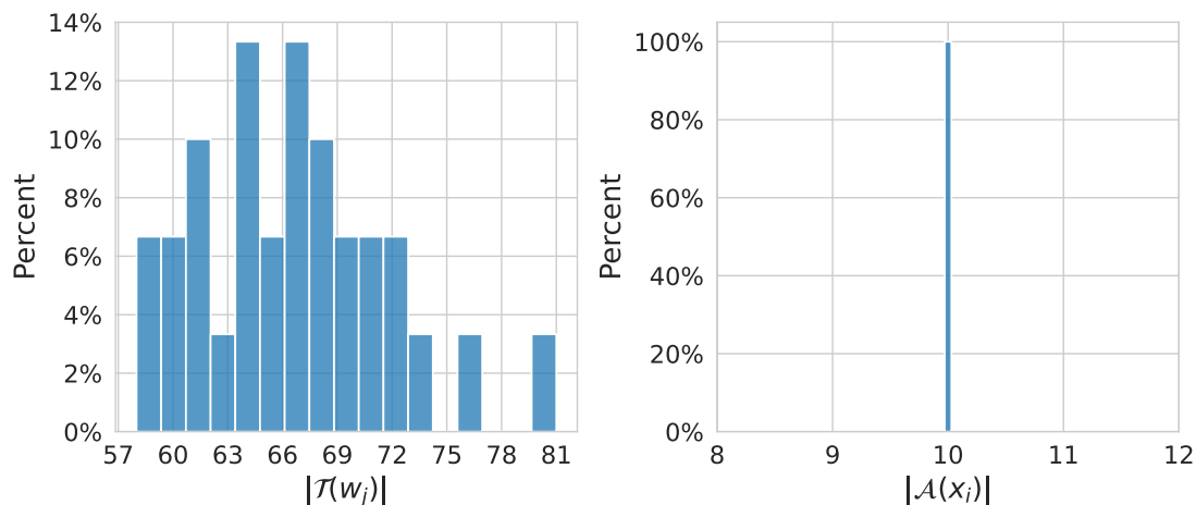
Figure 3.4 Distribution of the number of tasks given per worker (left) and number of labels per task (right) in the independent mistakes setting.
