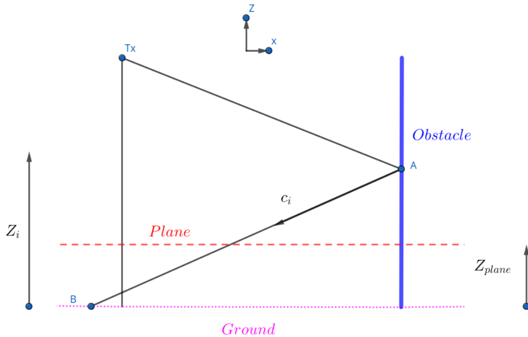
Figure 4.2: Ray-Plane intersection
