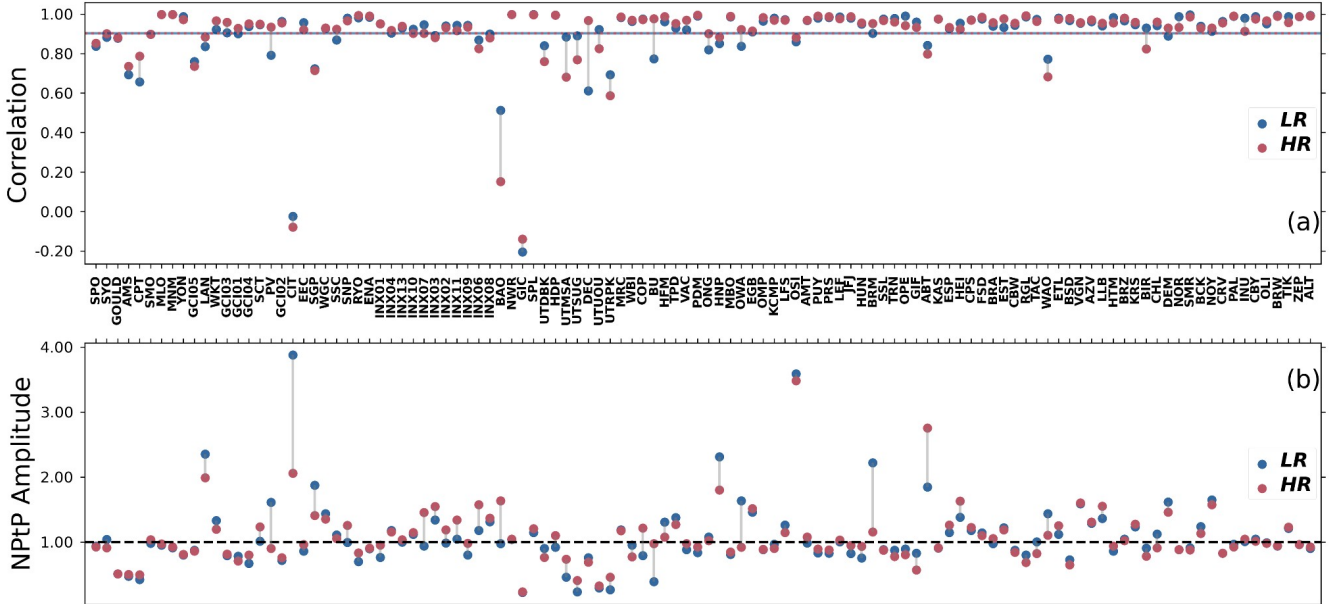
Figure 2. Pearson correlation coefficient (a) and average normalized peak-to-peak amplitude (b) of the modeled vs. measured CO 2 mole fraction seasonal cycle for each surface station studied for the years 2015-2016. Blue circles are for the LR model and red circles are for the HR model. The stations are represented by their code in the ObsPack database. The average correlation coefficient for each resolution is in the corresponding color as a solid or dotted line in panel (a). The black dashed line in (b) corresponds to the ideal normalized peak-to-peak amplitude of 1. The stations are ordered on the abscissa by increasing latitude from -90° to +90°.
