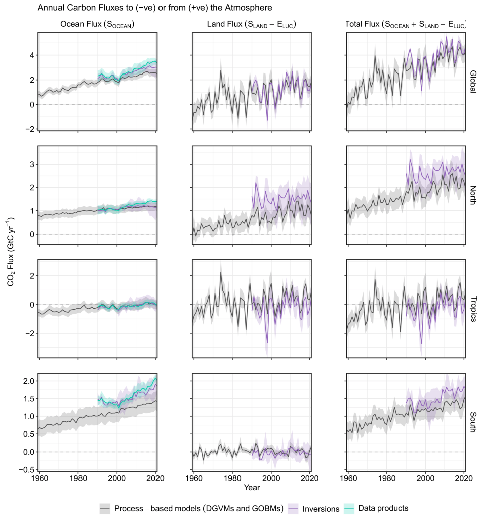
Figure II.2: CO 2 fluxes between the atmosphere and the Earth’s surface separated between land and oceans globally and in three latitude bands. The ocean flux is S_{\text{OCEAN}} , and the land flux is the net of atmosphere–land fluxes from the DGVMs. The latitude bands are (top row) global, (second row) north ( > 30^\circ \text{ N} ), (third row) tropics ( 30^\circ \text{ S} – 30^\circ \text{ N} ), and (bottom row) south ( < 30^\circ \text{ S} ), showing values over ocean (left column) and land (middle column) and in total (right column). Estimates are shown for process-based models, inversion systems, and f\text{CO}_2 -based data products (Friedlingstein et al., 2022).
