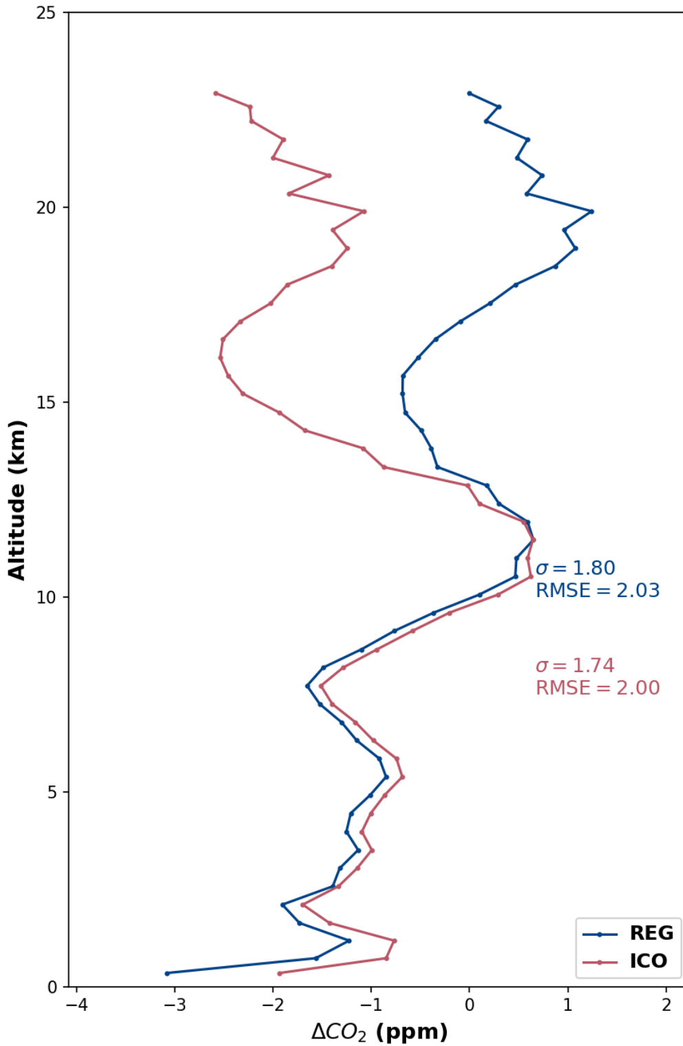
Figure 13: Difference in \text{CO}_2 mole fraction vertical profile between the two model configurations of the model and AirCore measurements. The blue line represents the difference between the REG model output and measurements, while the red line indicates the difference between the ICO model output and measurements. The fitted lines were generated by averaging the data over 50 altitude bins.
