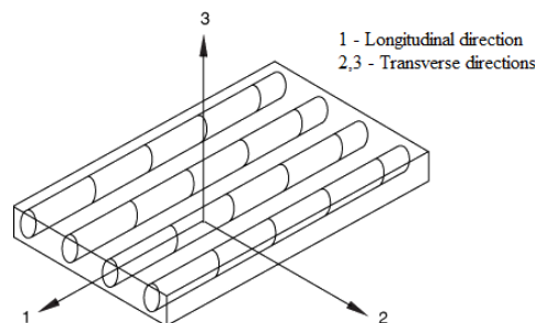
Fig. 1.11. Unidirectional ply axis system
