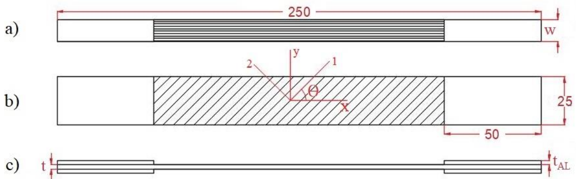
Fig. 3.3. Samples dimensions in mm; a) 0^\circ tensile test b) off-axis and transverse tensile test c) side view of samples; all dimensions are in mm, w – width of the sample, t – thickness of the sample, t_{AL} – thickness of aluminum tabs
