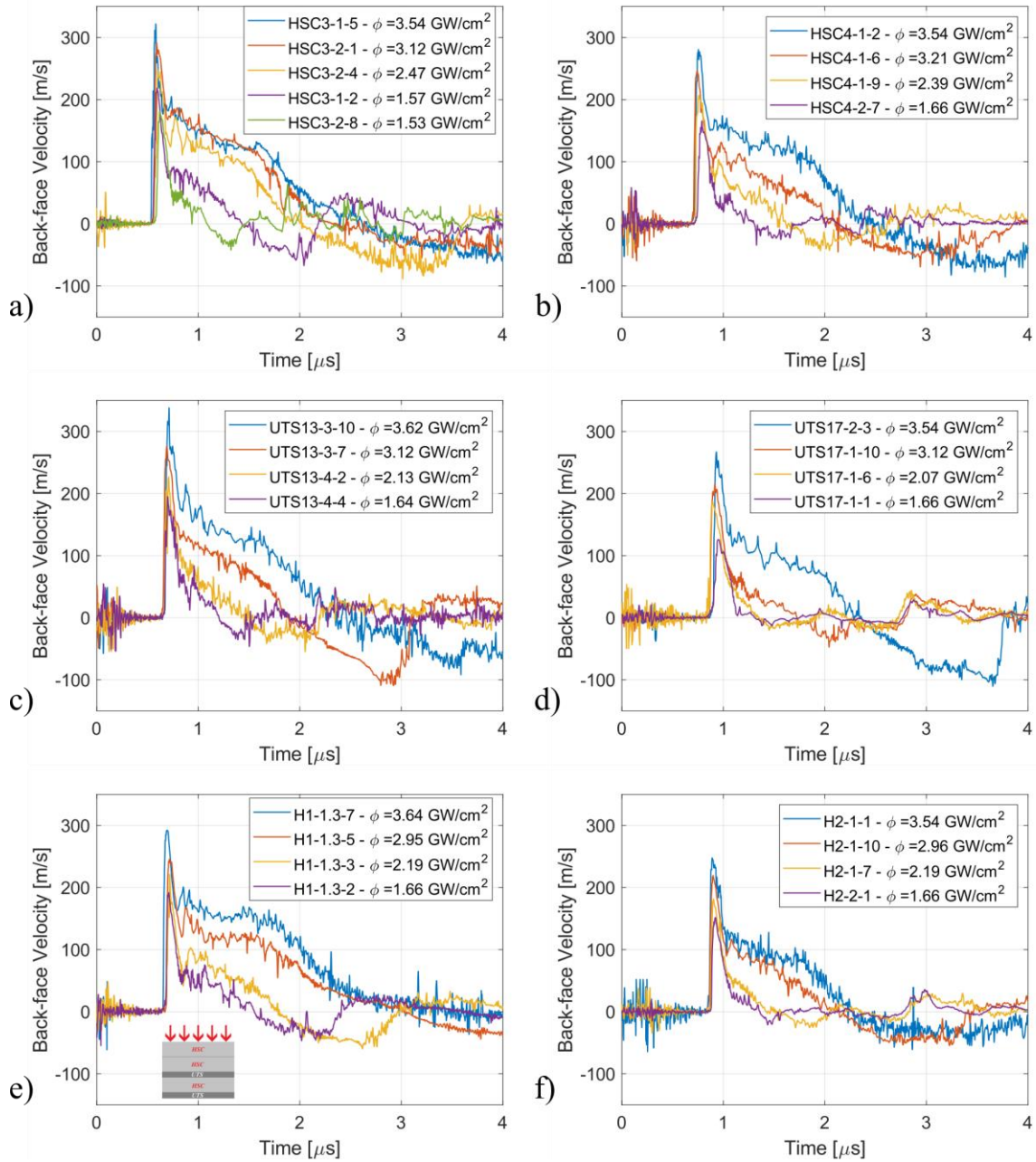
Fig. 4.38. Representative back-face velocity versus time signals for all tested materials, at different energy levels, with the corresponding density of power; a) HSC3; b) HSC4; c) UTS13; d) UTS17; e) H1 (2022 experimental campaign); f) H2
