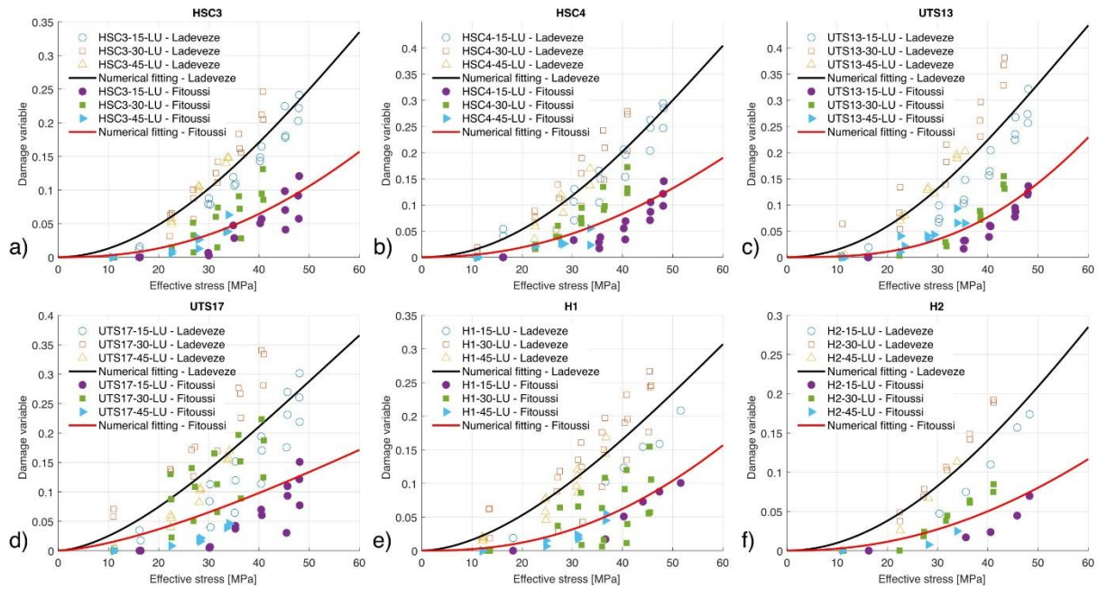
Fig. 3.37. Damage variable at 15°, 30°, and 45° off-axis angle - effective stress curves with numerical fitting, a_2=0.2 and b_2=0.05 ; a) HSC3; b) HSC4; c) UTS13; d) UTS17; e) H1; f) H2
