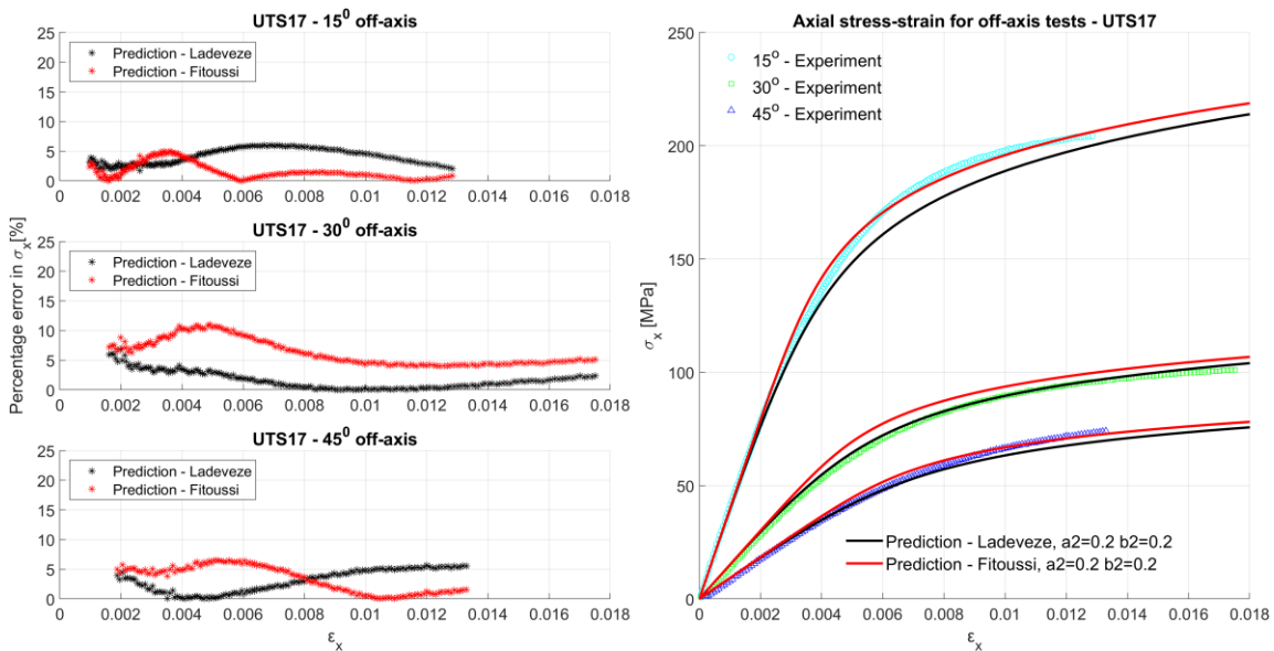
Fig. 3.51. Prediction for UTS17 using damage-plasticity parameters estimated from UTS13 data, a_2=0.2 and b_2=0.2 – with corresponding \sigma_x percentage error between predicted values and experimental results
