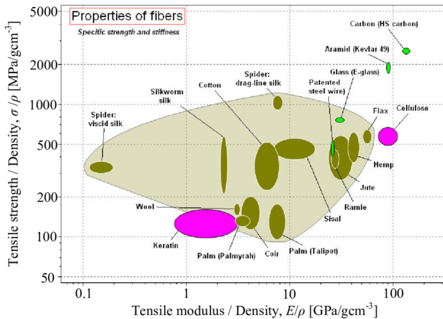
Fig. 1.1. Specific strength and stiffness of natural and synthetic fibers [33]
