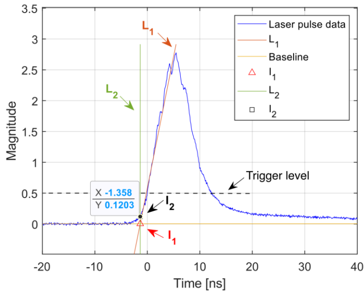
Fig. 4.5. Analysis of laser pulse data to extract required time shift
