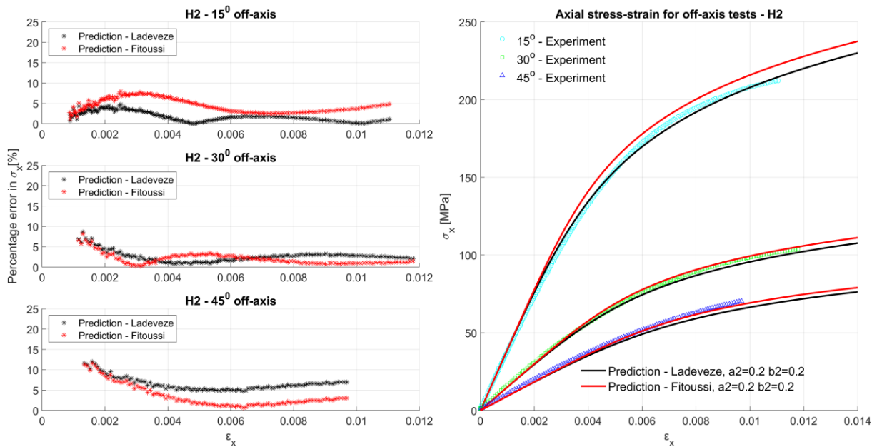
Fig. 3.54. Prediction for H2 using damage parameters from H2 data and plasticity parameters estimated from HSC4 data, a_2=0.2 and b_2=0.2 – with corresponding \sigma_x percentage error between predicted values and experimental results
