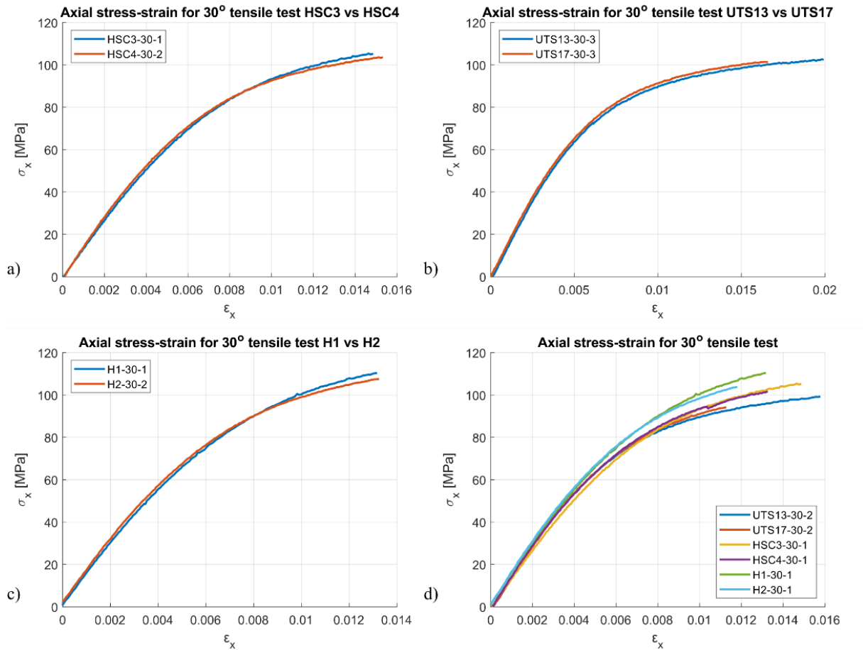
Fig. 3.16. Comparison of axial stress-strain response under 30° off-axis tensile test at 1 mm/min from DIC analysis, for representative samples of each laminate configuration; a) HSC3 vs HSC4; b) UTS13 vs UTS17; c) H1 vs H2; d) Simple and hybrid configuration materials
