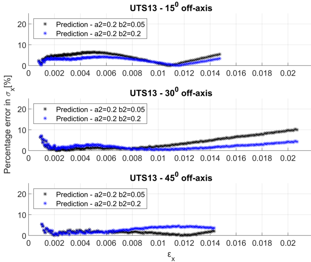
Fig. H. 3. Prediction percentage error comparison for UTS13, using a_2=0.2 ; b_2=0.05 or b_2=0.2
