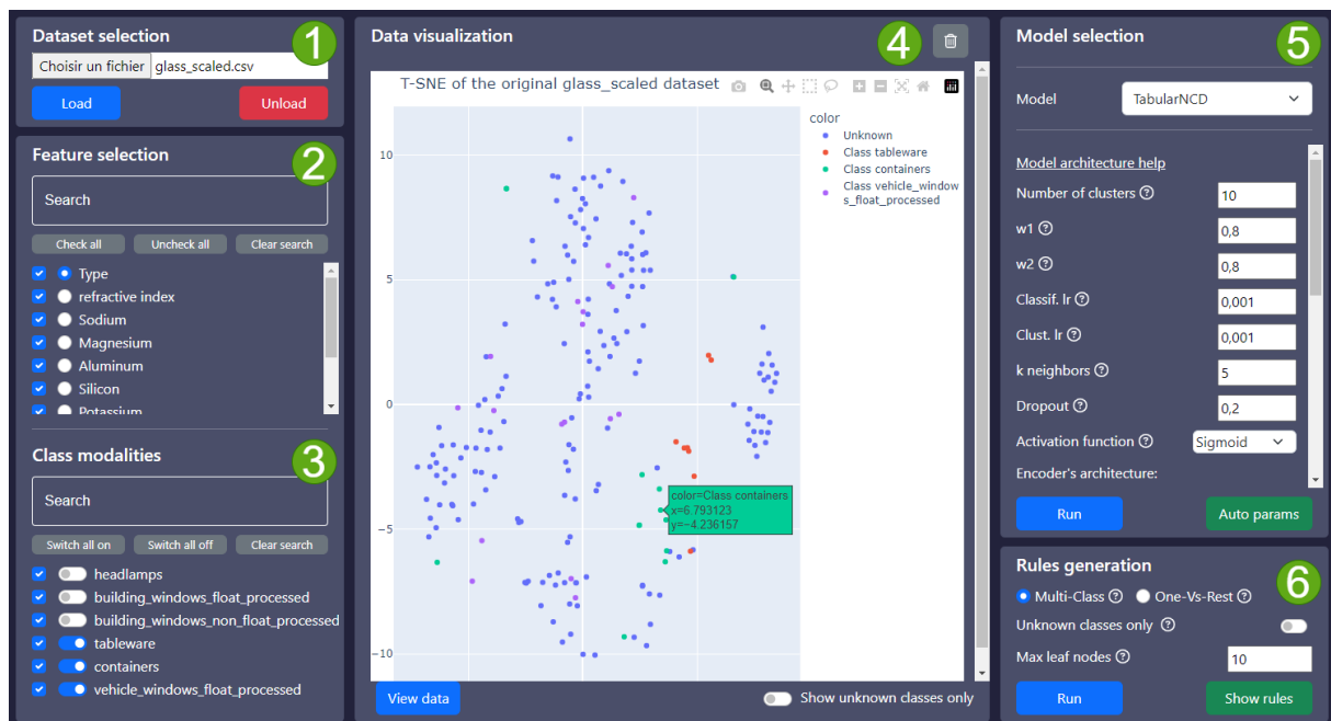
Figure 5.1 – The interface for interactive clustering and Novel Class Discovery.
