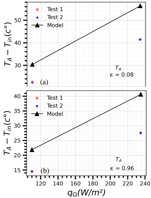
Figure 6.7: Validation of the results predicted by the SHBM for (a) Temperature difference between active wall mean and inlet air at low emissive walls (b) Temperature difference between active wall and inlet air at high emissive walls
