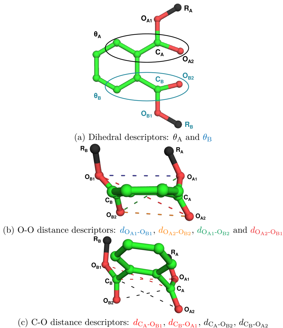
Figure 3.2: Structural descriptors: (a) dihedral angles and (b)-(c) interatomic distances. Carbon atoms are in green and oxygen atoms are in red. R balls in black represent the terminal group of each side chain.
