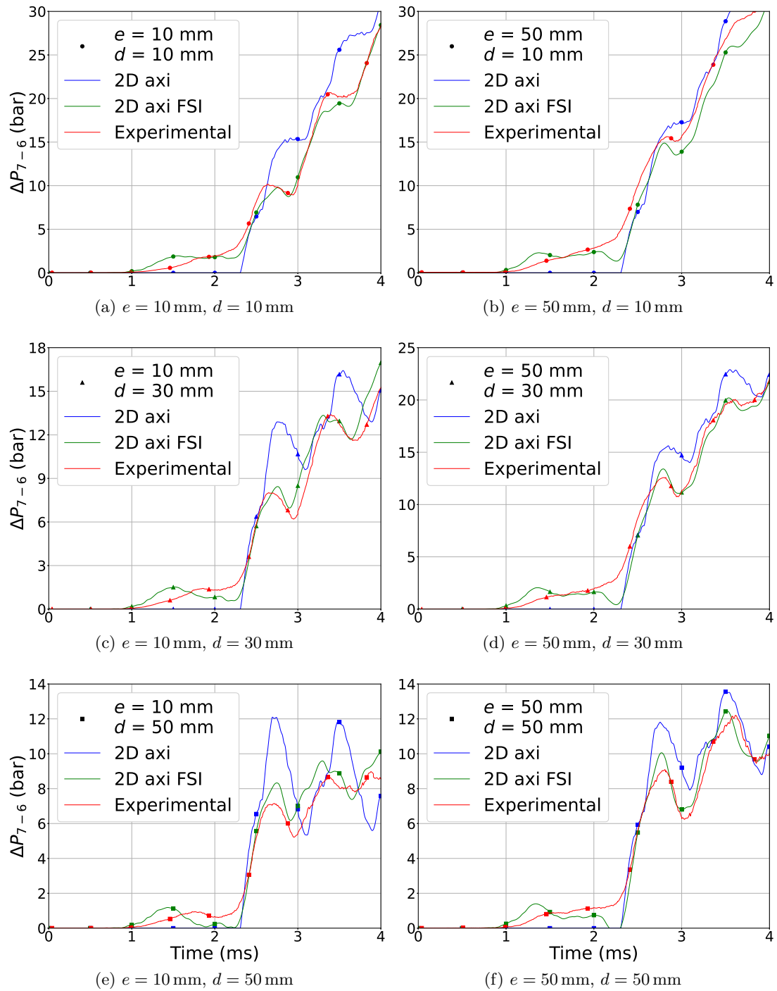
Figure 4.21: Pressure difference between sensors C6 and C7, \Delta P_{7-6} , for all orifice plates. Focus on 0 < t < 4 \text{ ms} .
