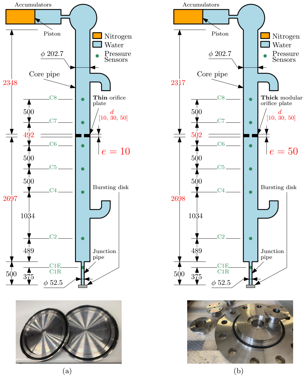
Figure 2.4: Experimental set-up (all dimensions in millimeters): (a) thin orifice plates, (b) thick modular orifice plate.
