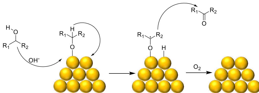
Scheme 1.3. Mechanism of aerobic oxidation of alcohols over Pd NPs
