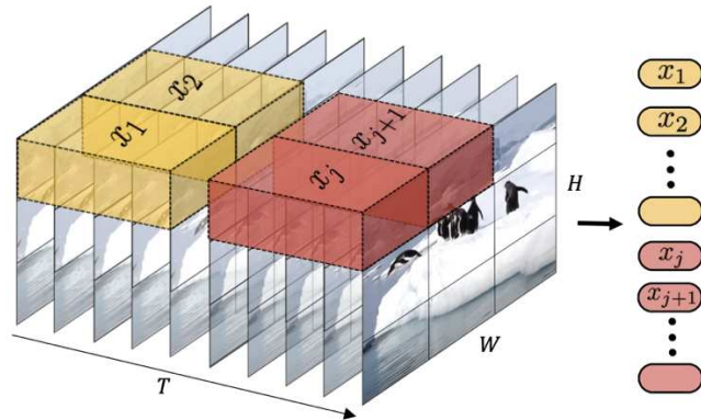
Figure 52. Illustration of input data embedding. This figure shows the input data embedding for the video vision-transformer. The operation is not only for the spatial dimensions, but also for the temporal dimensions. Image from (Arnab et al. , 2021)
