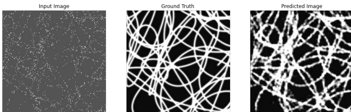
Figure 53. Preliminary result for video vision transformer architecture. This figure displays the first frame of the movie for the input data (left panel), the ground truth (the middle panel) and the model’s prediction (right panel).
