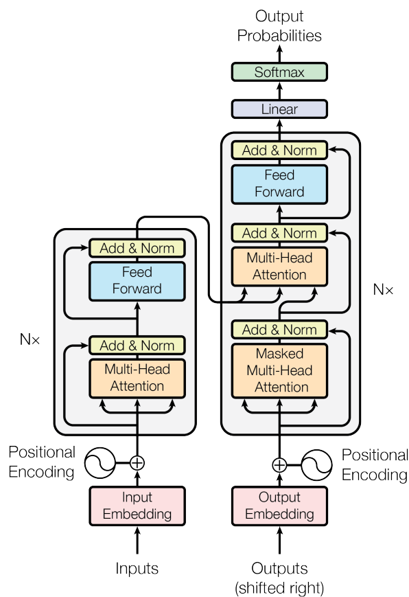
Figure 23. The architecture of Transformer. Image from (Vaswani et al. , 2017).
