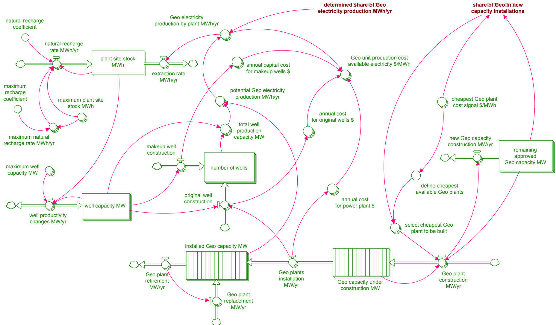
Fig.2: Simplified structure of geothermal resource dynamics model (green) and its connection to UniSyD_IS (red)
