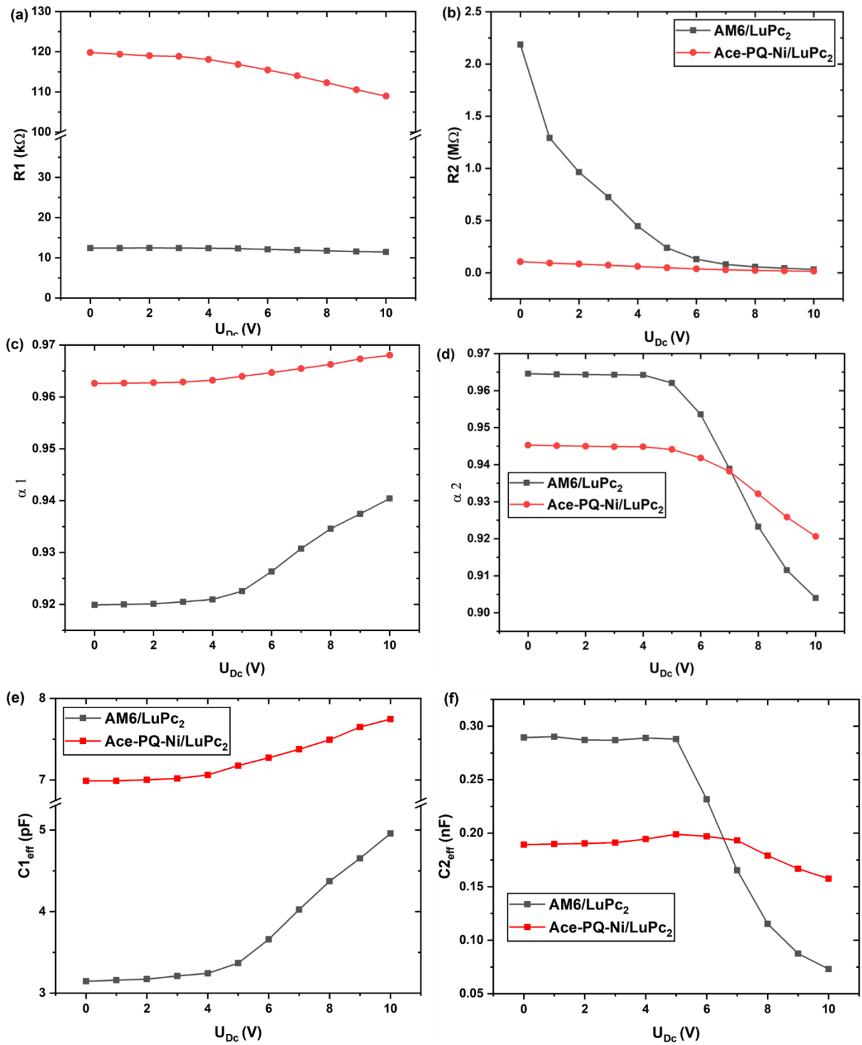
Figure 21. Variations of equivalent circuit resistances, R1 (a) and R2 (b), \alpha 1 (c) and \alpha 2 (d), effective capacitances C_{\text{eff1}} (e) and C_{\text{eff2}} (f), as a function of bias (0-10 V) for Ace-PQ-Ni/LuPc 2 and AM6/LuPc 2 heterojunction devices.
