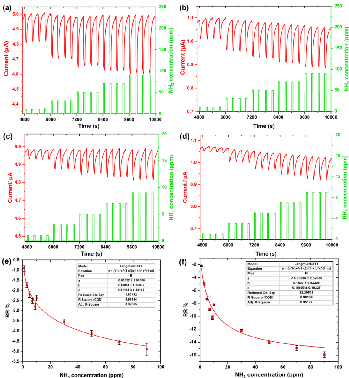
Figure 23. Response of Ace-PQ-Ni /LuPc 2 (a and c) and AM6/LuPc 2 (b and d) heterojunction sensors under NH 3 gas for 1 min and recovery under clean air for 4 min in the range of NH 3 concentration from 1 to 90 ppm at 45% of RH and room temperature (18–21 °C). The variation of relative response (calibration curve) of Ace-PQ-Ni /LuPc 2 (e) and AM6/LuPc 2 (f) as a function of NH 3 concentration.
