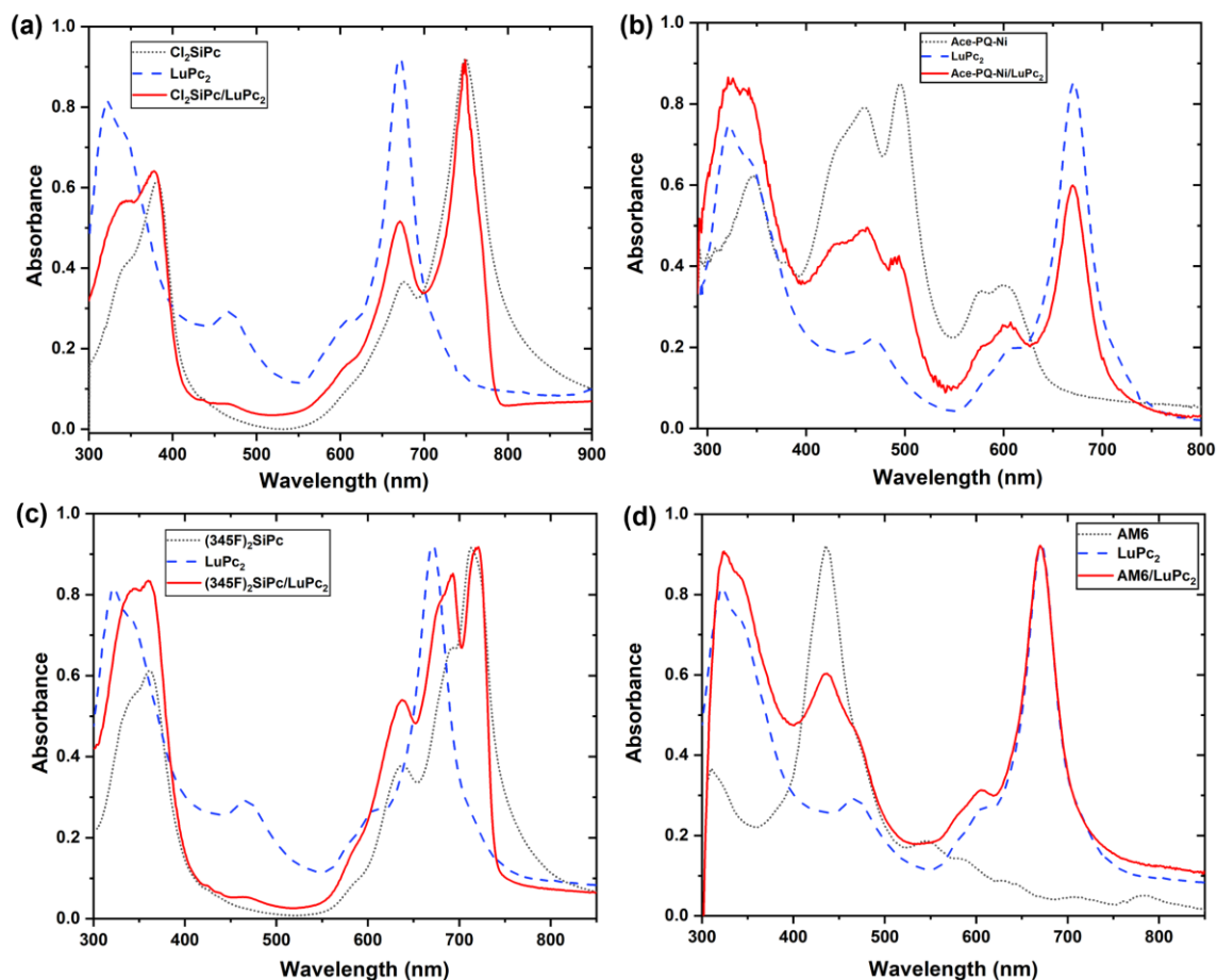
Figure 7. Absorption spectrum of Cl 2 SiPc/LuPc 2 (a), (345F) 2 -SiPc/LuPc 2 (c), Ace-PQ-Ni/LuPc 2 (b), and AM6/LuPc 2 (d) bilayer heterostructure films (red line) compared to the spectra of their corresponding sublayer (black dotted line) and top layer (LuPc 2 ) (blue dash line) in THF solutions.
