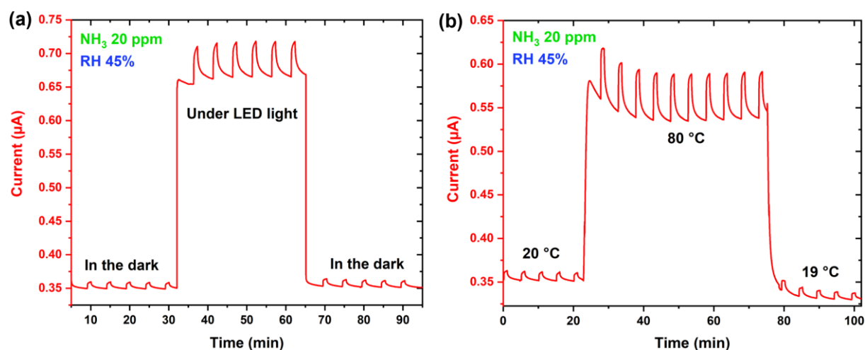
Figure 45. Response curve of VOF 8 Pc/LuPc 2 heterojunction sensor, under successive exposures to 20 ppm NH 3 under different conditions: in the dark and under light (a), as well as in room temperature and 80 °C (b) at 45% RH.
