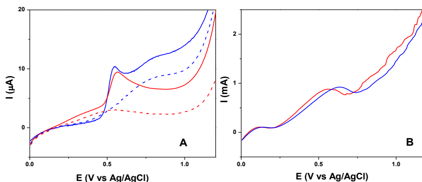
Figure 4.3. Linear sweep voltammograms at Pt electrode at 0.1 \text{ V s}^{-1} from 0 V to 1.2 V in 0.2 M PBS pH 8 with 50 mM \text{KNO}_3 (red) and \text{KCl} (blue) ( A ) containing 0 mM L-012 (dashed lines) and 0.42 mM L-012 (solid lines) and ( B ) containing 0.42 mM L-012 and 0.5 M \text{H}_2\text{O}_2 .
