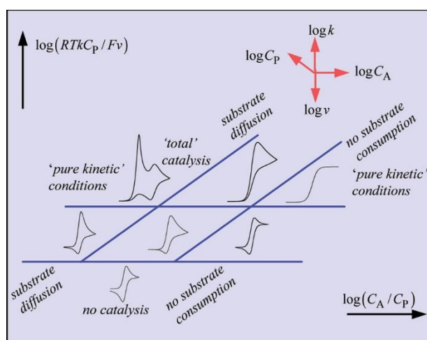
Figure 2.3. Kinetic zone diagram illustrating the characteristic CV response shapes for a catalytic reaction, first-order in both substrate and catalyst, as a function of two dimensionless parameters. Reproduced from 52 .
