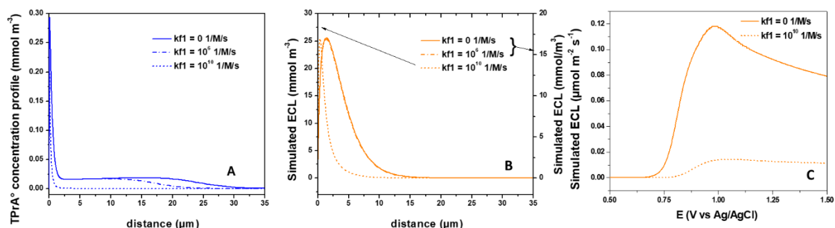
Figure 2.9. Simulated: (A) concentration profiles of TPrA radical; (B) thickness of the ECL generated photon concentration profiles (at 620 nm) layer in 500 nM [Ru(bpy) 3 ] 2+ , 1 mM [Ir(sppy) 3 ] 3- and 10 mM TPrA at different rates of homogenous reduction of [Ir(sppy) 3 ] 3- (reaction 7.1), with rate constant k_{f1} = 0 (solid line), 10^6 (dashed line, and 10^{10} \text{ M}^{-1}\text{s}^{-1} (dotted line). (C) Simulated ECL intensities at 620 nm, I_{\text{ECL,Ru}} in 500 nM [Ru(bpy) 3 ] 2+ , 1 mM [Ir(sppy) 3 ] 3- and 10 mM TPrA when homogenous reduction of [Ir(sppy) 3 ] 3- (reaction 2.14) is not included (solid line), and is diffusion-controlled, k_{f1} = 10^{10} \text{ M}^{-1}\text{s}^{-1} (dotted line).
