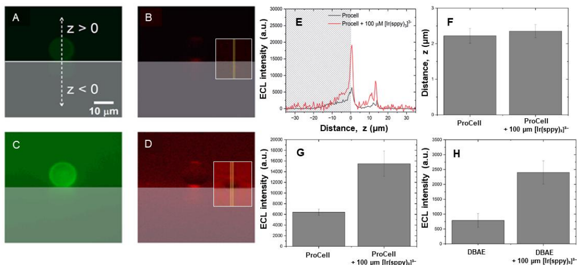
Figure 3.6. Side-view micrographs of 12 μm Ru@PS beads in (A) and (C) photoluminescence (PL) mode and (B) and (D) electrochemiluminescence (ECL) mode, with a contrast scale of 0–30,000. The solid horizontal line in (A) represents the electrode surface, while the intersecting dashed line indicates the ECL profile. Emission at z > 0 arises from ECL from Ru@PS or [Ir(sppy) 3 ] 3- in solution, and emission at z < 0 is due to the reflection of ECL at the glassy carbon working electrode surface (shaded zone in each micrograph). (A) and (B) show results obtained in ProCell, while (C) and (D) show results in ProCell with 100 μM [Ir(sppy) 3 ] 3- . Insets in (B) and (D) display representative ECL micrographs of unlabelled PS beads under the same conditions. (E) Representative background-subtracted ECL intensity profiles of Ru@PS beads at 1.2 V in ProCell, with and without 100 μM [Ir(sppy) 3 ] 3- . The hatched zone indicates the reflection of ECL on the electrode surface ( z < 0 μm). (F) ECL intensities and (G) thickness of the ECL emission layer in ProCell and ProCell with 100 μM [Ir(sppy) 3 ] 3- at 1.2 V, side-view configuration ( n = 4 electrodes). Same experimental conditions as in (B) and (D) . (H) ECL intensities at 1.2 V in 0.1 M, pH 7.4 phosphate buffer with 20 mM DBAE ( n = 6 electrodes).
