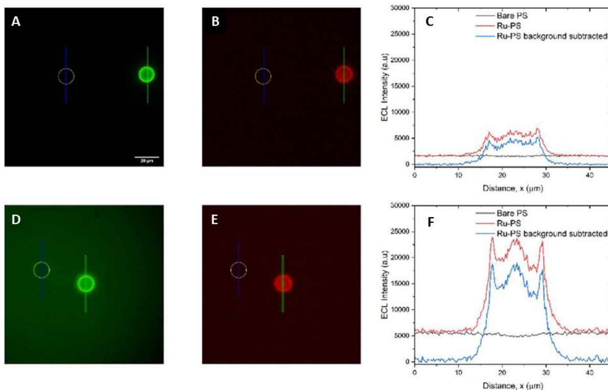
Figure 3.11. Representative top-view configuration PL micrographs ( A and D ) and ECL micrographs ( B and E ) obtained in Procell ( A and B ), and Procell with 100 μM [\text{Ir}(\text{sppy})_3]^{3-} ( D and E ) including 180×4 pixel rectangles (shown in blue and green) used to generate ECL emission profiles ( C and F , respectively) of bare PS beads (circled in yellow) and Ru@PS beads (circled in red) 1.2 V, 1 s CA pulse, EM-CCD exposure 2 s. To generate the bare-PS background subtracted profiles (blue lines, C and F ) the bare PS profile (black lines, C and E ) was subtracted from the raw Ru@PS profile (red lines, C and F ).
