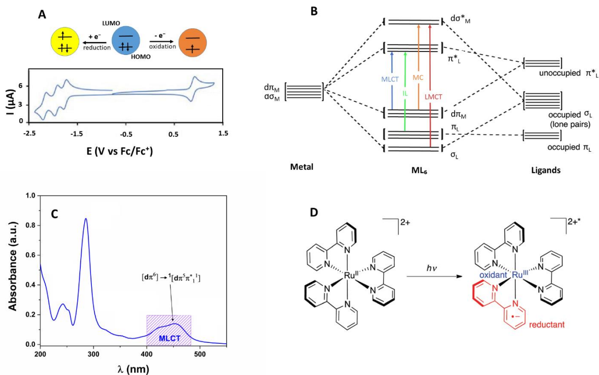
Figure 1.2 (A) Schematic representation of the electronic configuration of frontier orbitals upon oxidation and reduction and a CV of 5 mM [Ru(bpy) 3 ] 2+ solution in acetonitrile containing 0.1 M tetrabutylammonium hexafluorophosphate supporting electrolyte. Reproduced from 27 . (B) Simplified molecular orbital diagram of an octahedral transition metal complex with π-acceptor ligands (i.e Ru(bpy) 3 ] 2+ ). Possible types of electronic transitions from the ground to the first excited electronic state — metal to ligand (MLCT), interligand (IL), metal-centred (MC) and ligand to metal charge transfer (LMCT) — are indicated by the arrows. Reproduced from 28 (C) Electronic absorption spectrum of [Ru(bpy) 3 ] 2+ in water at ambient temperature, with MLCT band highlighted in the purple hatched region. Reproduced from 29 . (D) Schematics depicting the charge separation following the electronic excitation of the Ru(bpy) 3 ] 2+ luminophore. Reproduced from 28 .
