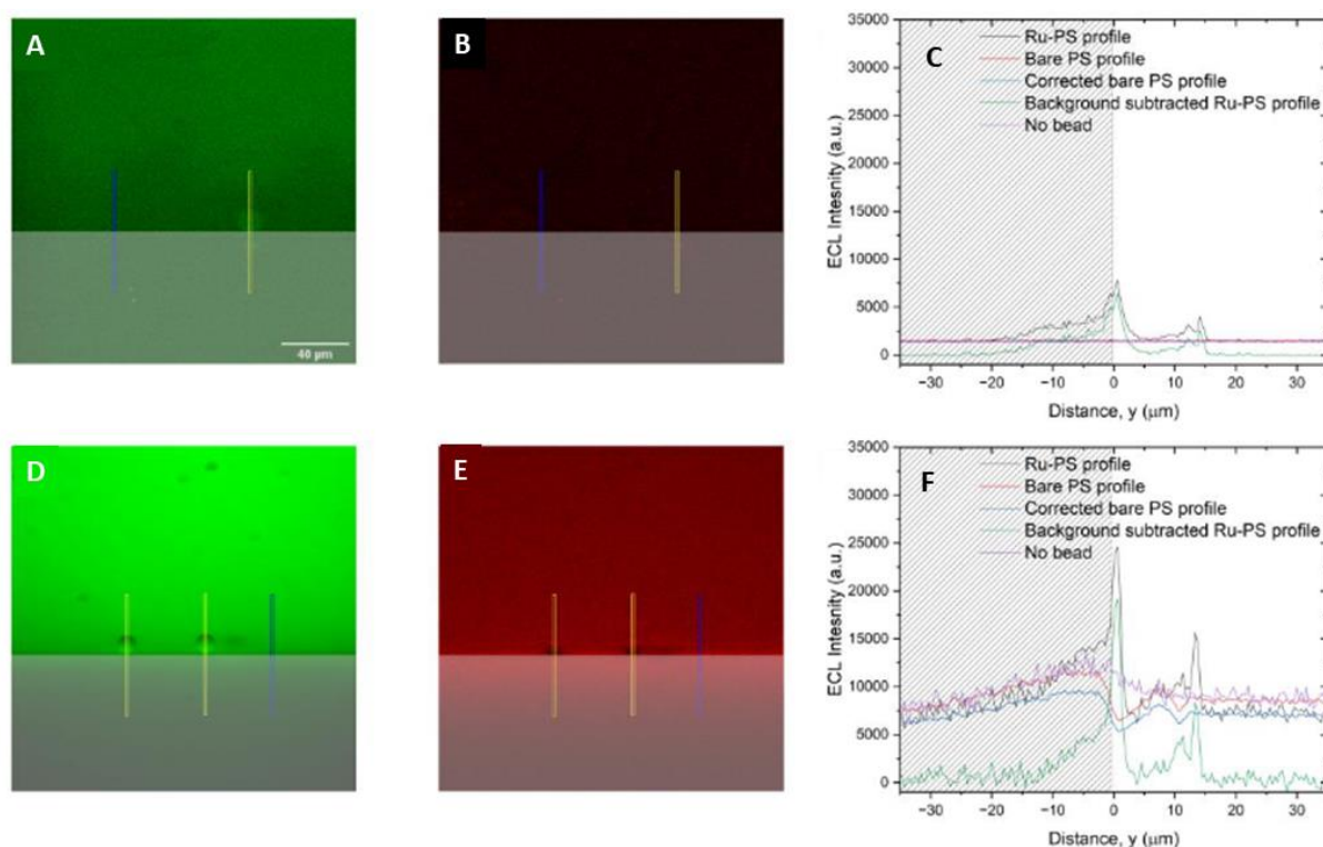
Figure 3.10. Representative side-view configuration PL micrographs ( A and D ) and corresponding ECL micrographs ( B and E ) obtained in ProcCell ( A and B ) and ProcCell with 100 \mu\text{M} [\text{Ir}(\text{sppy})_3]^{3-} ( D and E ) including shaded zone representing reflection of ECL on the electrode surface ( z < 0 \mu\text{m} ) 180 \times 4 pixel rectangles (shown in yellow) used to generate ECL emission profiles ( C and F , respectively) of unlabeled PS beads in side-view configuration at 1.2 V (2 s CA pulse, EM-CCD exposure 3 s), hatched zone represents reflection of ECL on the electrode surface ( z < 0 \mu\text{m} ). Blue rectangles, away from the PS spheres, show the background ECL profile; i.e. from [\text{Ir}(\text{sppy})_3]^{3-} in solution only (purple lines in figures C and F ). To generate the background subtracted profiles (green lines, C and F ) the maximum of the first 10 pixels ( \sim 3.97 \mu\text{m} ) of ECL emission (where no emission from Ru@PS was observed) was calculated for both Ru@PS (black lines) and bare PS (red lines) profiles. A correction factor was applied to the bare PS profile (blue lines) to normalize the bare PS profile to the Ru@PS profile. This corrected bare PS profile was then subtracted from the raw Ru@PS profile to generate the background subtracted Ru@PS profile (green lines).
