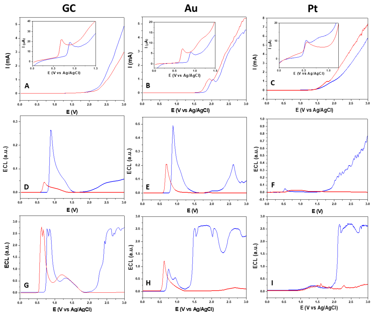
Figure 4.2. (A-C) Linear sweep voltammograms at 0.1 \text{ V s}^{-1} from 0 V to 3.0 V in 0.2 M PBS (pH = 8) with 50 mM \text{KNO}_3 (red) and KCl (blue) on (A) GC electrode, (B) Au electrode, (C) Pt electrode. Insets (A-C) show the electrochemical oxidation of L-012 in \text{KNO}_3 (red) and KCl (blue) supporting electrolytes on different working electrodes. (D-I) Corresponding evolution of the ECL intensity with electrode potential during a linear potential sweep at 0.1 \text{ V s}^{-1} from 0 V to 3.0 V in 0.2 M PBS (pH = 8), 0.42 mM L-012, 50 mM \text{KNO}_3 (in red) or KCl (in blue) and (D-F) 0 M \text{H}_2\text{O}_2 or (G-I) 0.5 M \text{H}_2\text{O}_2 on (D and G) GC electrode, (E and H) Au electrode, (F and I) Pt electrode.
