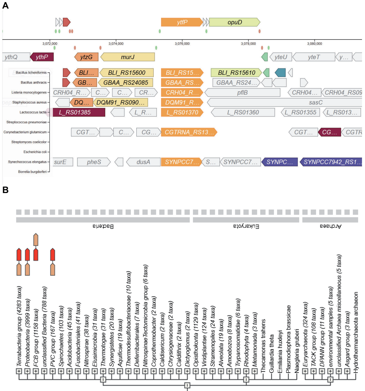
Figure S8: Examples of Sporadic gene neighborhood associations between of COG2081 and RNA modifications enzymes. (A) Physical clustering between dusA and the COG2081-encoded homolog in Syneccoccus elongatus extracted from ( http://corewiki.uni-goettingen.de/gene/3184 ); (B) Physical clustering associations in the String Database using the family search tool between COG2081 (Predicted flavoprotein YhiN) in red and COG1187 (Pseudouridylate synthase RsuA) in orange. https://string-db.org/cgi/network?taskId=bU9CkNV4A16g&sessionId=bplhPKknoWLb&allnodes=1
