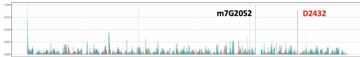
Figure S7: AlkAlinine-Seq profile of V. cholerae 23S rRNA
