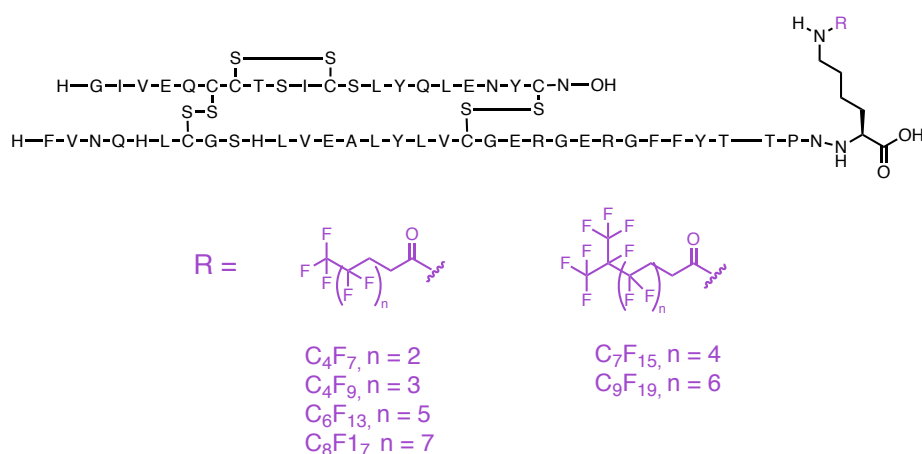
Figure 36 : Structures des fluoro-insulines.
