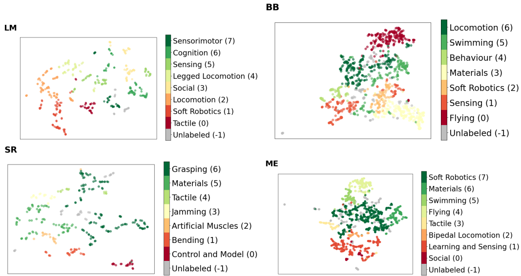
Figure 3.3: Clustering of research themes by natural language processing (NLP). The latent representations of articles are computed using the SciBERT model and projected in a two-dimensional space for the various corpora. The topic labels and their associated colors are assigned after applying the HDBSCAN clustering algorithm on a 5 or 10-dimensional projection (depending on the corpus) of the SciBERT latent representations. Dimensionality reductions are performed with UMAP. Naming the clusters is done manually by inspecting the n-grams and checking some articles belonging to the cluster.
