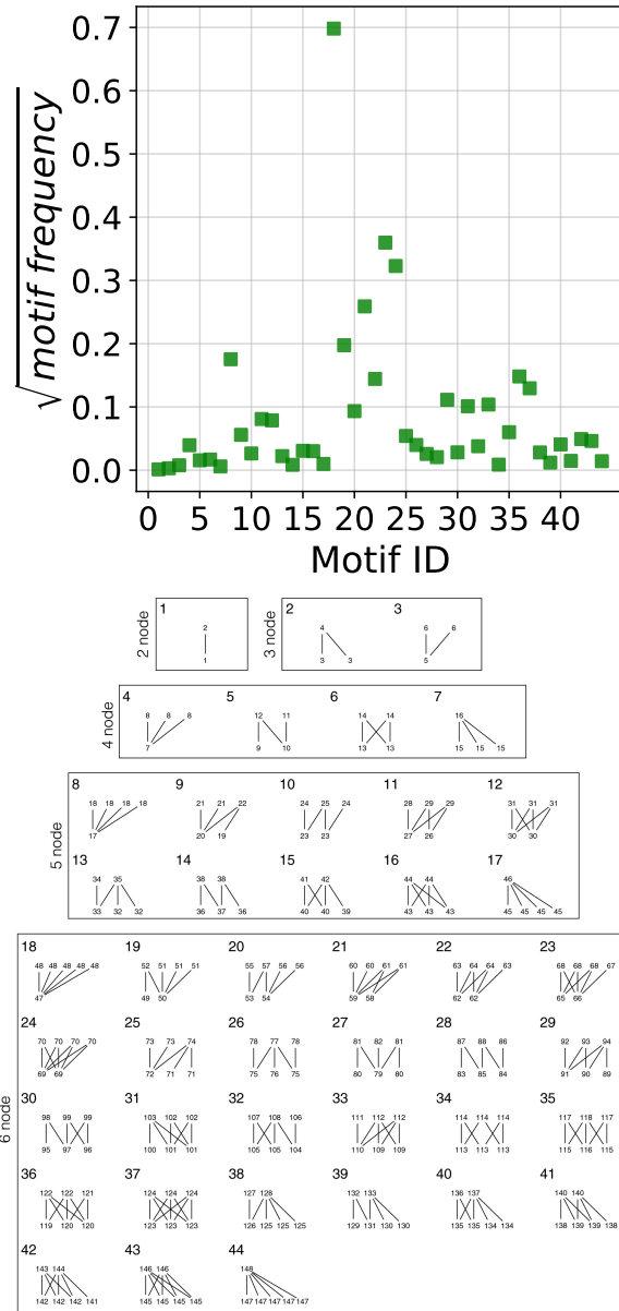
Figure 4.8: Bipartite motif analysis of the investor community-patent cluster network. Top : frequencies of bipartite network motifs found on the investor community-patent cluster network. Motif frequencies were computed using the bmotif package [272]. Bottom : shape corresponding to each motif ID (taken from [272]). Comparisons with the motif frequencies shown in [238] do not easily allow for the discrimination between antagonistic and mutualistic networks.
