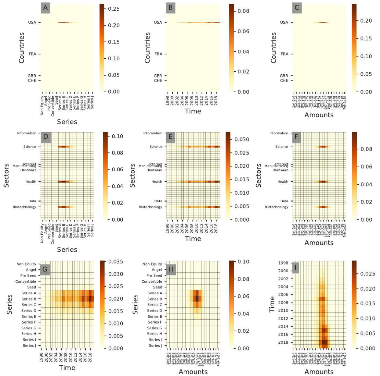
Figure 2.14: Cross-interaction heatmaps for community A7. These distributions correspond to Health Care specialists.
