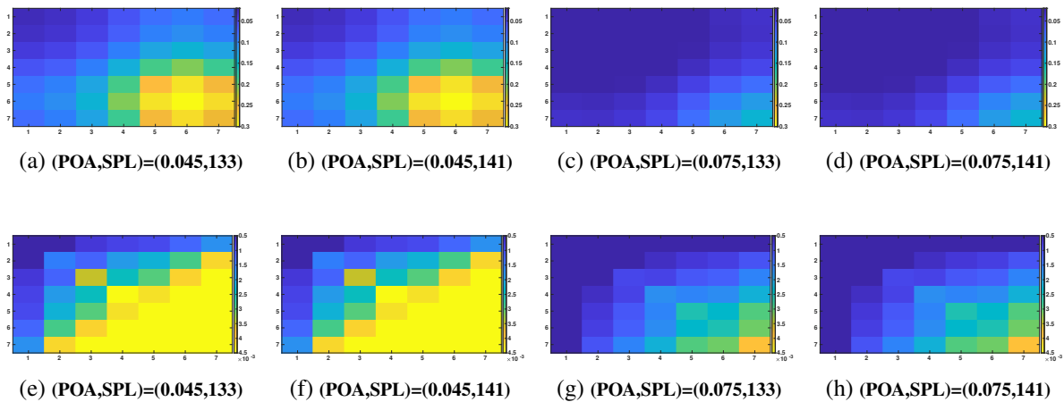
Figure 3.3: Conditional covariance matrices with statistical ANN-based metamodel estimation of the conditional covariance of resistance (Figs.3.3a to 3.3d) and reactance (Figs. 3.3e to 3.3h) given four different values of \mathbf{w}
