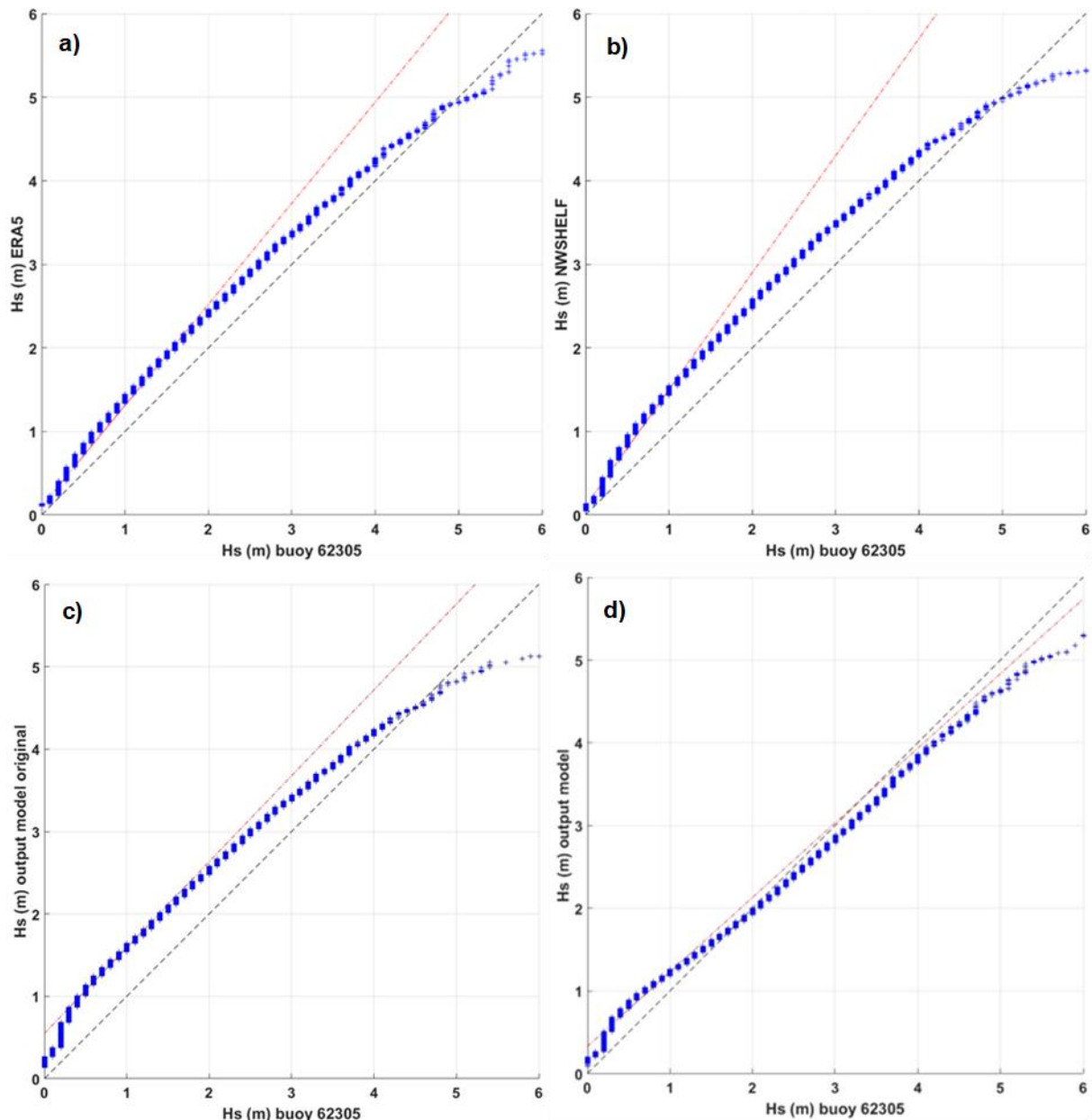
Figure 45. QQplots of significant wave height ( H_s ) comparison of reanalysis or results of modelling versus observations measured by buoy 62305: a) reanalysis of ERA5, b) reanalysis of NWSHELF, c) results of the simulations from the Delft3D model forced with the original values of wind, and d) results with the calibrated values of wind speed. Extracted from López Solano et al. (2024)
