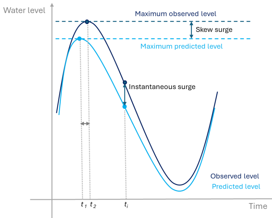
Figure 16. Calculation of the skew surges S from the measurements of sea level of the tide gauges. Adapted from the website of SHOM ( refmar.shom.fr )
