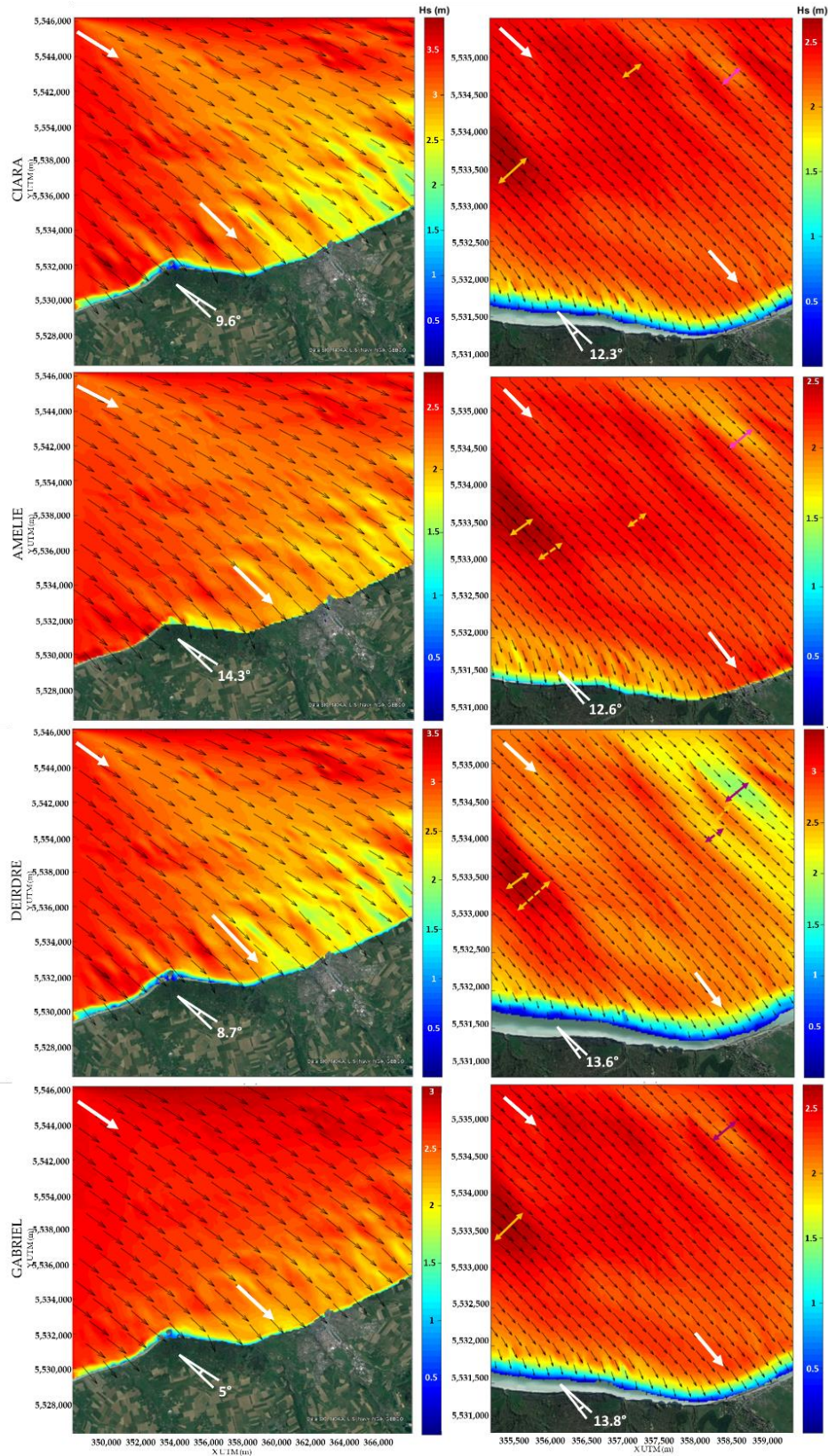
Figure 63. Distribution maps at the peak of the storm of H_s and \theta in the coarse grid (a,c,e,g) and nested grid (b,d,f,h) in Etrétat for Ciara (February 2020) (a,b), Amelie (November 2019) (c,d), Deirdre (December 2018) (e,f) and Gabriel (January 2019) (g,h) storms. White arrows show the refraction of waves when approaching to coast. Extracted from López Solano et al. (2022)
