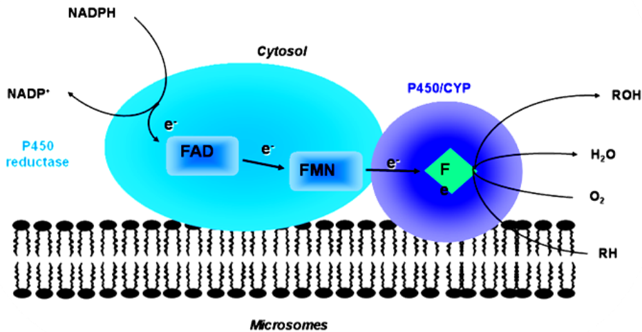
Figure 4. Reactive oxygen species production and redox cycling by CYP monooxygenases. CYPs of the monooxygenase subfamily contain a heme-based catalytic center, an NADPH reductase subunit, and an NADH/NADPH oxidase as cofactors. CYP450s are present in ferric and ferrous forms and the initial chemical reaction that takes place is the binding of a substrate to the ferric form. CYP450 reductase donates an electron to reduce the ferric form to a ferrous intermediate which then binds to an oxygen molecule to form a complex. The complex is reduced by the addition of a proton which is concomitant with H 2 O production and an oxenoid complex whereby activated oxygen bound to the heme moiety incorporates into the substrate to yield an oxidized form (Johnston et al., 2011; Adapted from Eid et al., 2014).
