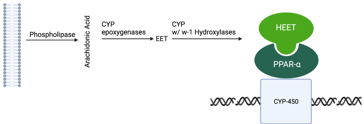
Figure 7. Transcriptional control of CYP-Hydroxylases and Epoxygenases. (Figure created by BioRender.com)
