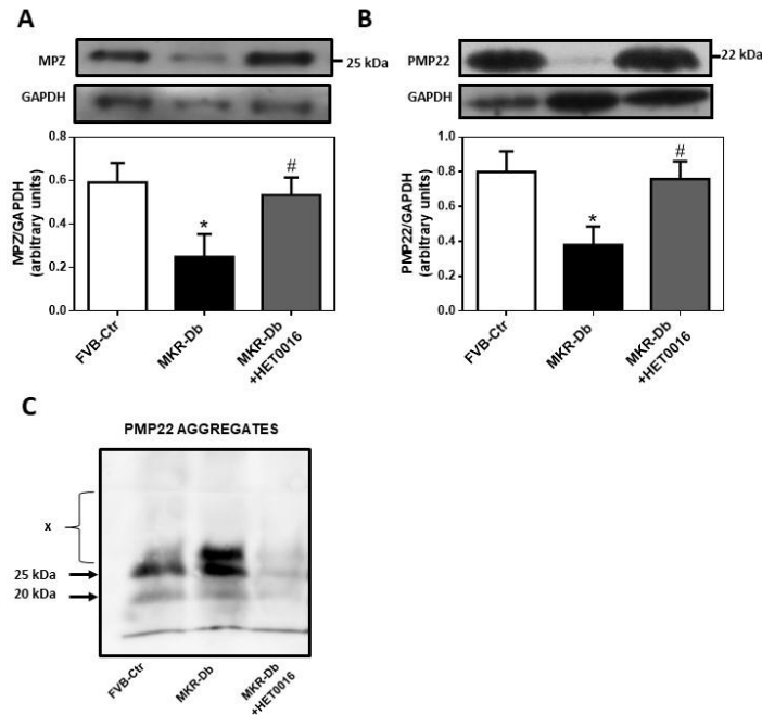
Figure 12. HET0016 administration intercepts diabetes-induced alterations in MPZ and PMP22 myelin protein profiles in the sciatic nerve of MKR non-obese T2D mice. Myelin protein soluble and insoluble profiles were assessed via western blot in sciatic nerves isolated from FVB control mice, MKR non-obese type 2 diabetic mice, and MKR non-obese type 2 diabetic mice treated with HET0016. Representative western blots with their respective densitometric quantification are shown for (A) MPZ (n=5) and (B) PMP22 (n=6-7). (C) Putative western blot of the insoluble PMP22 aggregates indicated by x. Values are the means \pm SE. *P<0.05, vs. control. #P<0.05, vs. MKR.
