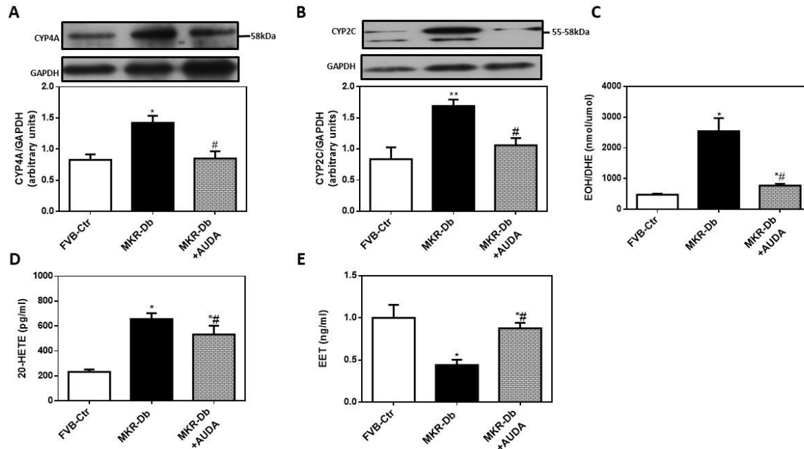
Figure 23. sEH inhibition with AUDA restores EET levels and alleviates CYP-dependent ROS overproduction in sciatic nerves of MKR non-obese T2D mice. Diabetes-associated oxidative injury was assessed in sciatic nerves isolated from FVB control, MKR non-obese type 2 diabetic mice and MKR non-obese type 2 diabetic mice treated with AUDA. The expression and activity of hydroxylase and epoxygenase CYPs was examined. Representative Western blot analysis of (A) CYP4A expression (n=3) and (B) CYP2C (n=4) with the respective densitometric quantification. (C) Assessment of superoxide generation in sciatic nerves via HPLC analysis (n=8-10). CYP activity was reflected by assessment of endogenous (D) 20-HETE and (E) EET production via HPLC analysis (n=8-10). Values are the means \pm SE. *P<0.05, vs. control. #P<0.05, vs. MKR.
