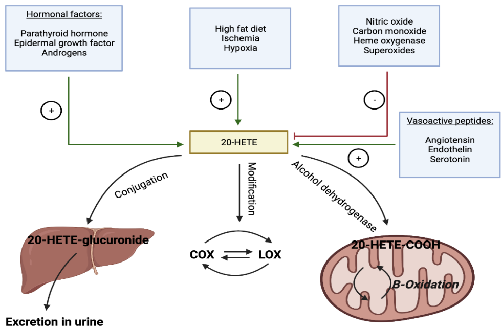
Figure 6. Metabolic regulation of 20-HETE. (Figure created by BioRender.com)
