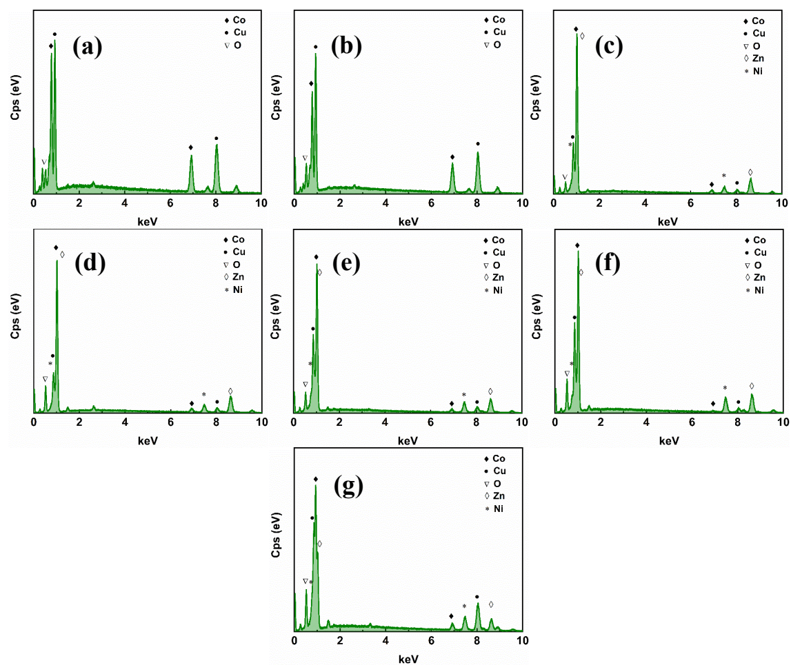
Figure 5.6 EDS curves of different deposited alloys before and after heat treatment steps and dealloying. a) The deposited Co on Cu; b) The deposited Co on Cu after the heat treatment; c) The deposited Zn-Ni on Co-Cu alloy; d) The deposited Zn-Ni on Co-Cu alloy after the heat treatment. The dealloyed Zn-Ni-Co-Cu alloys for different treatment times: 0.5 h (e), 1 h (f) and 2 h (g).
