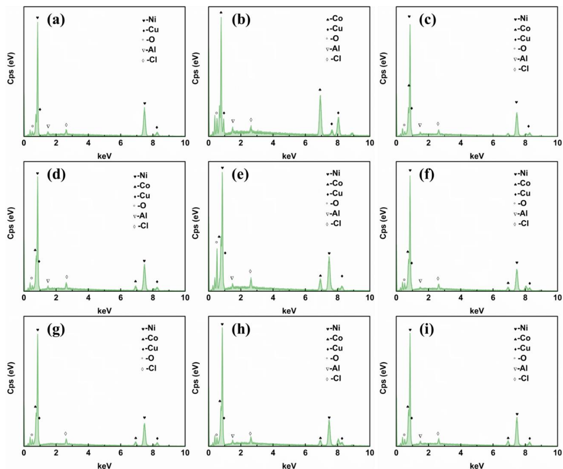
Figure 3.25 EDS spectra of electrodeposition on Cu foil. a) Ni deposition. b) Co deposition. Ni-Co alloys prepared at c) -1.0 \text{ V/Ag/Ag}^+ , 1 h, 60^\circ \text{C} , d) -1.05 \text{ V/Ag/Ag}^+ , 1 h, 60^\circ \text{C} , e) -1.1 \text{ V/Ag/Ag}^+ , 1 h, 60^\circ \text{C} , f) -1.05 \text{ V/Ag/Ag}^+ , 0.5 h, 60^\circ \text{C} , g) -1.05 \text{ V/Ag/Ag}^+ , 2 h, 60^\circ \text{C} , h) -1.05 \text{ V/Ag/Ag}^+ , 1 h, 40^\circ \text{C} , i) -1.05 \text{ V/Ag/Ag}^+ , 1 h, 80^\circ \text{C} .
