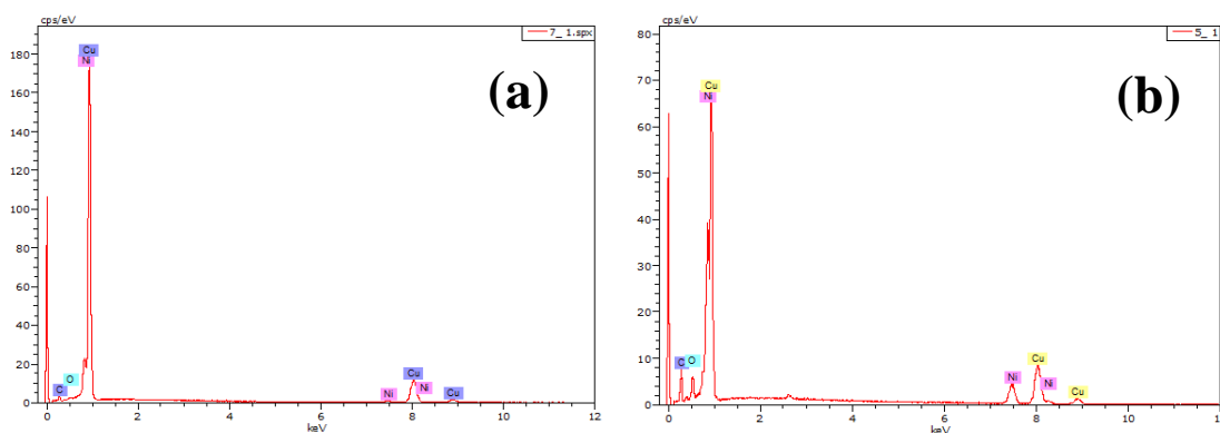
Figure 4.5 EDS analysis of electrodeposited Ni on Cu foam at 40°C from Menthol-DES for 5 h (a) and 15 h (b).
