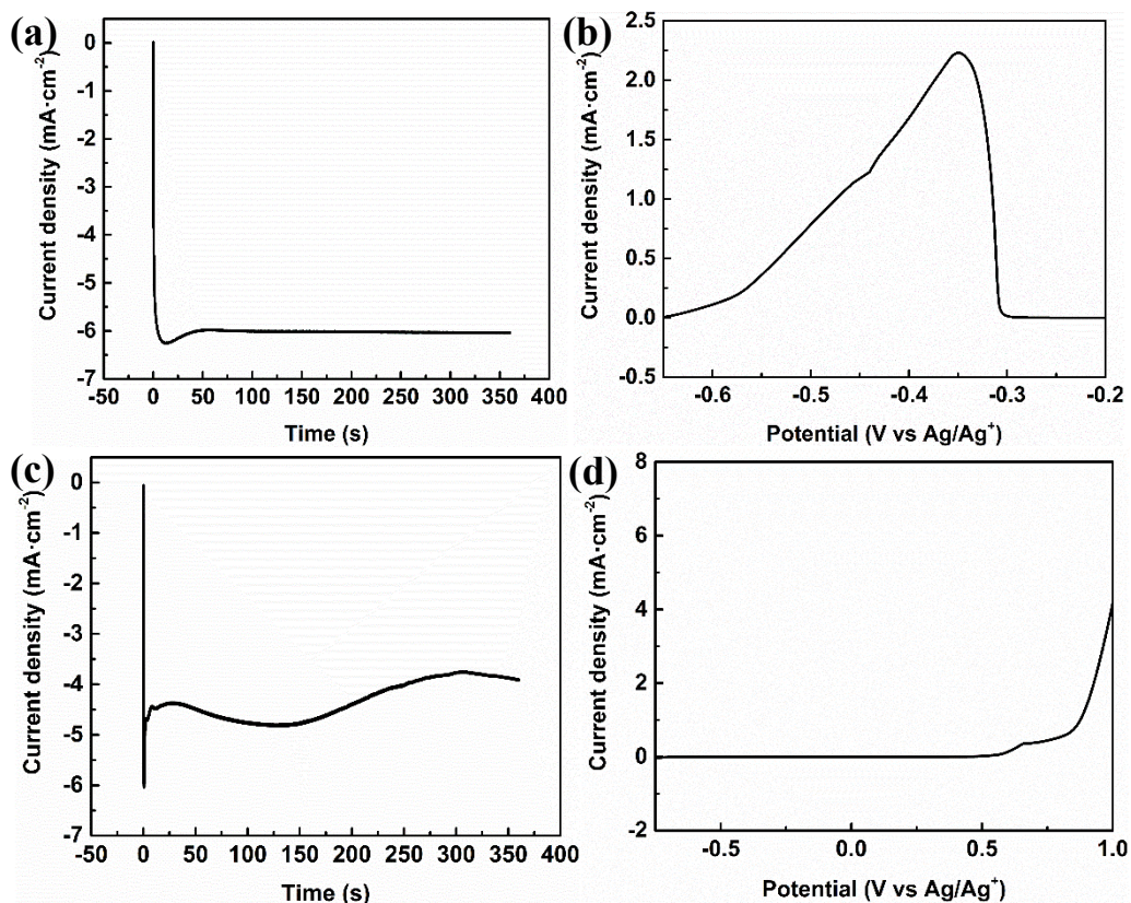
Figure 3.6 a) Chronoamperometry curve and oxidation LSV curve of \text{Ni}^{2+} and \text{Co}^{2+} on glassy carbon.
