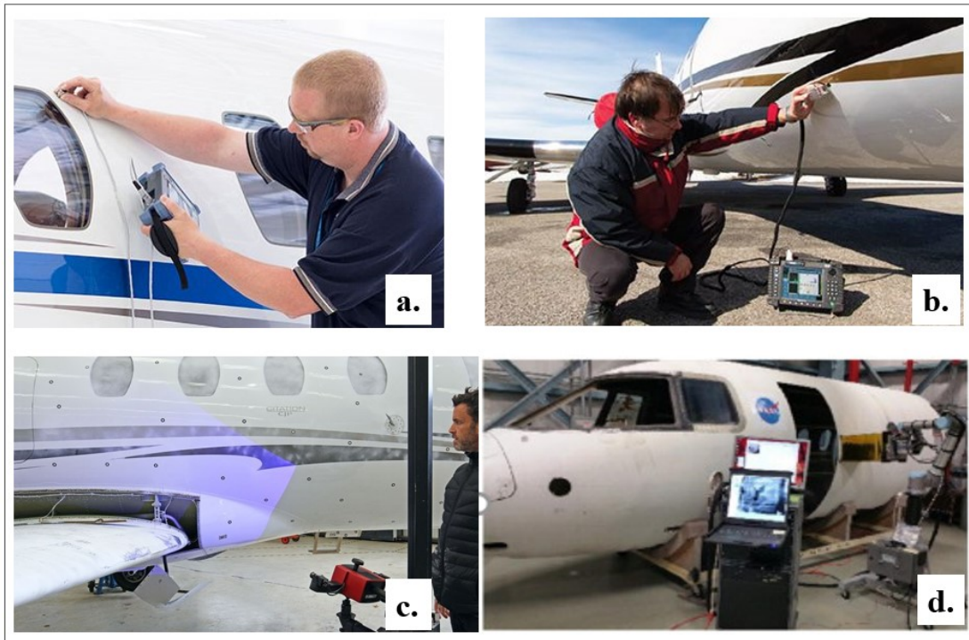
Figure 1.4: Illustration of NDT techniques currently applied in damage diagnosis of aerostructures, adapted from www.makepartsfast.com and www.gom.com .
