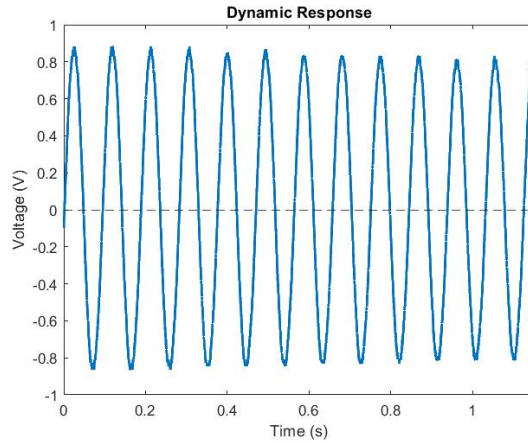
Figure 3.14: The smart composite vibration tests voltage response obtained at the structure's resonance frequency with a recorded peak-to-peak voltage of approximately 1.8 V.
