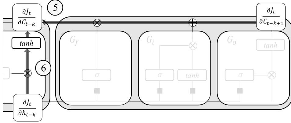
Figure 4.16: Two paths that the gradients backpropagate to C_{t-k} . Gradients that backpropagate through the path (5) don't get vanishing or exploding thanks to the lack of activation function.
