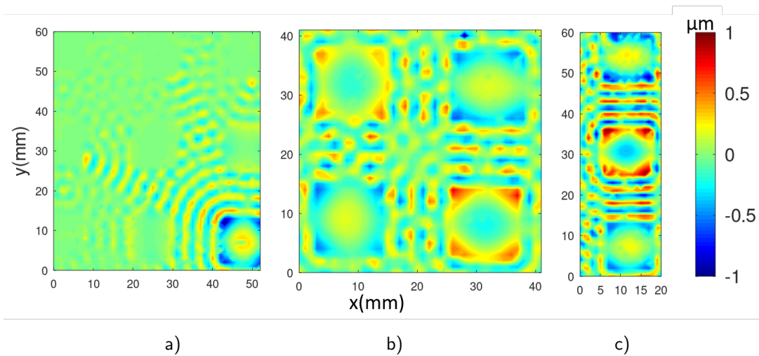
Figure 3.19: Displacement measurements for different configurations.
