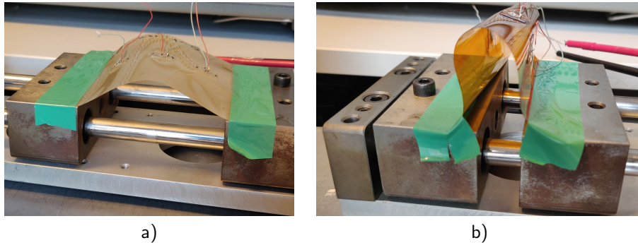
Figure 3.26: a) Large curve radius for PEEK; b) Small curve radius for KAPTON.
