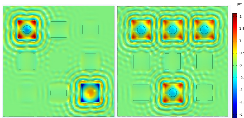
Figure 3.16: Displacement field for two points and for a line and a point.
