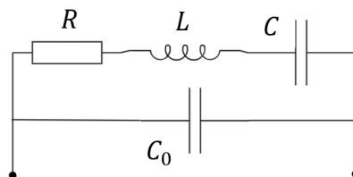
Figure 2.16: Butterworth Van Dyke model for a piezoelectric transducer.
