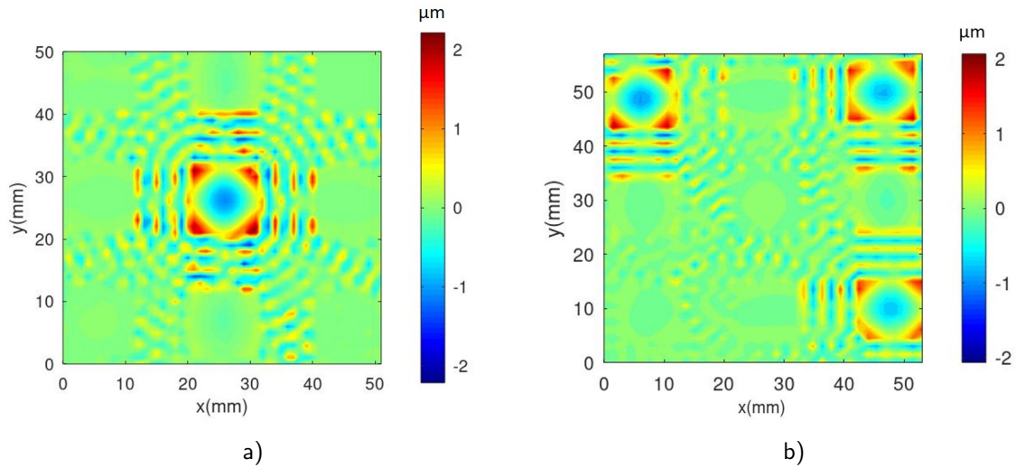
Figure 5.2: Displacements field for a) one actuated resonator and for b) three.
