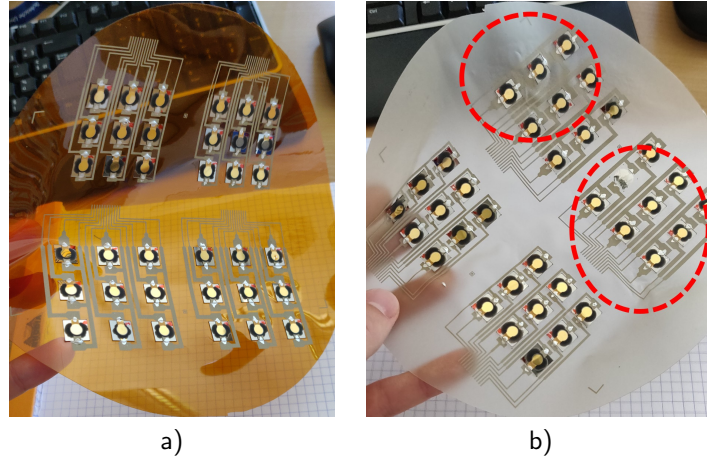
Figure 4.9: a) The instrumented KAPTON polymer and b) the instrumented PEEK polymer after the release of the REVALPHA film.
