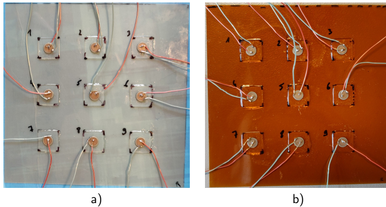
Figure 3.18: a) PEEK 100 \mu\text{m} with 9 resonators; b) KAPTON 75 \mu\text{m} with 9 resonators.
