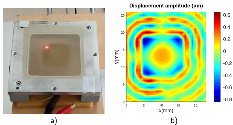
Figure 2.23: a) Setup for measurement ; b) Displacement amplitude for the mode of vibration (PEEK assembly - 20 Vpp).
