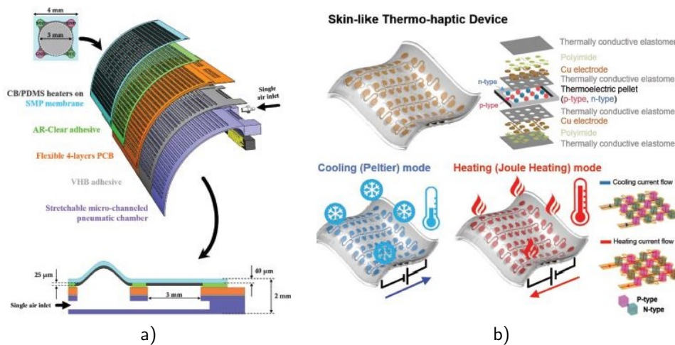
Figure 1.19: a) Pneumatic solution [94]; b) Thermohaptic solution [95].
