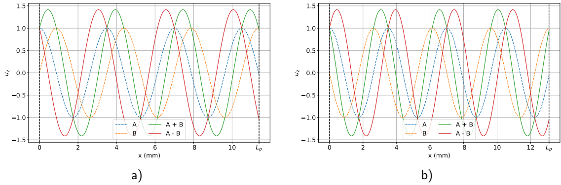
Figure 3.9: Transversal displacement for a) L_p = 11.4 mm or b) L_p = 13.1 mm with a PEEK film obtained with the model.
