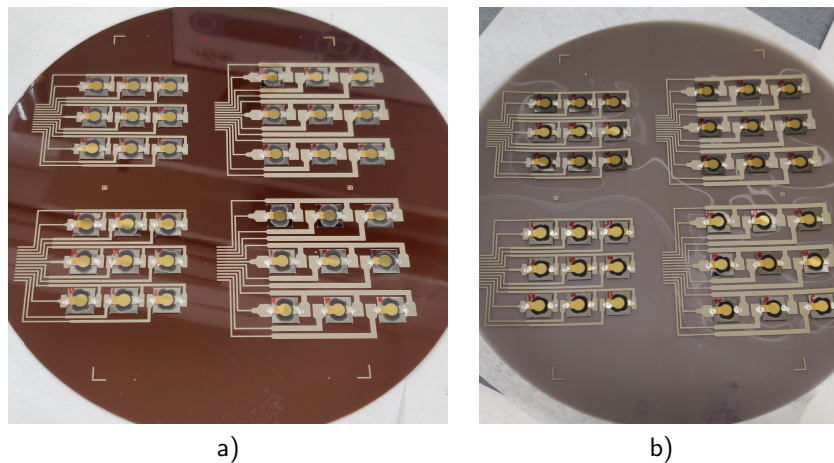
Figure 4.8: Substrate with a) the instrumented Kapton polymer and b) the instrumented PEEK polymer.
