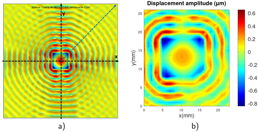
Figure 3.1: a) FEM and b) Mapping of one resonator at the resonance.
