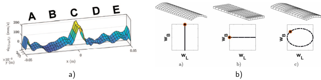
Figure 1.10: a) Experimental cartography for modal superimposition [50] ; b) Superimposition of two modes to obtain a click [51].
