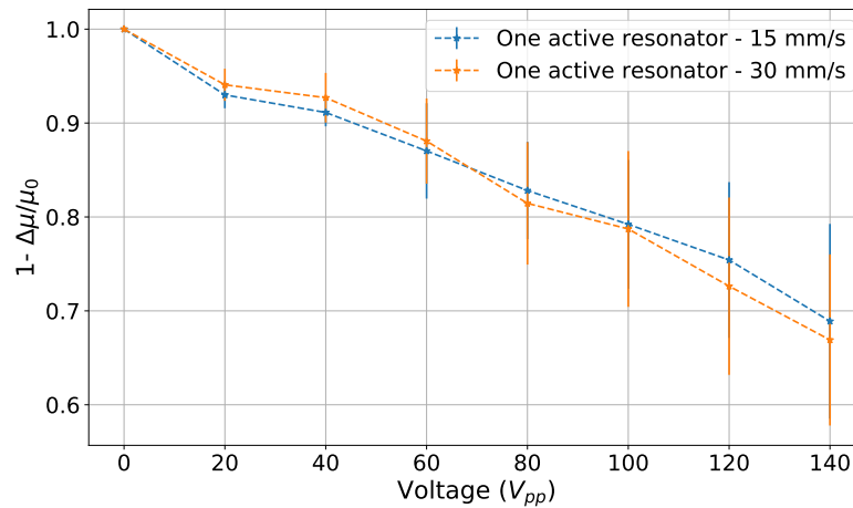
Figure 5.13: Friction reduction for one active resonator.
