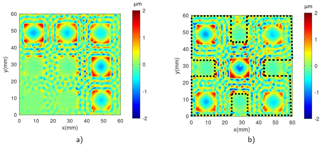
Figure 5.5: Displacement measurement on the surface: a) : activated L-shape; b): activated X-shape.
