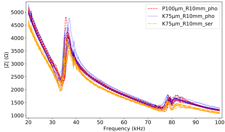
Figure 4.13: Impedance obtained for surfaces with PEEK-100 \mu\text{m} and KAPTON-75 \mu\text{m} .
