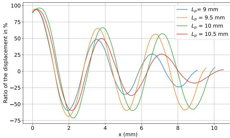
Figure 3.5: Displacement amplitude on the polymer film between one active and one passive resonator for various L_p .
