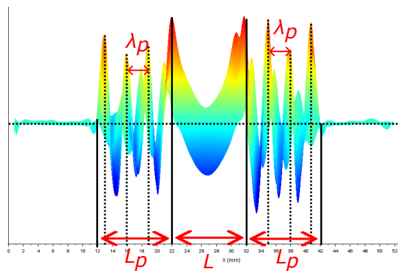
Figure 5.3: Transverse view : the central resonator active and the 2 others passive.
