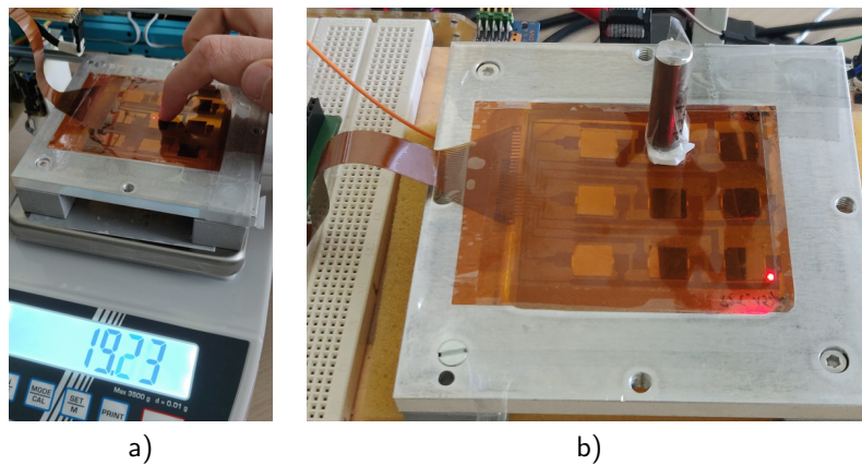
Figure 5.8: a) Set up for measurement with a finger and b) with a cylindrical mass.
