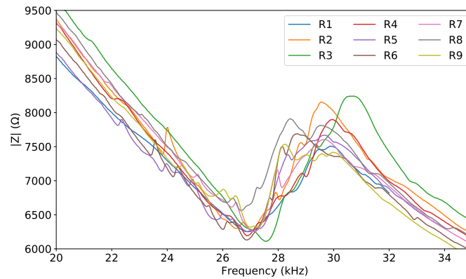
Figure 3.20: Impedance obtained for the 9 resonators of the surface with PEEK 100 \mu\text{m} and a space of 13 mm.
