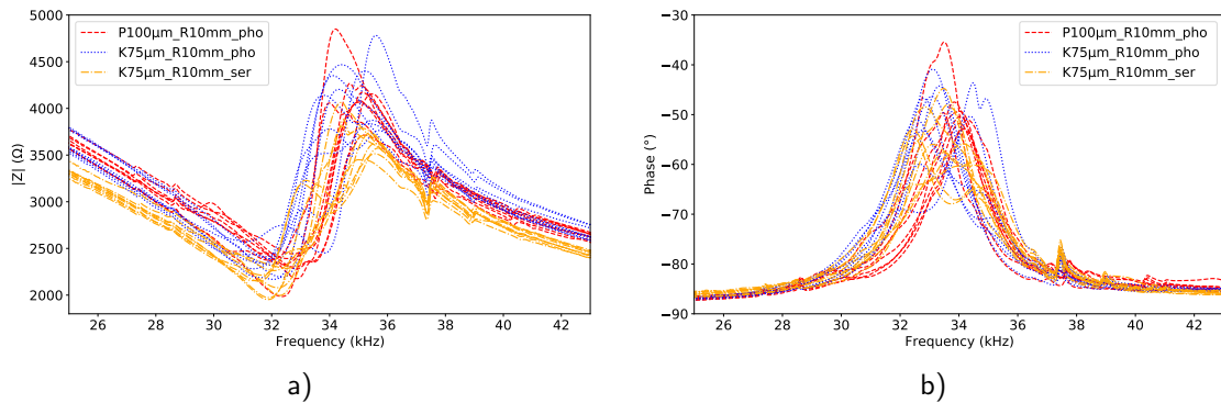
Figure 4.14: a) Impedance and b) phase obtained for the three surfaces around the resonance.
