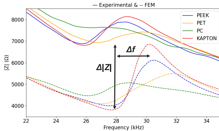
Figure 2.22: Impedance modulus obtained with the FEM study (- -) and experimental (-) results.
