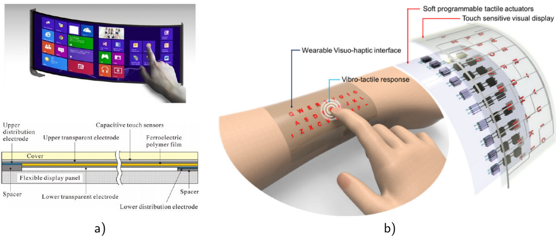
Figure 1.16: a) Haptic interface with PVDF actuators [84]; b) Haptic interface with dielectric microactuators [85].
