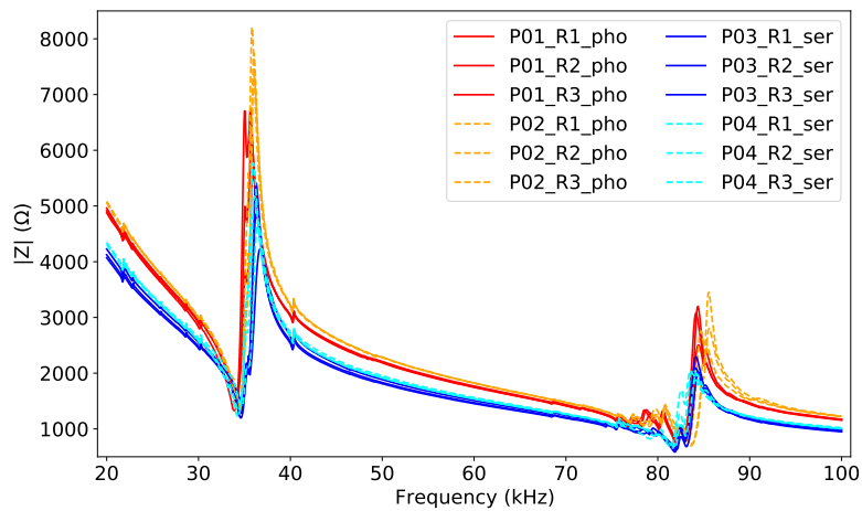
Figure 4.11: Impedance obtained for three resonators of two different substrate for the two methods of fabrication of the bottom electrode.
