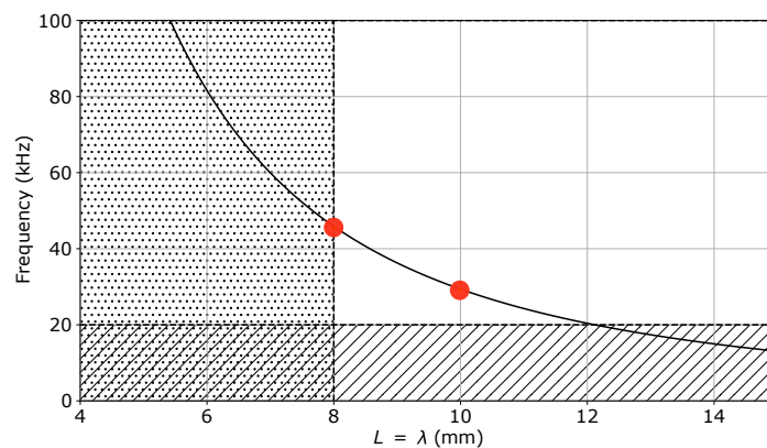
Figure 2.12: Evolution of the frequency for the (2,0 + 0,2) mode.
