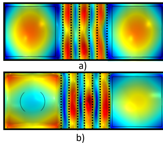
Figure 3.10: Transversal displacement for L_p = 11.4 mm : a) Resonators in phase with 6 nodes of vibrations, b) Resonators in out of phase with 7 nodes of vibrations.
