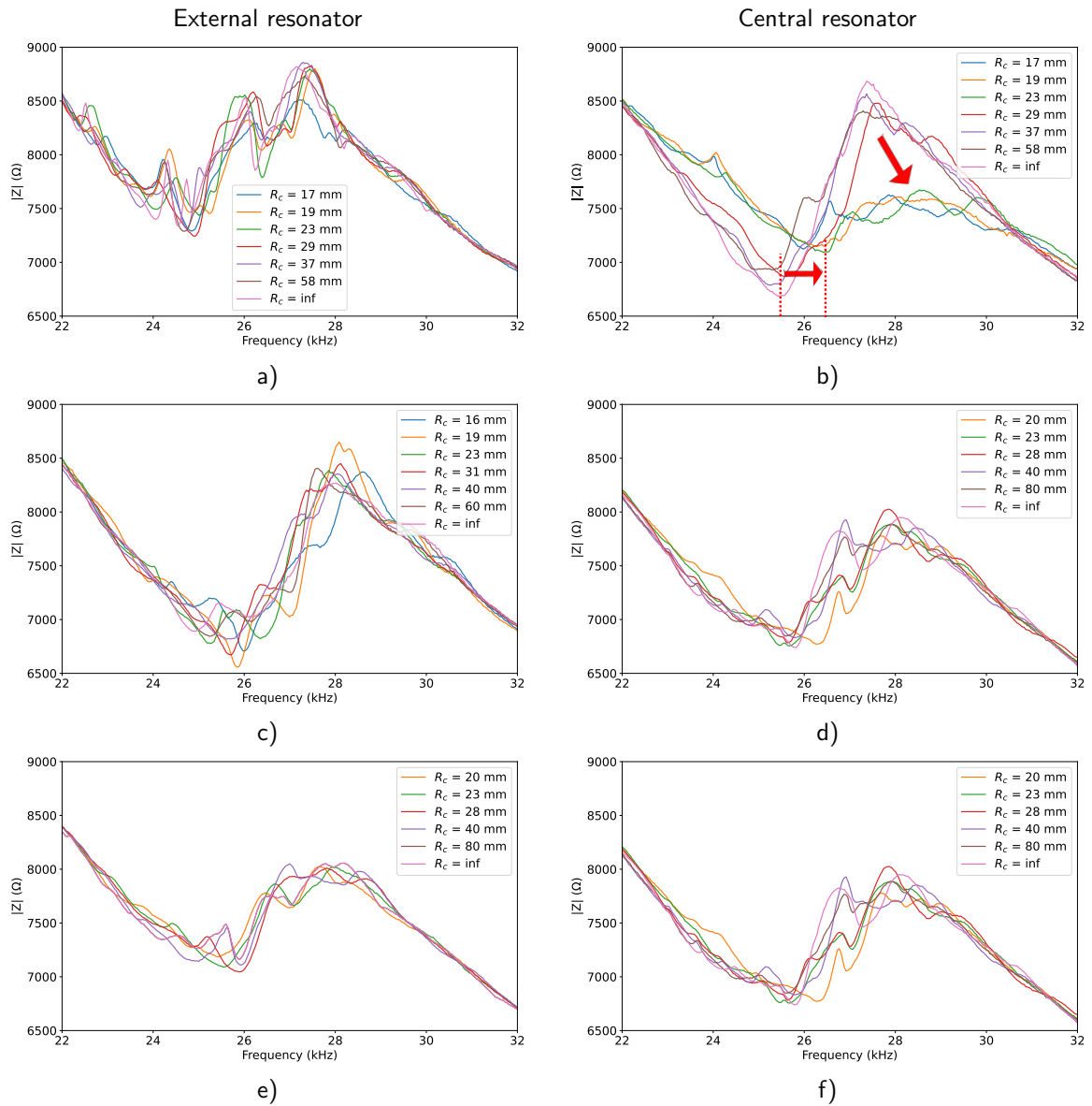
Figure 3.27: Impedance of external resonator : a) 6 mm gap, c) 10 mm gap, e) 13 mm gap; Impedance of central resonator : b) 6 mm gap, d) 10 mm gap, f) 13 mm gap.
