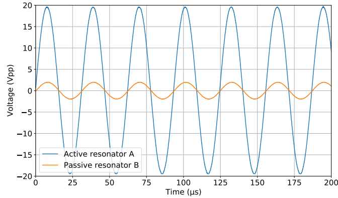
Figure 4.25: Actuation signal of resonator A and captation signal of resonator B.
