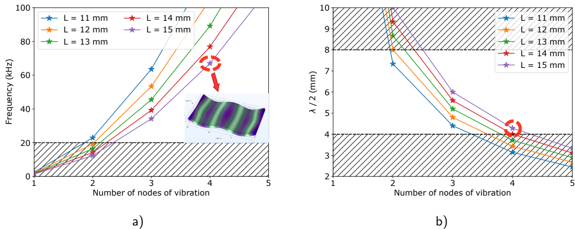
Figure 2.8: Evolution of Lamb A0 modes as a function of the length L and the number of nodes.
