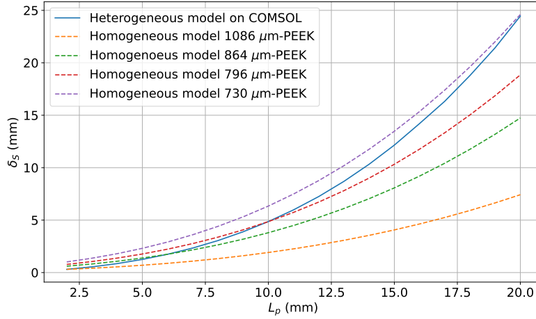
Figure 3.24: Deflection \delta_S obtained with the heterogeneous model on COMSOL and with homogeneous beam model.
