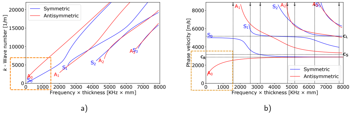
Figure 2.5: a) Wave number evolution for the Lamb mode of a glass plate; b) Phase velocity evolution for the Lamb mode of a glass plate.
