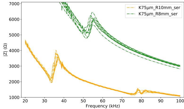
Figure 4.15: Impedance obtained for 10 mm x 10 mm resonators or 8 mm x 8 resonators.
