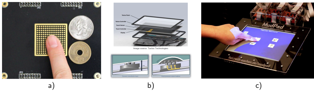
Figure 1.6: a) Electrode array [37]; b) Fluidic chamber [40]; c) Magneto-rheological chamber [41].
