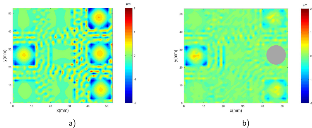
Figure 5.9: Surface displacement measurements : a) Without the mass; b) With the mass.
