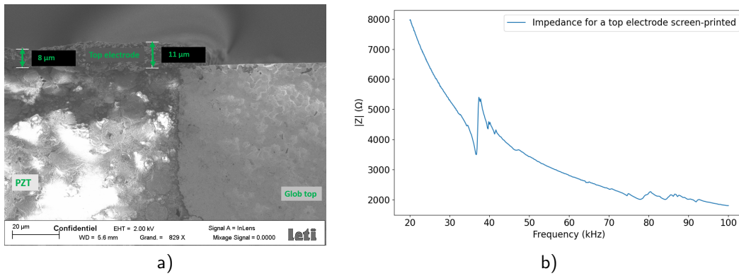
Figure 4.22: a) SEM cross-section and b) Impedance obtained for the top electrode in silver.
