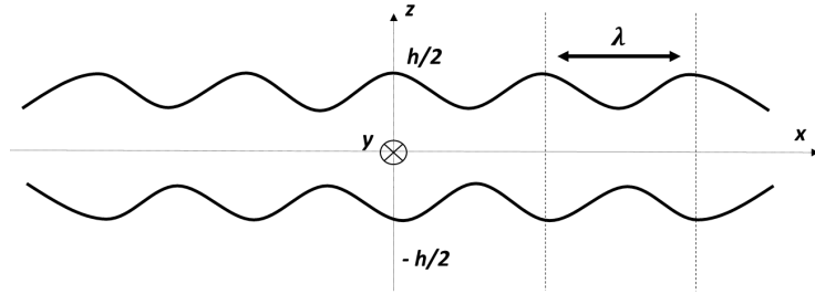
Figure 2.3: Symmetrical plate mode S_0 .
