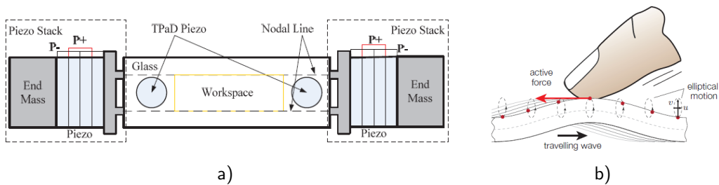
Figure 1.15: a) Lateralpad [74]; b) Operation of Ultraloop solution [75].
