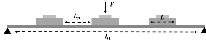
Figure 3.22: Haptic surface assimilated to a bending beam.
