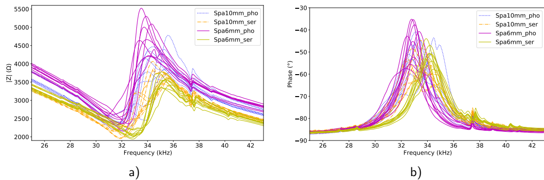
Figure 4.16: a) Impedance and b) phase obtained for space of 10 mm and 6 mm between resonators.
