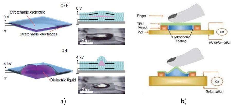
Figure 1.18: a) HAXEL [92]; b) Actuator based on acoustofluidics [93].
