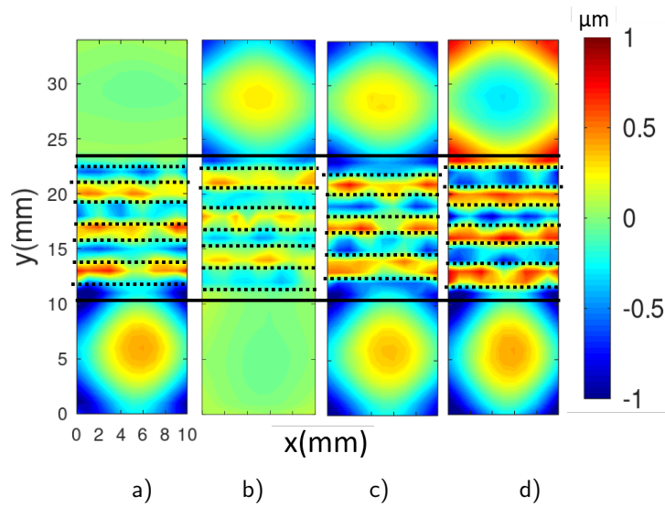
Figure 3.12: Amplitude displacement for 4 different situations.
