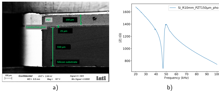
Figure 4.24: a) SEM cross-view and b) Impedance of the silicon resonator.
