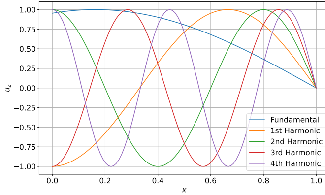
Figure 3.8: First mode of vibration of an undamped free-clamped beam.
