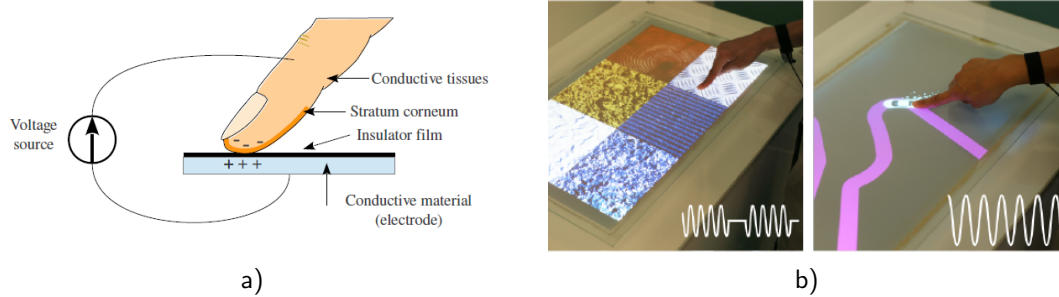
Figure 1.11: a) Operation of electrovibration [55]; b) Testatouch [53].
