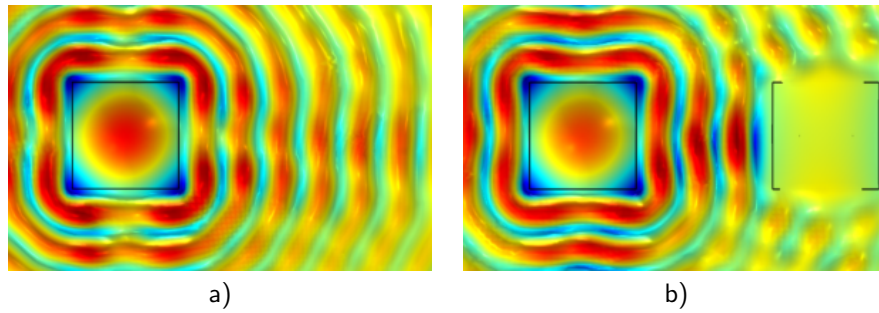
Figure 3.4: Vibration mode without (a) and with (b) adjacent passive resonators.
