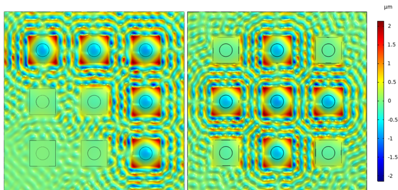
Figure 3.17: Displacement field for a "L" shape and a "+" shape.
