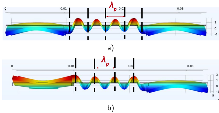
Figure 3.11: Cross-view of two haptic resonators on COMSOL: a) L_p = 14.9 mm , b) L_p = 13.1 mm.
