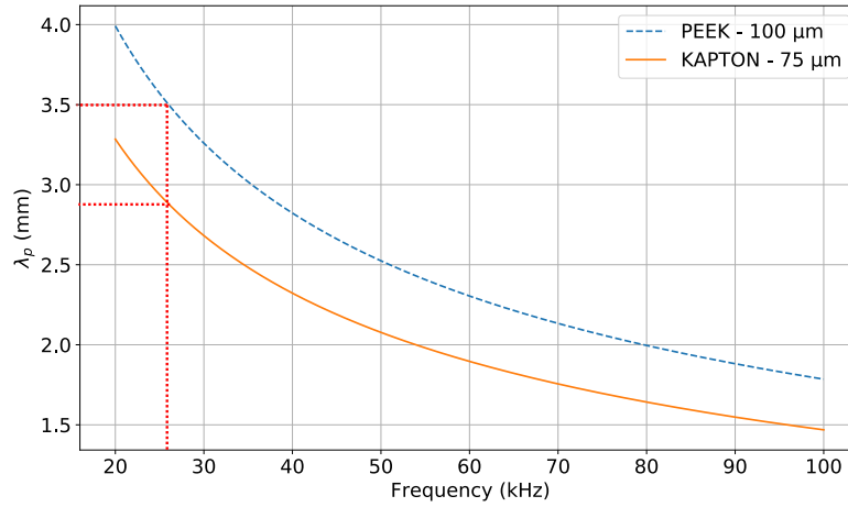
Figure 3.2: \lambda_p on the polymer films.
