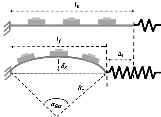
Figure 3.25: Set-up drawing for bending study.
