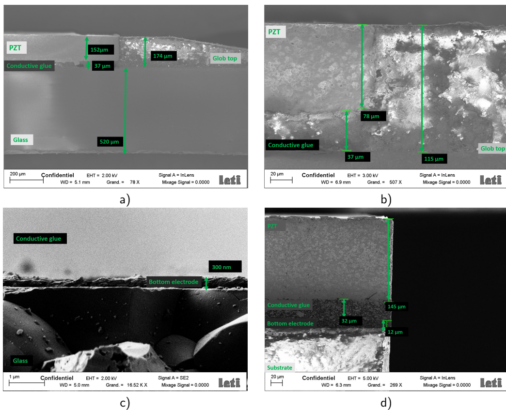
Figure 4.5: SEM cross-sections of resonators with a PZT thickness of: a) 150 µm or b) 75 µm; c) Zoom on the gold bottom electrode and d) Resonator with a silver bottom electrode.
