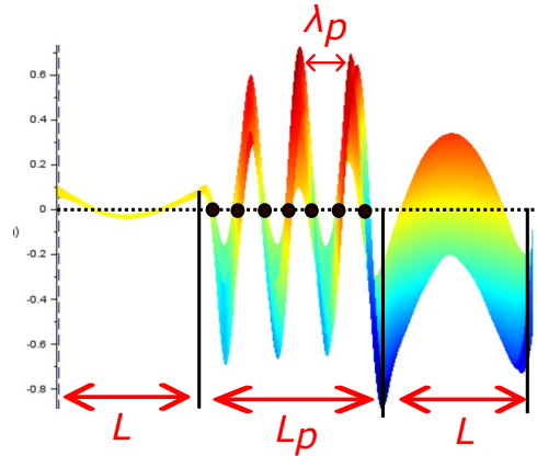
Figure 3.13: Transverse view for one active and one passive resonator for L_p = 13.1\text{mm} .
