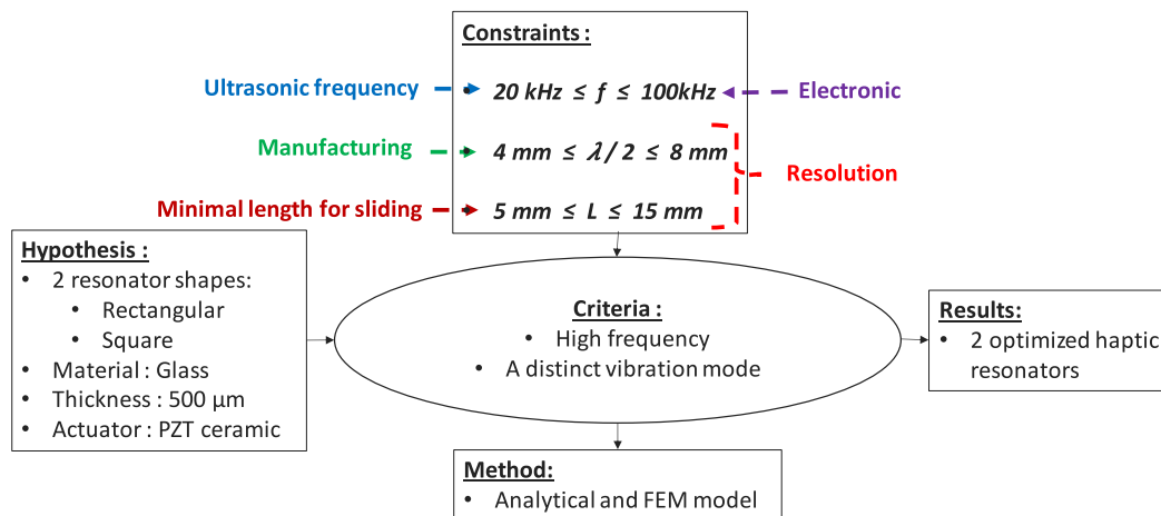
Figure 2.6: Methodology to design two haptic resonators.
