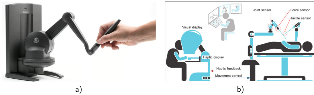
Figure 1.3: a) Phantom device "Touch X" [21]; b) Operation of a robot for surgery with haptic feedback [23].
