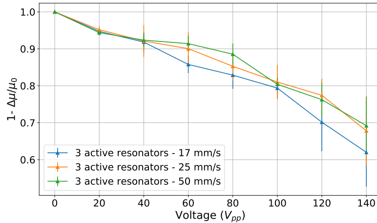
Figure 5.14: Friction reduction for a line of three active resonators.
