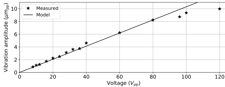
Figure 5.4: Amplitude of displacement at 32 kHz.
