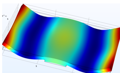
Figure 2.9: Displacement field at resonance with the PZT actuator.
