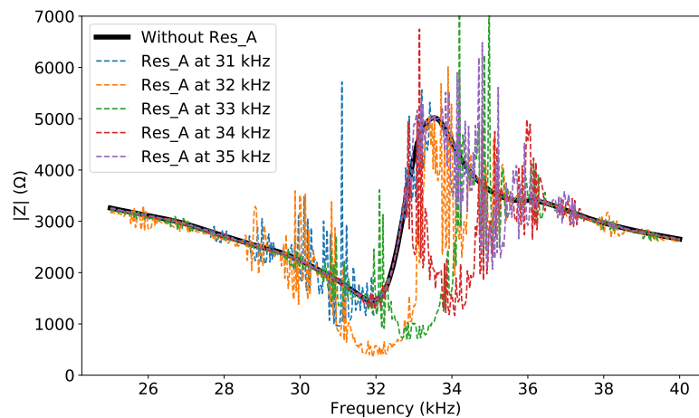
Figure 4.27: Impedance variation on B when an adjacent resonator A is actuated at different frequencies.
