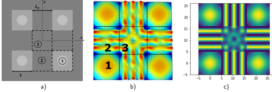
Figure 3.15: a) Model of 4 resonators, b) Displacements fields for L_p = 11.4 mm obtained with COMSOL and c) with the simplified model.
