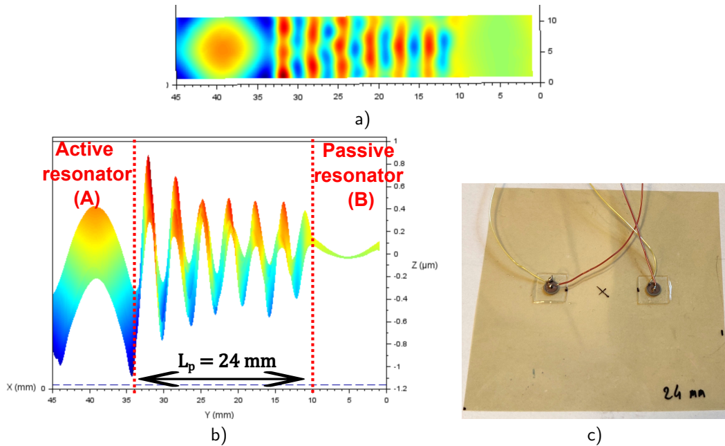
Figure 3.6: Measurement of the displacement field for L_p = 24 mm : a) Top view, b) Transverse view and c) Assembly used.
