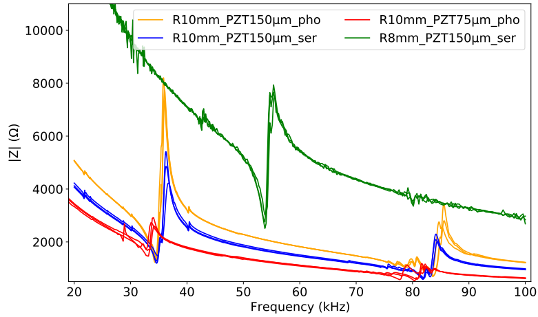
Figure 4.12: Impedance obtained for three resonators of each design.
