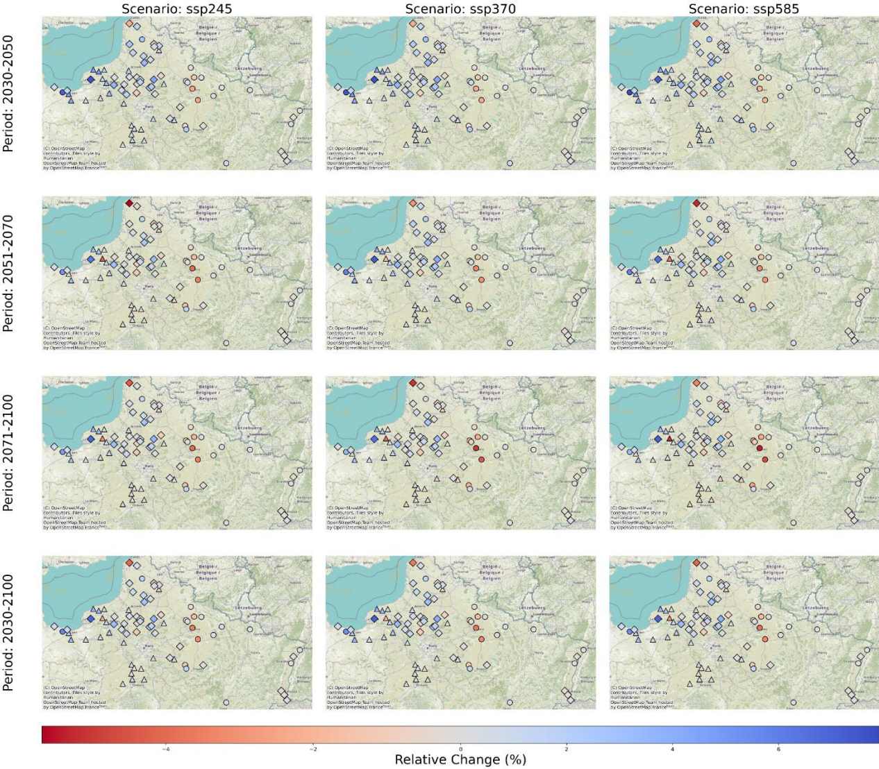
Relative Change (1970-2022) in Groundwater Levels for Different Scenarios and Periods
