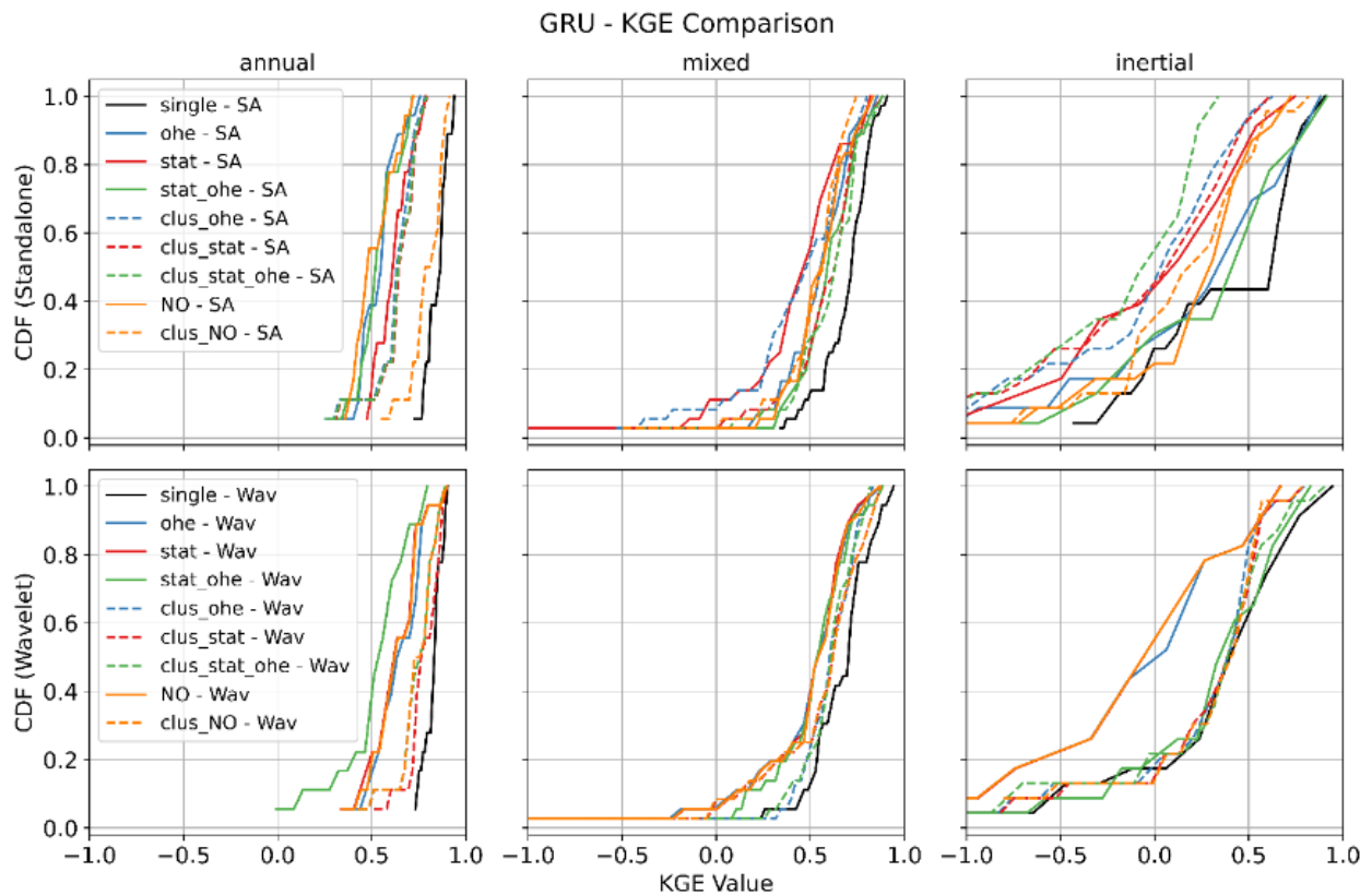
Figure 4.7: CDF Comparison of KGE values of the GRU With different approaches and GWL types.
