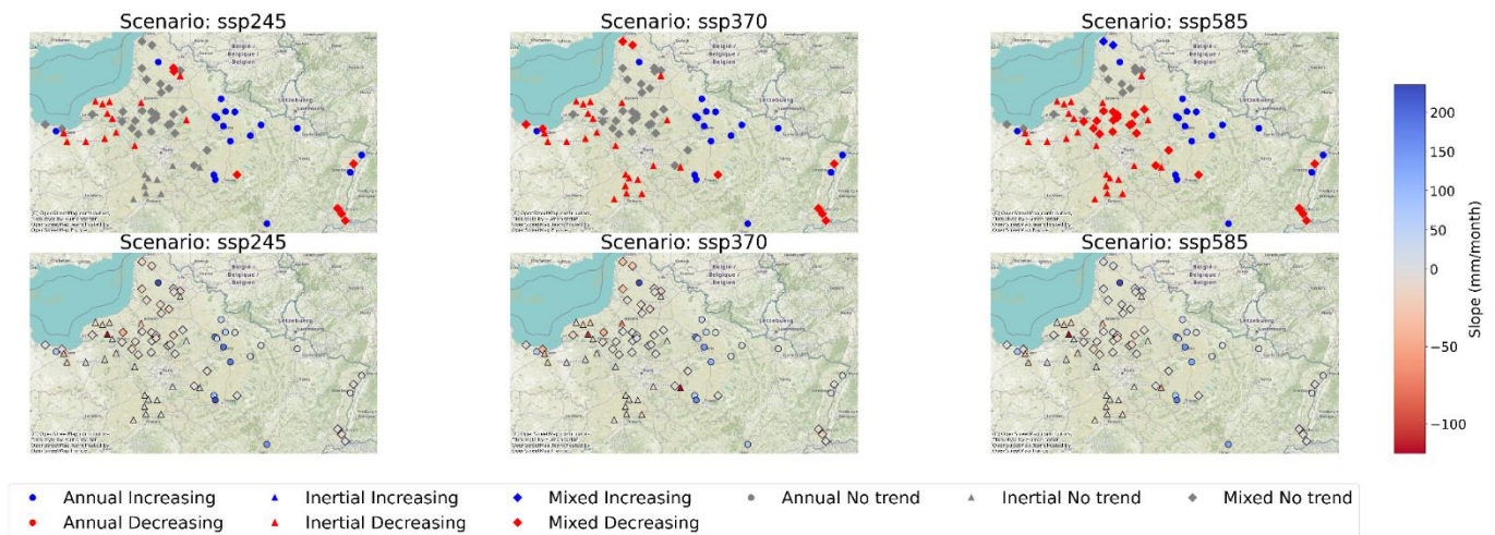
Figure 5.11: Trends and slopes in the total variability of projected GWL
