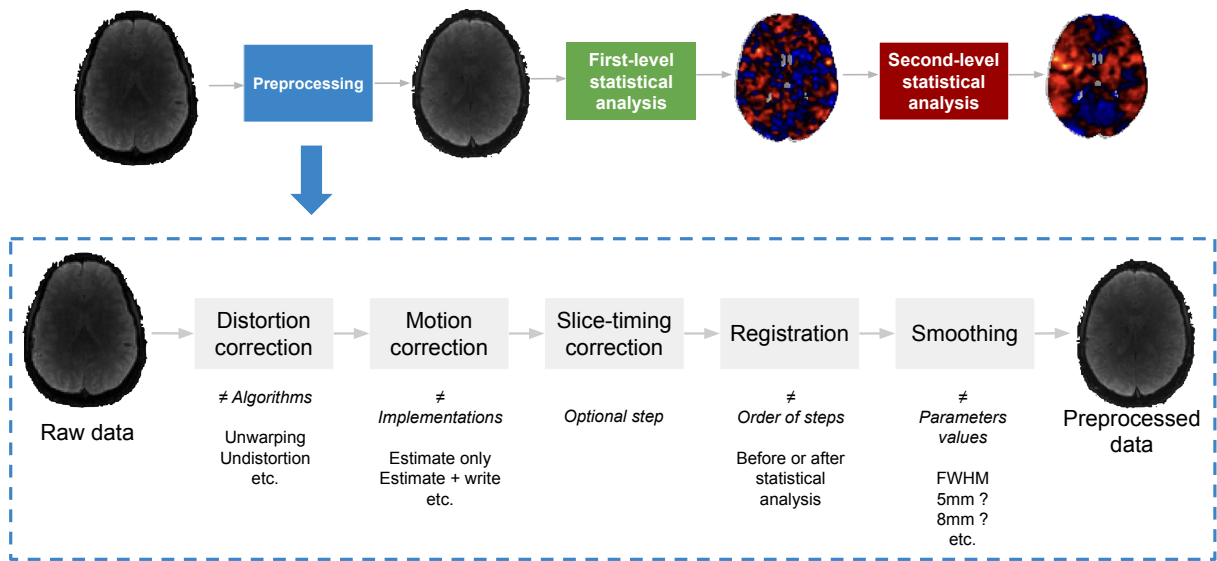
Figure 2.2 – Overview of possible choices to make during a standard fMRI preprocessing pipeline.
