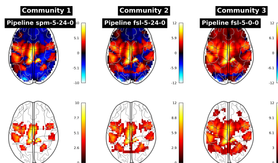
Figure 7.6 – Mean statistic map for the contrast right-foot across groups (of participants) for a representative pipeline in each community. Unthresholded maps (upper) and thresholded maps (lower) with voxelwise FDR-corrected p < 0.05 .
