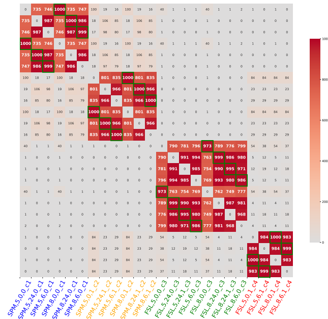
Figure 7.2 – Adjacency matrix representing the number of times each pair of pipelines belong to the same community across different group-level statistic maps of the contrast right-hand
