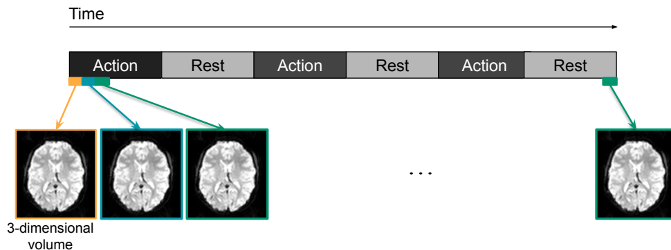
Figure 1.1 – Illustration of common fMRI protocols
