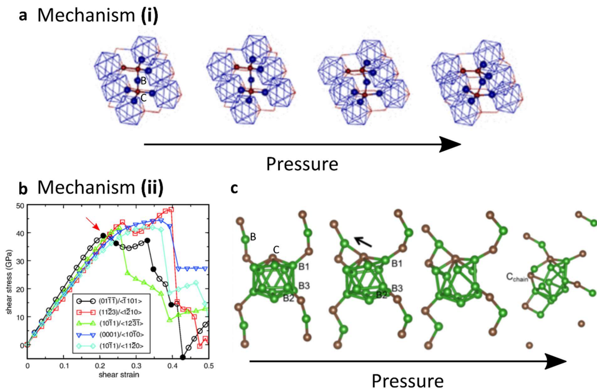
Figure II. 6. Possible amorphization mechanisms of boron carbide. (a) Chain-bending with pressure according to mechanism (i) . (b) Modelled stress/strain curves for the most plausible failure slip planes of boron carbide. The system failing at the lowest strain is marked with a red arrow: (01\bar{1}\bar{1})/\langle\bar{1}101\rangle . (c) Structural visualization of the failure mechanism (ii) .
