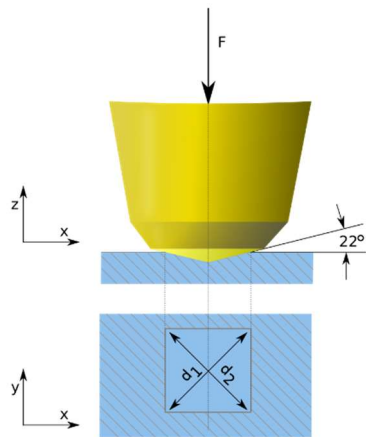
Figure II. 1. Vicker's indentation experiment scheme, reproduced from reference [50].
