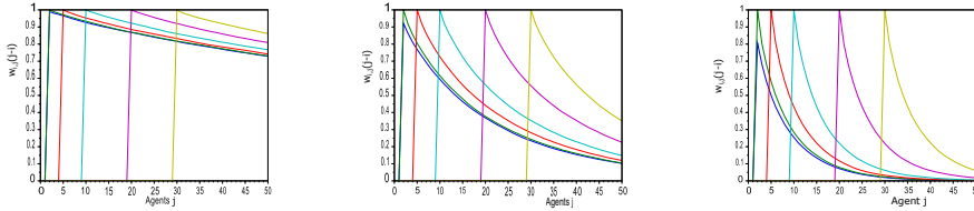
Figure 3.14 – Delayed mutual information w_{i,j}(j - i) as a function of j , for agents i = 1, 2, 5, 10, 20 and 30 (curves from left to right, respectively). The vote of agent i = 0 is forced to 1 and the noise is \epsilon = 0.001 (left panel), \epsilon = 0.01 (middle panel) and \epsilon = 0.05 (right panel).
