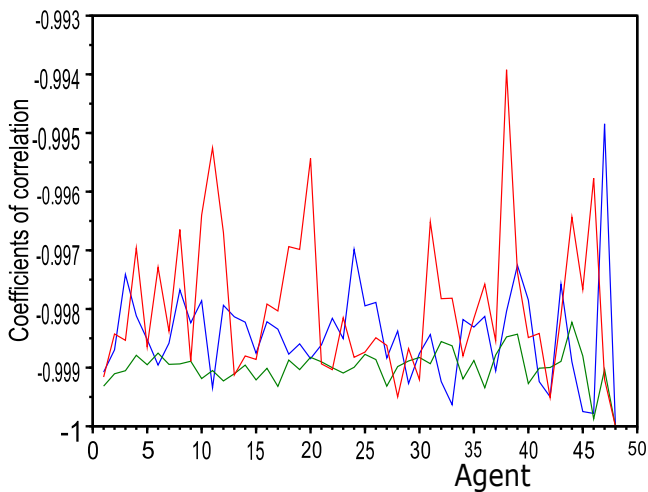
Figure 3.17 – The coefficient of correlation between w_{i,j}(j-i) and i with different noise \epsilon = 0.001, 0.01 and 0.05 .
