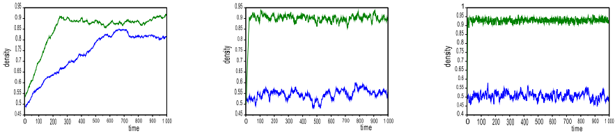
Figure 3.16 – Evolution of the density of vote 1 during the time when only the vote of the agent 1 is forced to 1 (blues curves) and when every vote of the agents j \propto \lfloor \frac{1}{\lambda} \rfloor is forced to 1 (greens curves). left \epsilon = 0.001 . middle \epsilon = 0.01 , right \epsilon = 0.05 .
