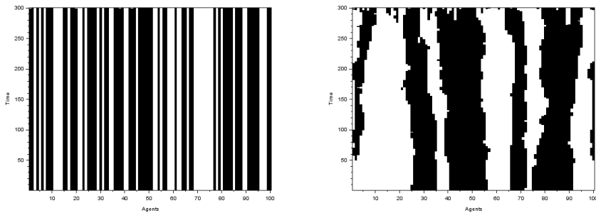
Figure 5.3 – Left: Space time diagram for Wolfram rule 232, computed block-wise for blocks of 3 consecutive agents. The individual cell state values are computed exactly (using rule 232). Then the block state values (black/white) are determined according to the majority projection F . The initial configuration is arbitrary. Right: the same block state values are represented for the proposed coarse-grained elementary stochastic cellular automaton with probabilities given in (5.2.16).
