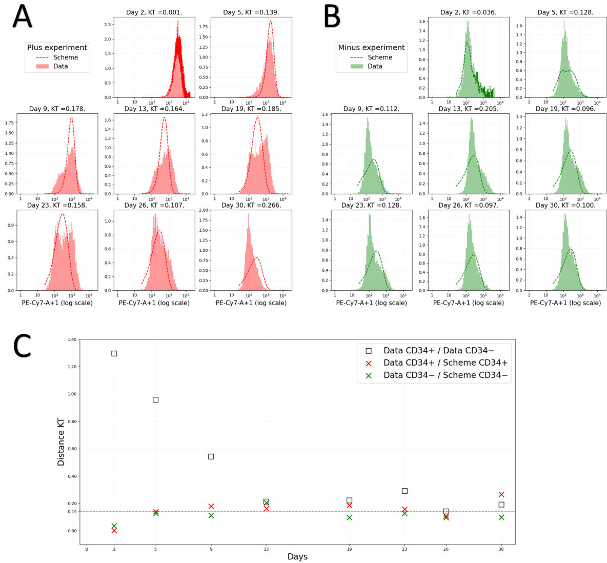
FIGURE 5.6 – Comparison of model and data. On the left the fitting of the CD34^+ relaxation experiment (in A) and on the right in green of the CD34^- (in B) experiments. Experimental data in logarithmic scale are represented by plain histograms and the numerical results of model (5.5) are represented by the dotted curves. We initialize the model on day 2, using the biological data. The initial condition is given by (5.24). Parameter values are given in table 5.1. KT : the modified Kantorovich-Rubinstein distance, defined by the equation (5.14). C. Time-dependent evolution of the Kantorovich-Rubinstein distance between model and experimental data. For different days of the experiment, the modified Kantorovich-Rubinstein distance between the two relaxation experiments is depicted using black squares. The minimum distance, reached on day 26, is illustrated by a horizontal dotted line. The red crosses correspond to the modified Kantorovich-Rubinstein distance between the model for the parameter values from Table 5.1, and the CD34^+ cell relaxation experiment. Similarly, the green crosses represent the distance for the CD34^- cell relaxation experiment.
