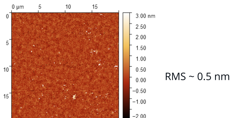
Figure 2.45: AFM image of 0.5/5 nm Cr/Au acquired OptMatLab at University of Genova. Field is 20 \times 20 \mu\text{m} with 3 nm height colorbar. Resulting RMS was measured to be 0.5 nm.
