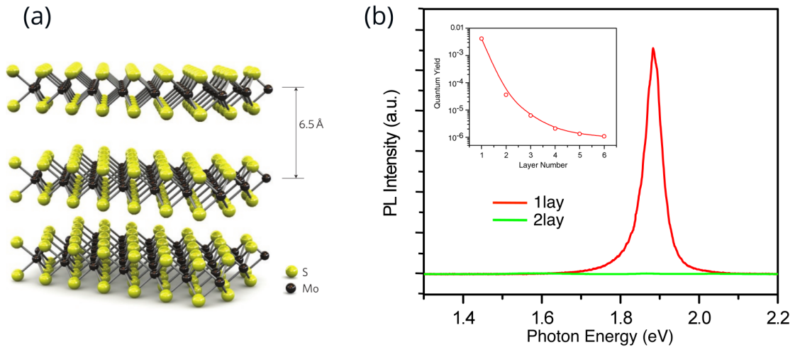
Figure 1.1: (a) Diagram of MoS 2 crystal structure, from [15]. (b) Photoluminescence intensity of MoS 2 for monolayer, bilayer, trilayer, 4, 5, 6 layer, reproduced from [16].
