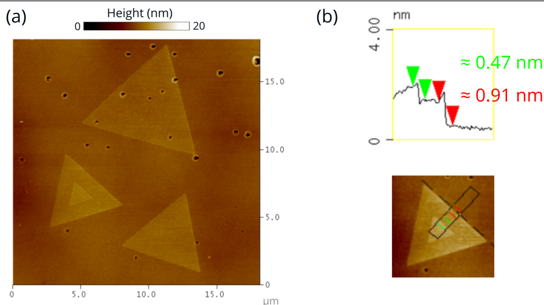
Figure 1.12: (a) AFM image acquired at LICSEN of monolayer (and bilayer) MoS 2 grown by CVD. This sample is rather smooth and defect-free, with one flake containing a 3R stacked bilayer. (b) Averaged line profile of the mono/bi-layer flake, giving an approximate value of height as shown. This is relatively consistent with the textbook value of 0.65 nm. Different factors can influence the measured height such as the presence of adsorbates above or below the mono/bi-layer.
