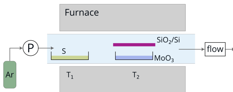
Figure 1.11: Chemical vapor deposition (CVD) setup used at LICSEN to grow 2D MoS 2 and other 2D TMDs. A chemical reaction between the sublimated sulfur and MoO 3 result in 2D MoS 2 on the substrate. Many tunable parameters as shown in the furnace impact the result making it very challenging to consistently grow 2D MoS 2 . Some include carrier gas, pressure, flow rate, temperatures T 1 and T 2 , sulfur and MoO 3 quantities, and many more.
