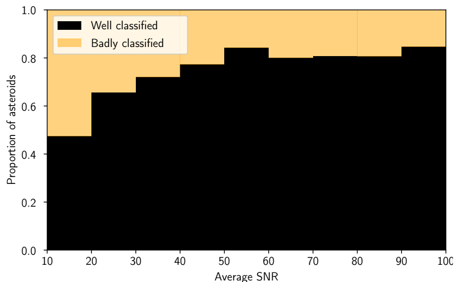
Figure B.9: Proportion of well and badly classified asteroids with my classification algorithm for ranges of SNR going from 10 to a hundred by steps of 10.
