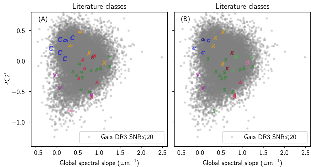
Figure B.9: Plot of the principal component \text{PC2}' with respect to the global slope, calculated for the 22 066 filtered Gaia DR3 asteroids with \text{SNR} \leq 20 . The 33 asteroids highlighted are the objects classified from NIR observations. Each coloured letter represents the assigned spectral type from the literature in panel (A), and the first best spectral type assigned with the Gaia classification in panel (B).
