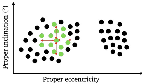
Figure 1.7: Simplified illustration of the steps of the HCM applied to the proper orbital elements space of asteroids. The proper inclination versus eccentricity space is taken as an example for clarity, the HCM being applied to the 3D space including the proper semi-major axis.
