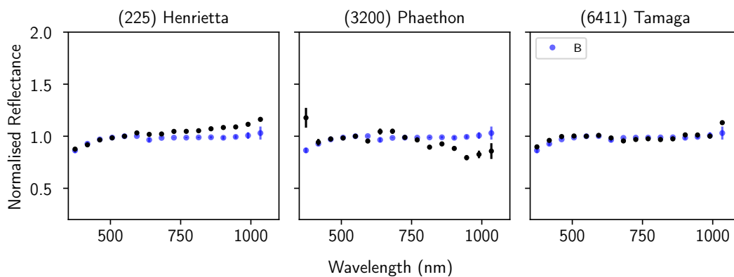
Figure B.9: Gaia DR3 spectra of the three B-type asteroids contained in the NIR list (black dots). The Gaia B-type template is displayed as blue dots, for reference.
