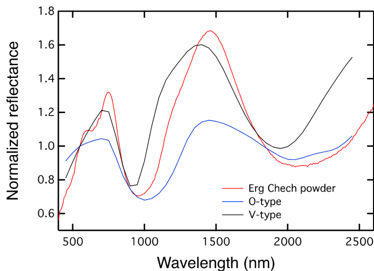
Figure 3.2: Figure from the supplementary material of Barrat et al. (2021), showing the reflectance spectrum of a powder sample of EC 002 compared to the spectra of the V and O-types of DeMeo et al. (2009).
