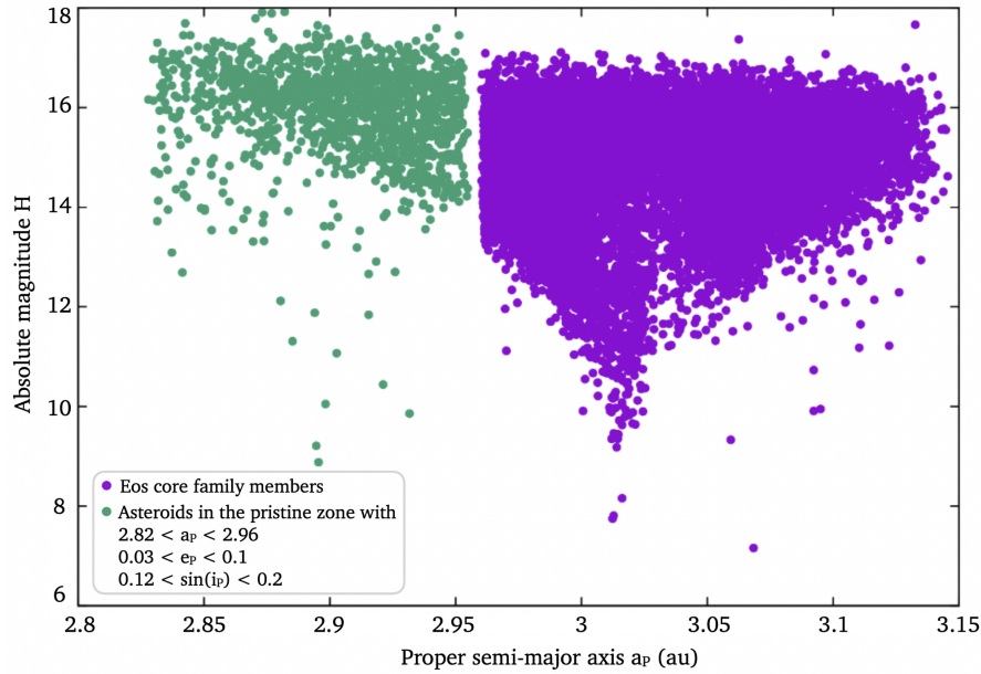
Figure 4.5: Figure 3 from Tsirvoulis et al. (2018): (221) Eos family V-shape and identified population of Eos fugitives in the pristine zone. The Eos family core as identified by Milani et al. (2014) is displayed in purple dots, and the asteroids in the pristine zone in the region delimited by 2.82 < a_p < 2.96 , 0.03 < e_p < 0.1 and 0.12 < \sin(i_p) < 0.2 in green dots.
