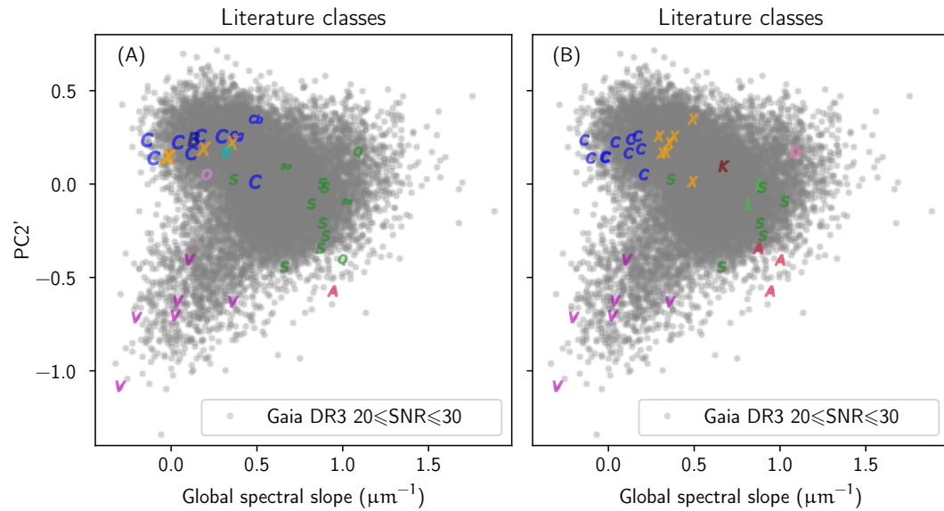
Figure B.9: Plot of the principal component \text{PC2}' with respect to the global slope, calculated for the 14 132 filtered Gaia DR3 asteroids with 20 \leq \text{SNR} \leq 30 . The 36 asteroids highlighted are the objects classified from NIR observations. Each coloured letter represents the assigned spectral type from the literature in panel (A), and the first best spectral type assigned with the Gaia classification in panel (B).
