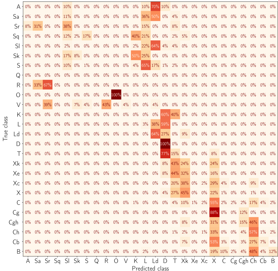
Figure 5.2: Confusion matrix corresponding to the classification of Gaia DR3 spectra, using Bus and Binzel (2002a) templates.
