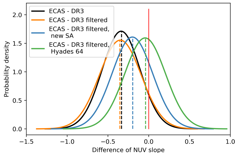
Figure 2.19: Gaussian fit of the histogram of the calculated NUV slope on the 154 asteroids having spectra in the filtered DR 3 and in Tinaut-Ruano et al. (2023). In black is displayed the Gaussian fit of the histogram of the NUV slope difference between the one calculated on spectra from the ECAS database and the one calculated on Gaia DR 3 mean reflectance spectra, in orange the red slope difference calculated between the red slope of ECAS spectra and the one calculated on filtered Gaia spectra, and in blue the same difference calculated on filtered Gaia DR 3 spectra produced with the new mean solar analogue. In green is displayed the Gaussian fit of the histogram of the NUV slope difference between ECAS and the Gaia mean reflectance spectra calculated using Hyades 64 as solar analogue. A line at 0 nm is highlighted in red.
