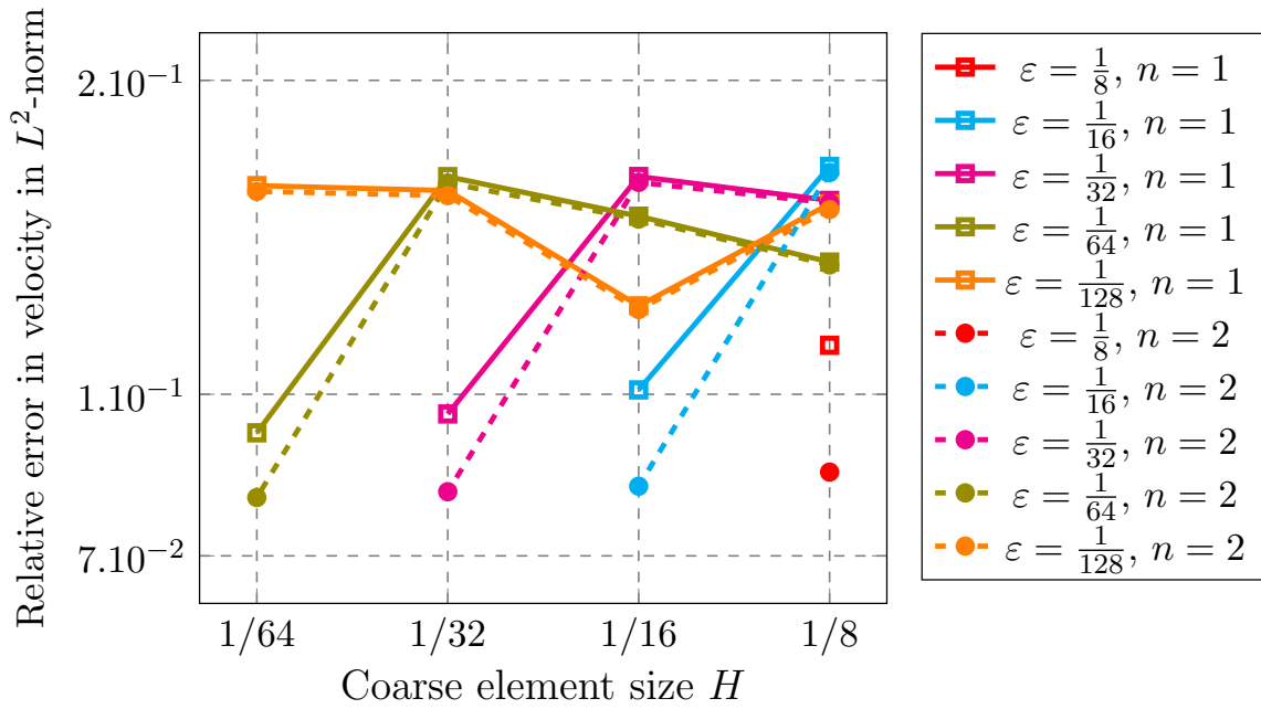
Figure 14.2: Relative errors between MsFEM approximations and reference solutions for velocity in L^2 -norm (Stokes flow).
