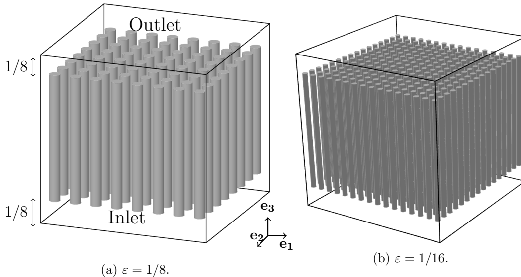
Figure 13.4: Scheme of the computational domain \Omega^\varepsilon in three dimensions.
