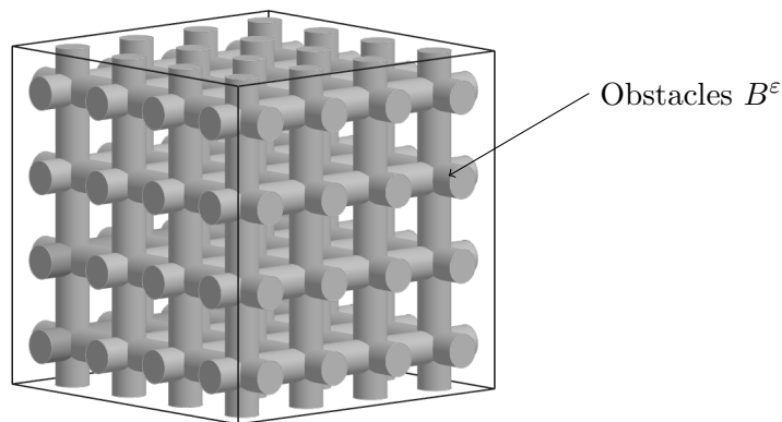
Figure 1.3: Three-dimensional porous domain \Omega^\varepsilon , obtained from a domain \Omega perforated by a set of solid obstacles B^\varepsilon .
