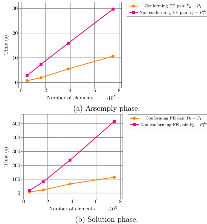
Figure 5.13: Comparison of the computational times of the non-conforming FE pair V_2 - \mathbb{P}_1^{\text{dc}} and the conforming FE pair \mathbb{P}_2 - \mathbb{P}_1 for different mesh sizes computed on 64 processes.
