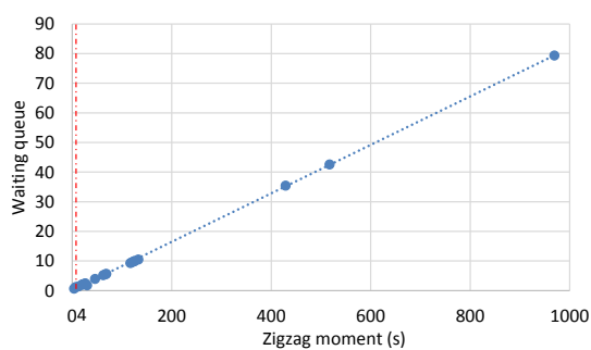
(b) The length of waiting queue at LX 69 in G1
