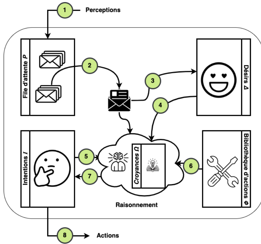
FIGURE 1.11 – Architecture BDI
