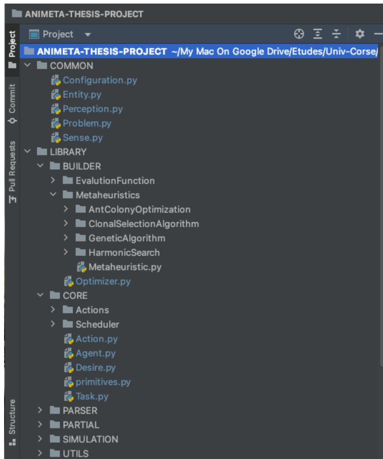
FIGURE 5.2 – Arborescence du ANIMETA-ENGINE
