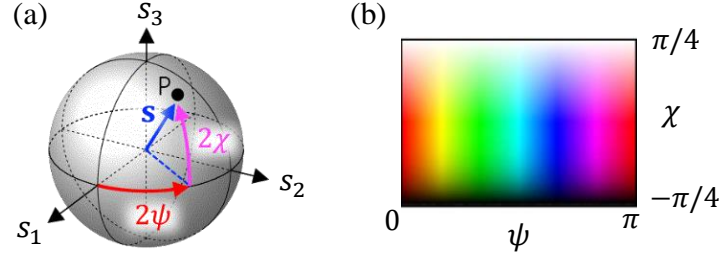
Figure 3.1 (a) Representation of the Poincaré sphere, where any point P is described by Stokes vector \mathbf{s} , polarization ellipse azimuth \psi , and ellipticity \chi . (b) Colormap used for Stokes vector and texture coloring, where each point on the Poincaré sphere is represented by a hue indicating the \psi angle, and brightness referring to the ellipticity \chi .
