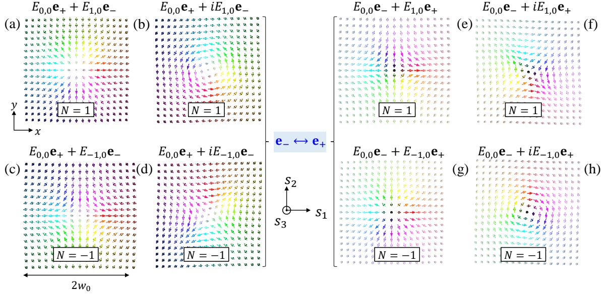
Figure 3.2 Representative set of Stokes vector fields in the plane (x, y) that correspond to fundamental skyrmions with N = \pm 1 , where w_0 = w(0) . The Stokes vector fields are colored according to the bijective relationship illustrated in Fig. 3.1, which associates every point on the Poincaré sphere to a given point of a colormap.
