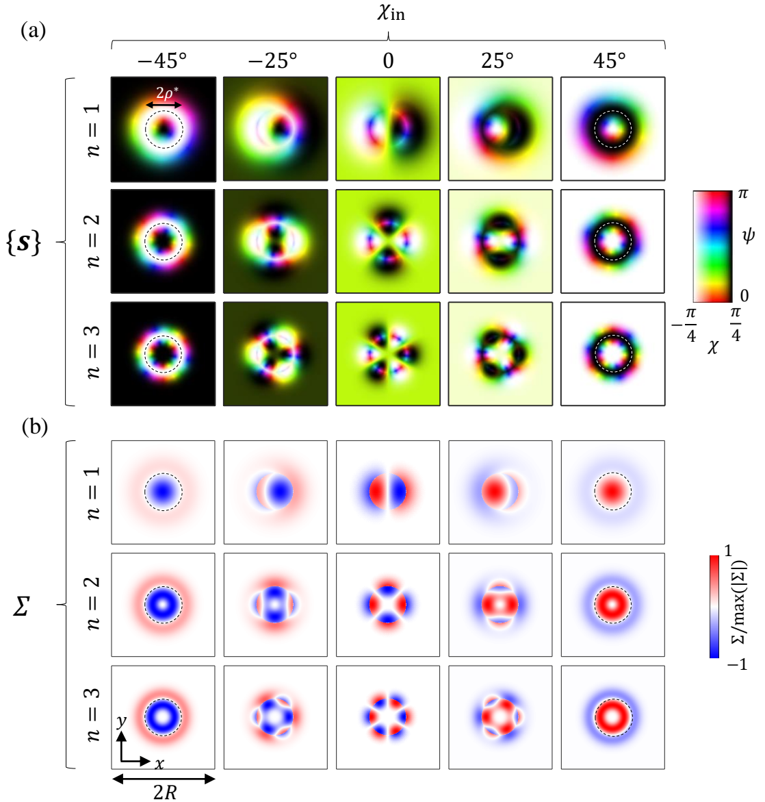
Figure 3.8 Simulation results of (a) Stokes textures \{s\} and (b) Skyrme density \Sigma corresponding to the counterpart of Figs. 3.7(b) and 3.7(c).
