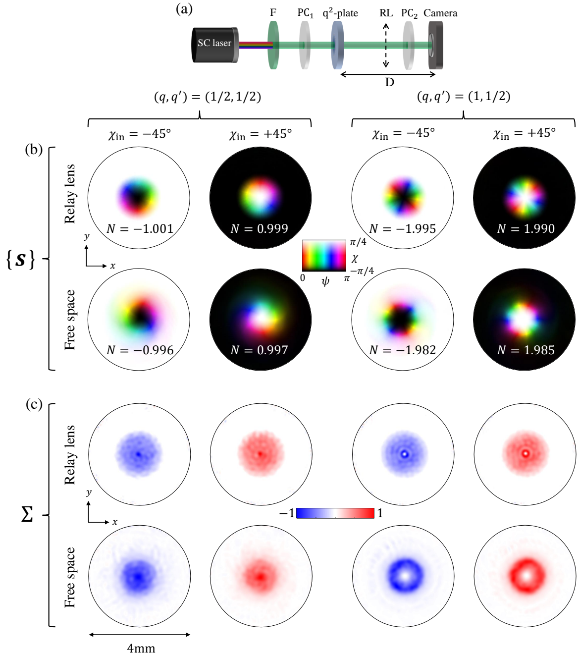
Figure 3.21 (a) Experimental setup for the observation of the generated skyrmion beam. It was used a supercontinuum laser with 1.5 mm beam waist radius and filtered by 532 nm spectral filter (F). PC 1 : polarization controller made of a linear polarizer, quarter-waveplate, and half-waveplate to achieve any arbitrary incident polarization state. RL: relay lens with 30 cm focal length placed at mid-distance between the q 2 -plate and the camera. PC 2 : polarization controller allowing to project the intensity distribution of the output field on H, V, D, A, L, R polarization states and to record the corresponding intensity profiles with a camera placed at a distance D = 1.2 m from the q 2 -plate. (b) Experimental Stokes textures \{s\} and (c) Skyrme density of q 2 -plates with (q, q') = (1/2, 1/2) and (q, q') = (1, 1/2) that correspond to skyrmions with Skyrme number ideally equal to N = 2\sigma q , respectively and in the case of with (top) and without (bottom) the presence of the relay lens.
