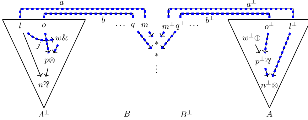
Figure 6.8: Switching cycle containing w if p is a \otimes -vertex in the proof of Lemma 6.59
