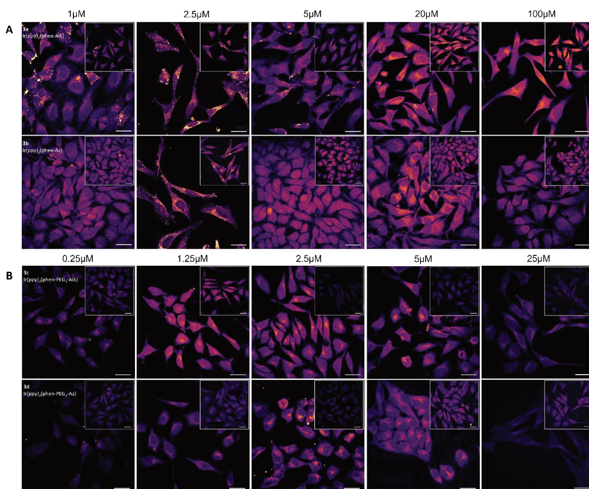
Figure S1 : Probe concentration optimization for cell labeling via CuAAC. (A) Optimization of the non-PEG complexes 3a and 3b with concentrations ranging from 1 to 100 \mu\text{M} after 48h incorporation of ManNAz or ManNAc (control, corner inserts). (B) Optimization of the PEG-spacer bearing complexes 3c and 3d with concentrations ranging from 0.25 to 25 \mu\text{M} after 48h incorporation of ManNAz or ManNAc (control, corner inserts). (exc 405nm, em 570-620nm). Scale bar = 30 \mu\text{m} .
