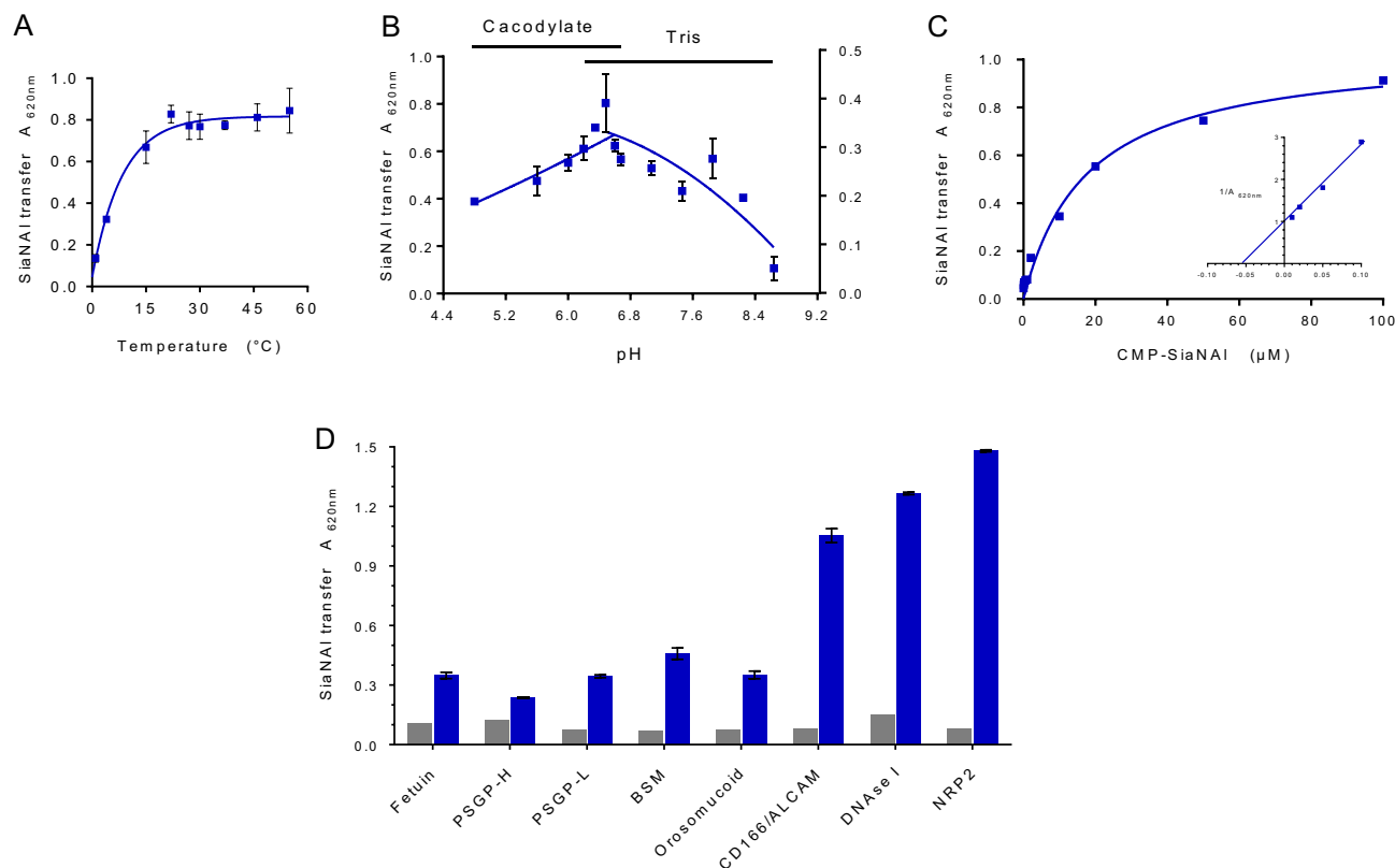
Figure 3. Optimization of sialylation conditions in the MPSA. (A) Effect of temperature on the sialylation by CmaST8Sia IV . Sialylation was performed 4 h on 400 ng of CD166/ALCAM with 100 \mu M CMP-SiaNAI and 20 \mu L of CmaST8Sia IV at different temperatures from 0 ^{\circ} C to 60 ^{\circ} C ( n=2 ). (B) Effect of pH on the sialylation by CmaST8Sia IV . Sialylation reactions were performed 4 h at 27 ^{\circ} C on 400 ng of CD166/ALCAM with 100 \mu M CMP-SiaNAI and 20 \mu L of CmaST8Sia IV at different pH from 4.8 to 8.6 ( n=2 ). (C) Determination of kinetic parameters of ST8Sia IV towards donor substrates. Sialylation reactions were carried out in cacodylate buffer pH 6.4, at 27 ^{\circ} C for 4 h with 20 \mu L of fish ST8Sia IV. CMP-SiaNAI was used at various concentrations ranging from 0 to 100 \mu M with 400 ng of CD166/ALCAM ( n=3 ). Michaelis–Menten constants were determined graphically with GraphPad. CmaST8Sia IV shows an apparent K_m of 17.60 \pm 2.52 \mu M towards donor substrate. (D) Enzymatic activities on several acceptors in the MPSA. Sialylation reactions were performed 4 h at 27 ^{\circ} C using 400 ng of various acceptors (fetuin, PSGP-H, PSGP-L, BSM, orosomucoid, CD166/ALCAM, DNase I and NRP2) with 100 \mu M of CMP-SiaNAI and with 20 \mu L of CmaST8Sia IV (blue) or Mock (grey). Error bars represent SEM ( n=2 ).
