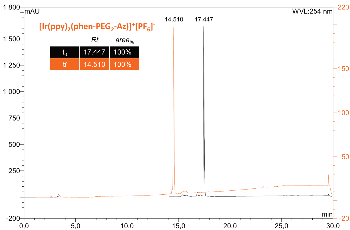
Figure S8 – UV HPLC chromatograms of complexes 3a-d before and after CuAAC ligation with ManNAz.
